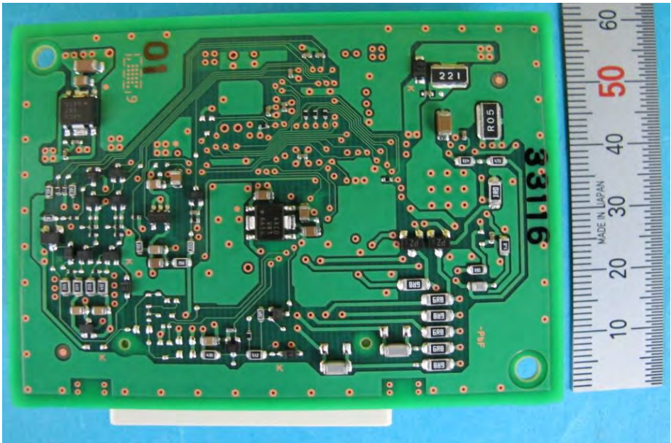
BACK
