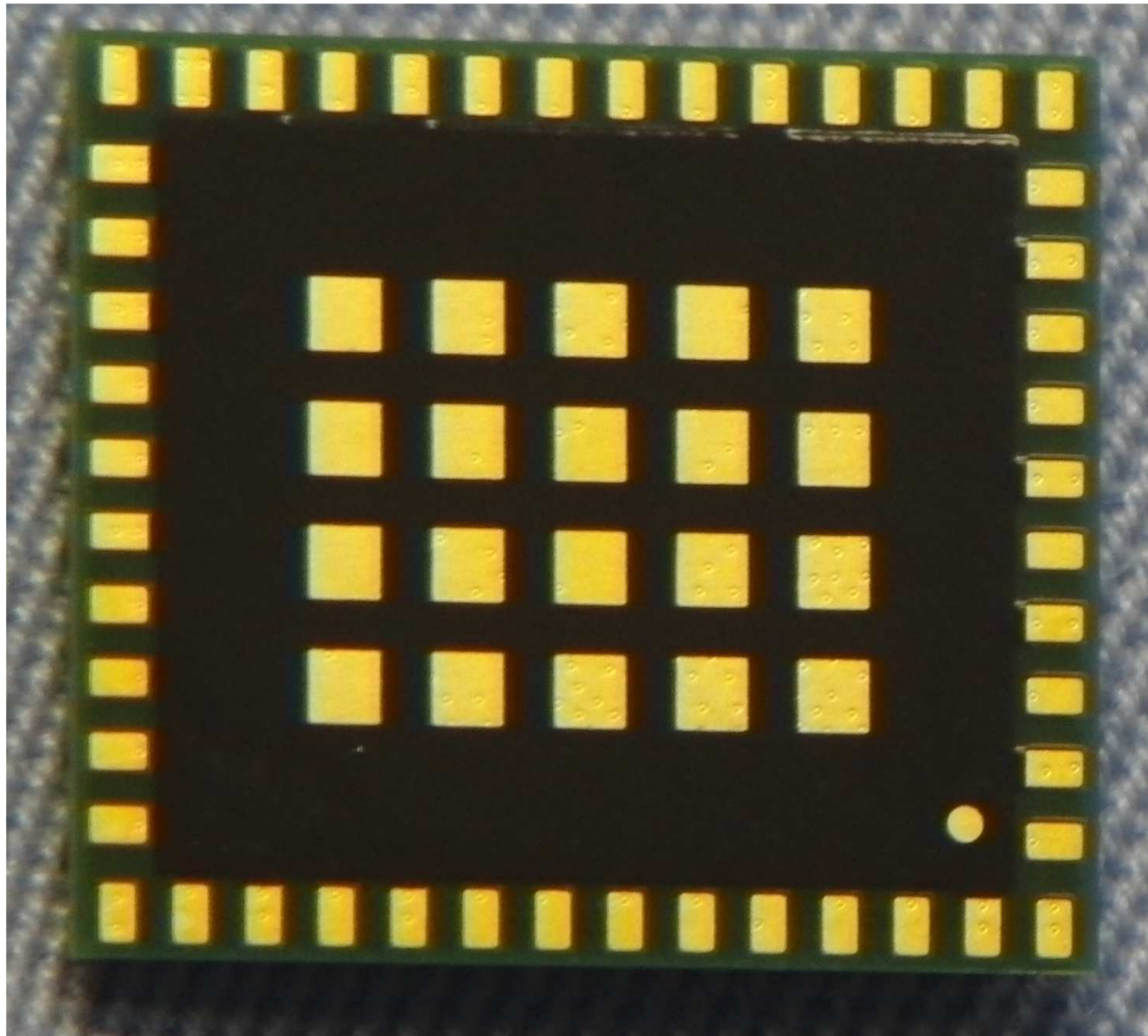
3.Bottom View
