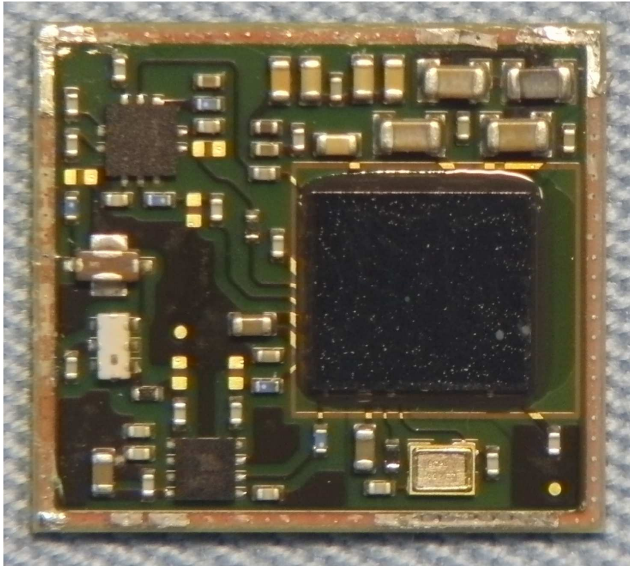
2.Top View(Shield is removed)
