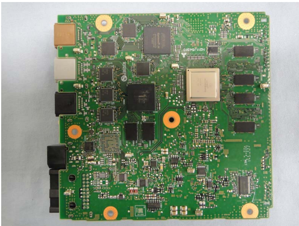
Board Bottom
