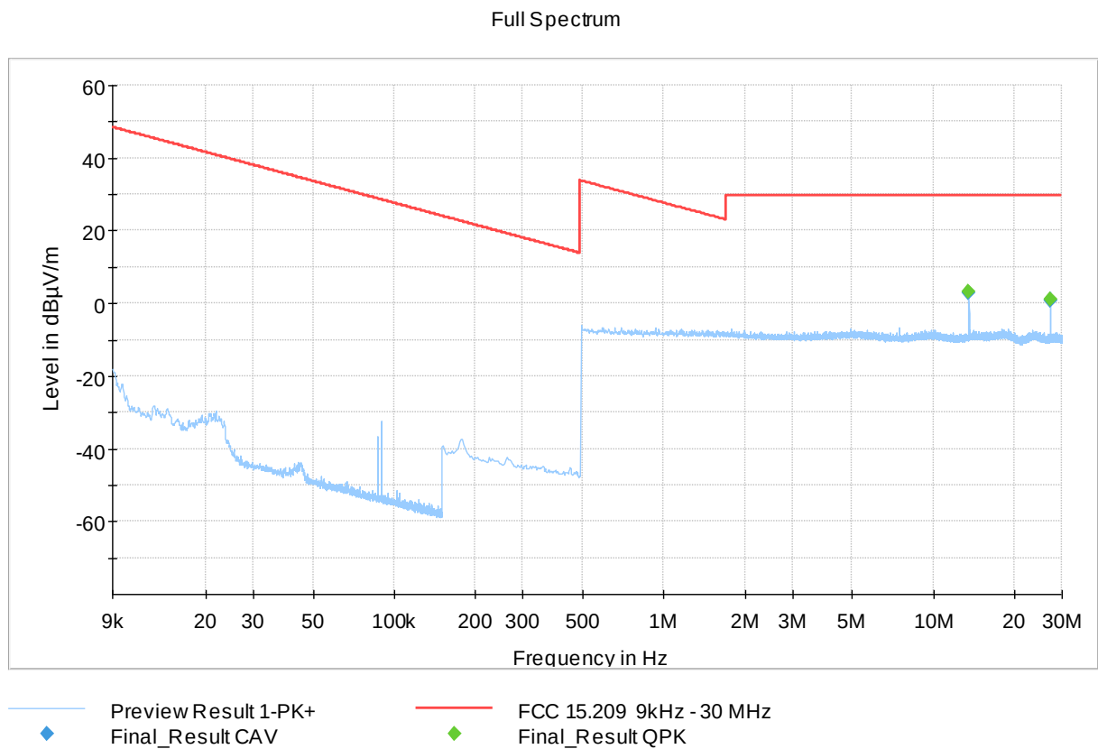
Figure 5. TX radiated emission 9 kHz to 30MHz, Cylinder antenna with TAG
