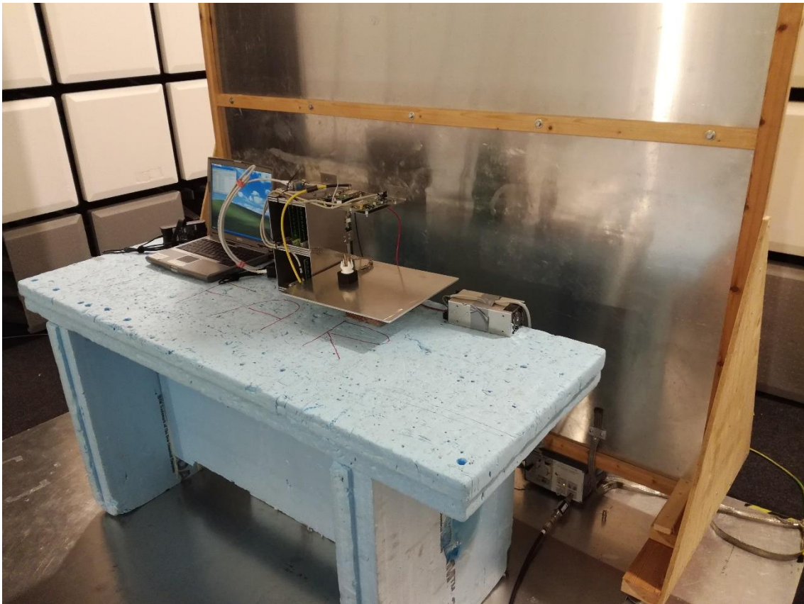
Photograph 5. Conducted Emissions 150 kHz – 30 MHz
