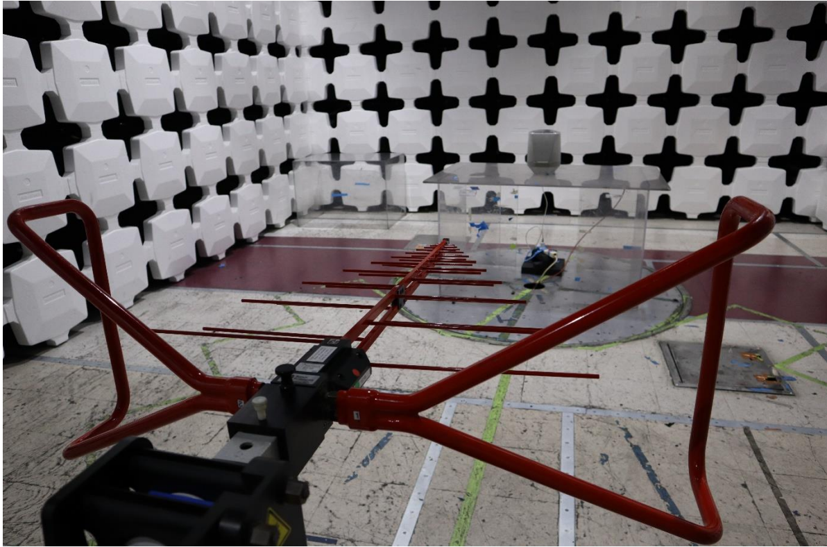
Figure 1. Radiated Spurious Emissions, (30 MHz – 1 GHz) Test Setup
