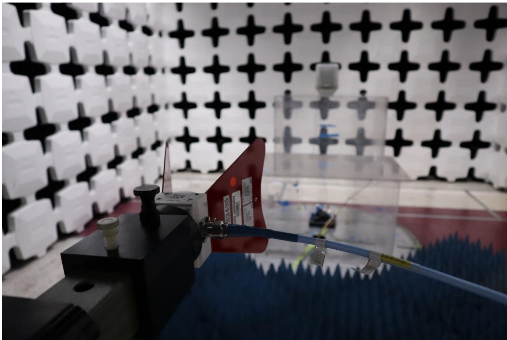
Figure 4. Radiated Spurious Emissions, (1 - 18 GHz) Test Setup
