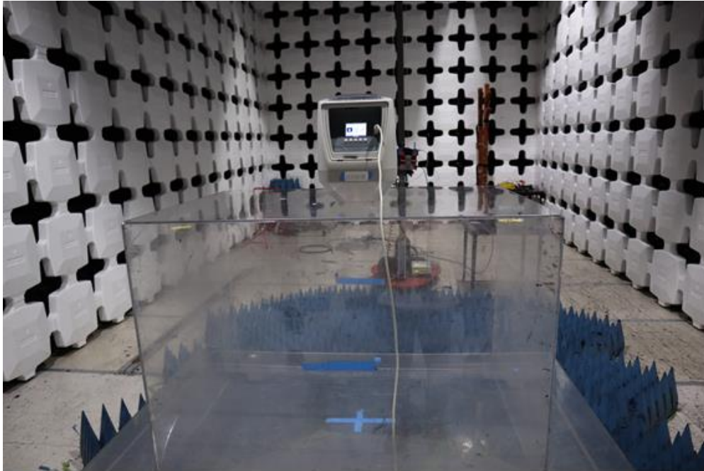
Figure 3. Radiated Spurious Emissions, (1 - 18 GHz) Test Setup
