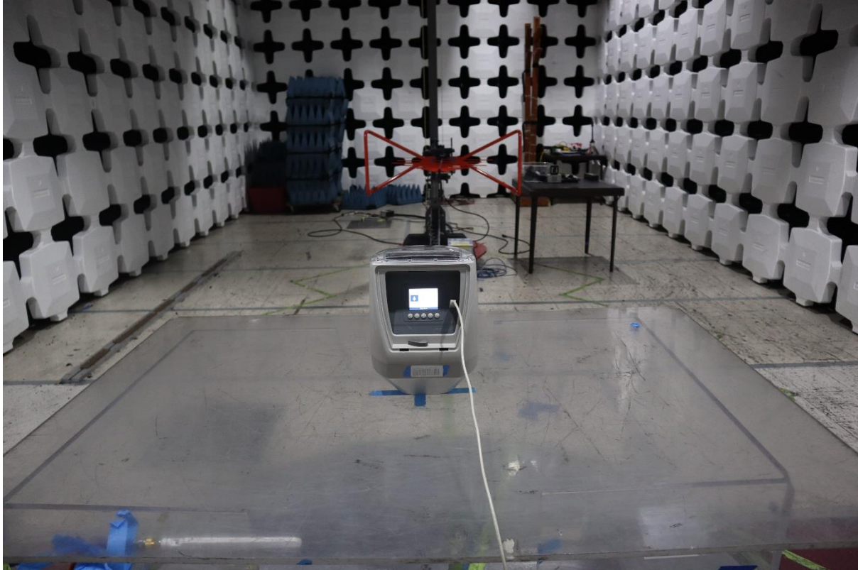
Figure 2. Radiated Spurious Emissions, (30 MHz – 1 GHz) Test Setup
