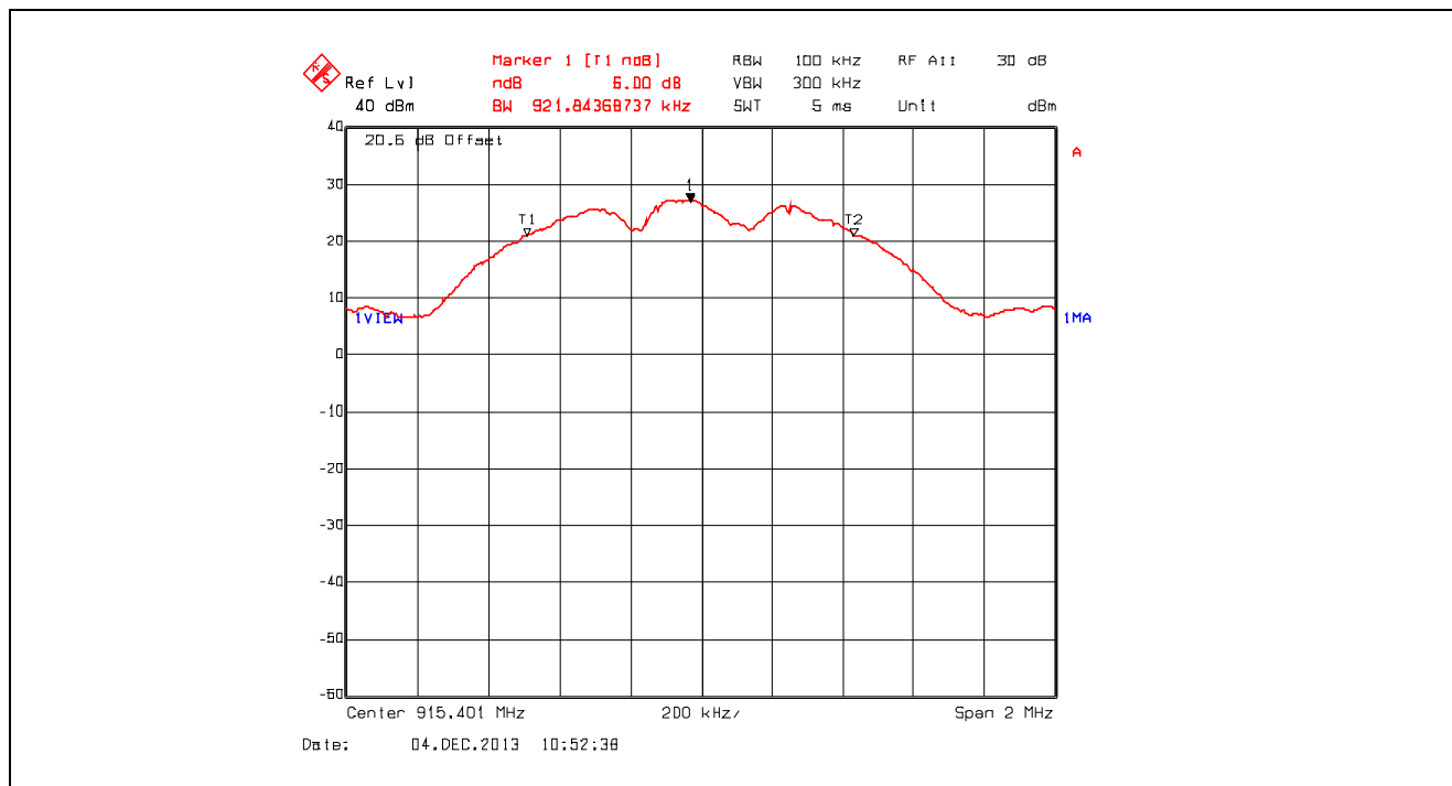
Plot 5.2.4.2. 6 dB Bandwidth, 915.401 MHz
