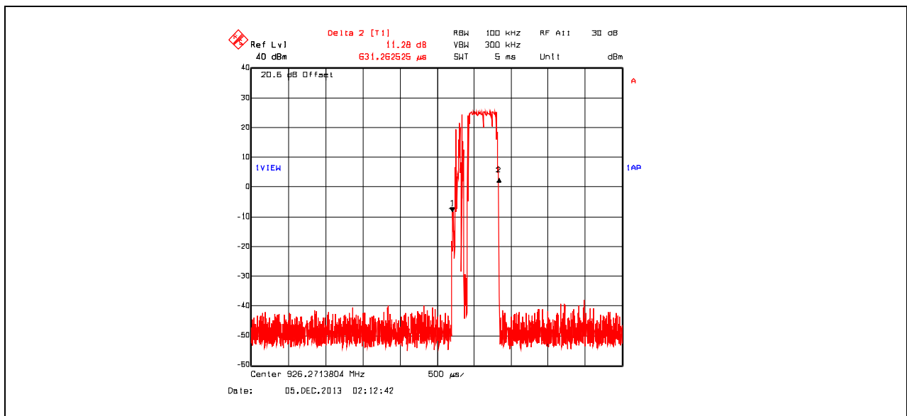
Plot 5.5.4.2. Duty Cycle (pulse duration is 631.262525 \mu s = 0.631263 ms)
