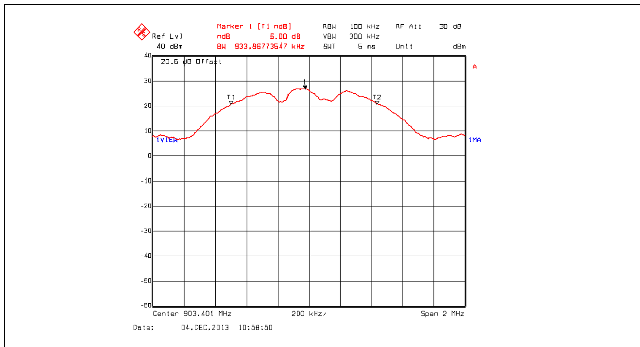
Plot 5.2.4.1. 6 dB Bandwidth, 903.401 MHz
