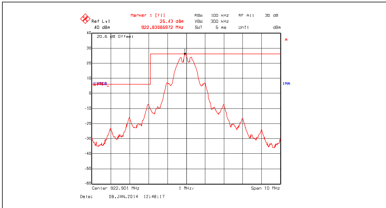
Plot 5.4.4.1.5. Band-Edge RF Conducted Emissions for New Zealand Band 921 – 928 MHz , 922.901 MHz
