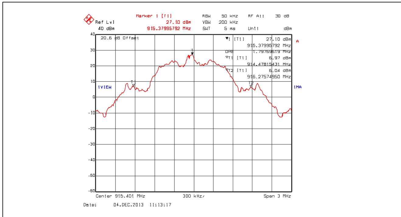
Plot 5.2.4.5. 99% Occupied Bandwidth, 915.401 MHz
