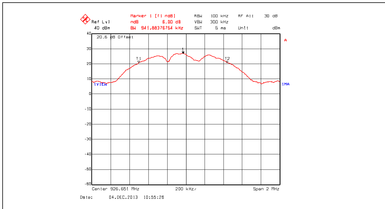
Plot 5.2.4.3. 6 dB Bandwidth, 926.651 MHz
