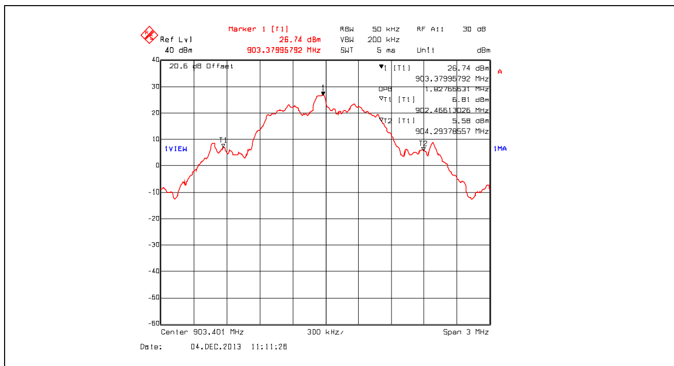
Plot 5.2.4.4. 99% Occupied Bandwidth, 903.401 MHz
