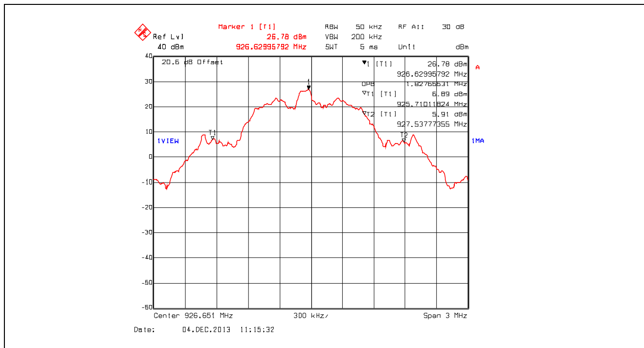
Plot 5.2.4.6. 99% Occupied Bandwidth, 926.651 MHz
