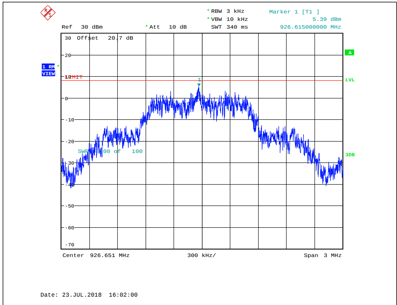
Plot 5.5.4.3. Power Spectral Density, 926.651 MHz, FSK Modulation Detector RMS, Video Trace Averaging with 100 Traces, Sweep Points 5000 \geq 2*Span/RBW
