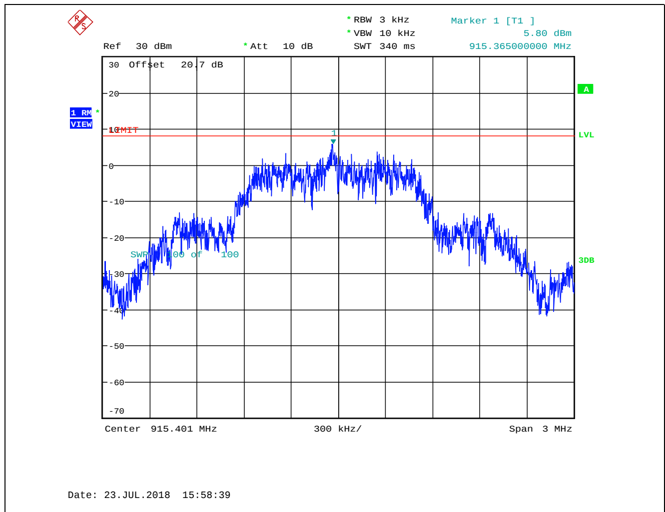
Plot 5.5.4.2. Power Spectral Density, 915.401 MHz, FSK Modulation Detector RMS, Video Trace Averaging with 100 Traces, Sweep Points 5000 \geq 2 \times \text{Span/RBW}
