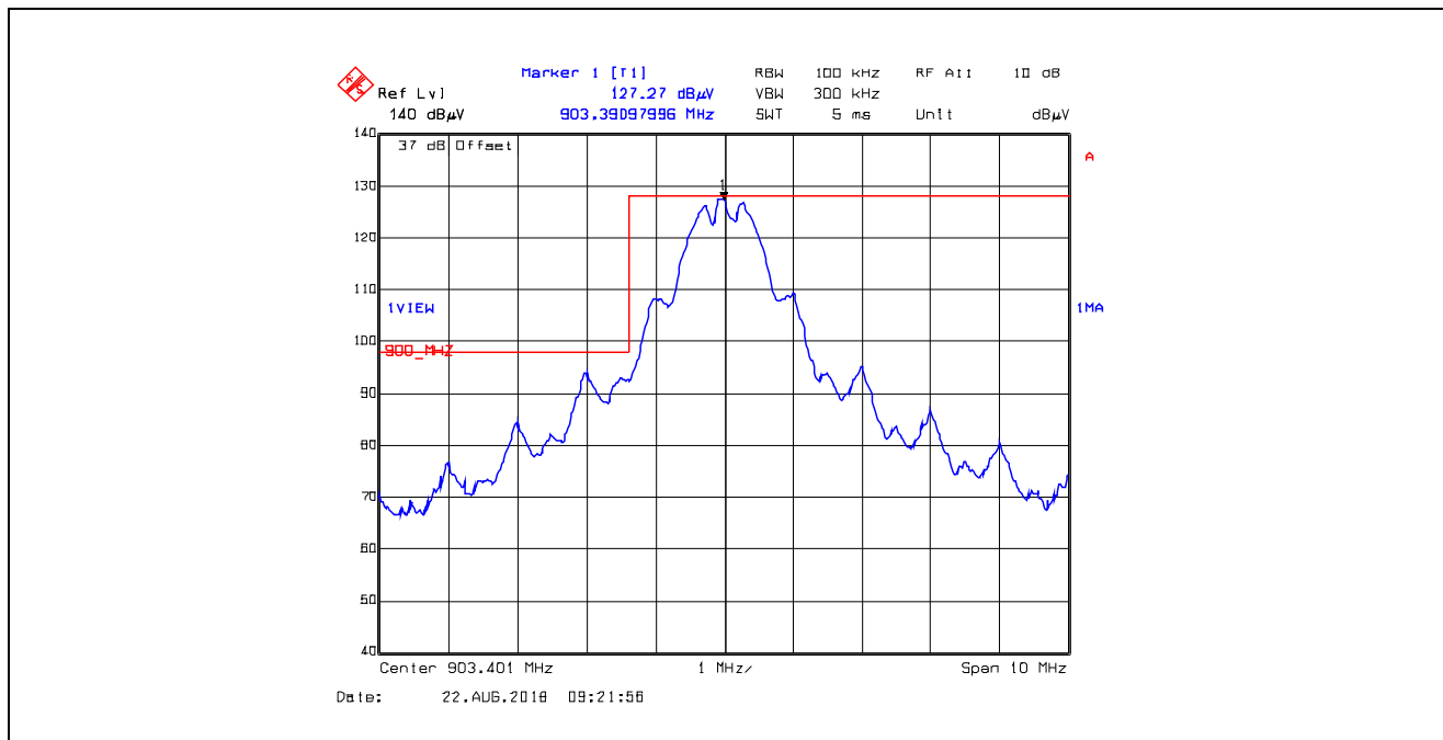
Plot 5.4.4.2.1. Band-Edge RF Radiated Emissions at 3 m, Vertical Polarization Low End of Frequency Band, 903.401 MHz FSK Modulation
