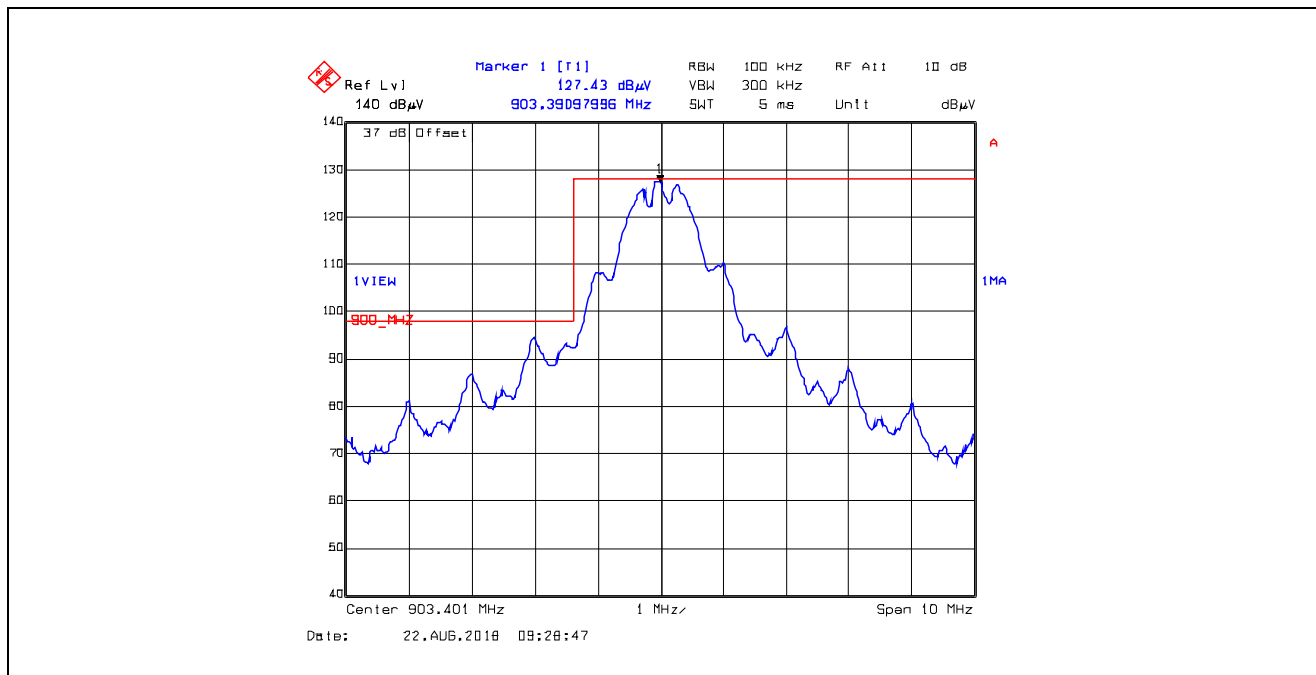
Plot 5.4.4.2.2. Band-Edge RF Radiated Emissions at 3 m, Horizontal Polarization Low End of Frequency Band, 903.401 MHz FSK Modulation
