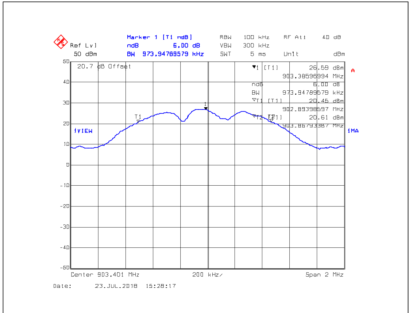
Plot 5.2.4.1. 6 dB Bandwidth, 903.401 MHz, FSK modulation
