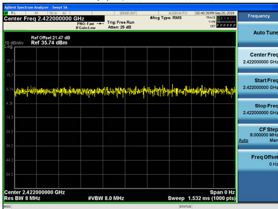
Duty cycle plot (802.11n (40M)(MCS0))
