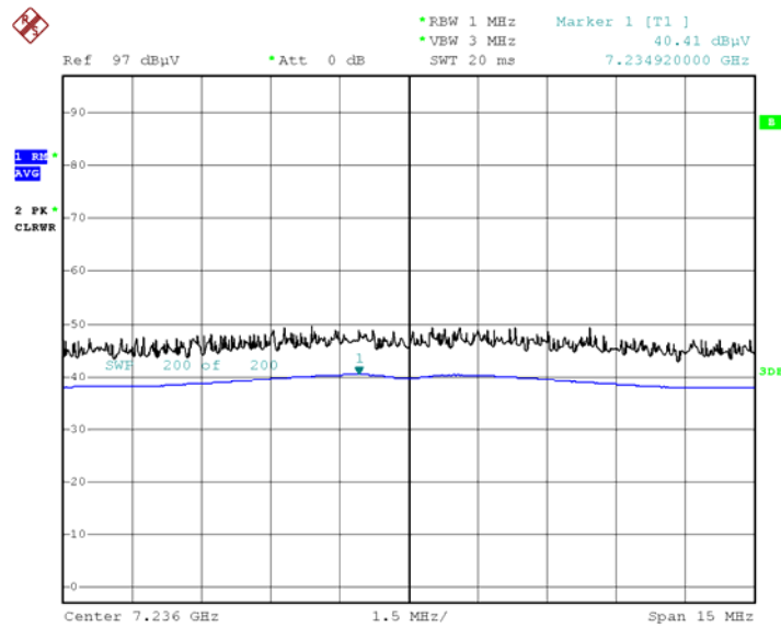
Radiated Spurious Emissions plot – Average Reading (802.11b_1Mbps, Ch.1 3rd Harmonic)
