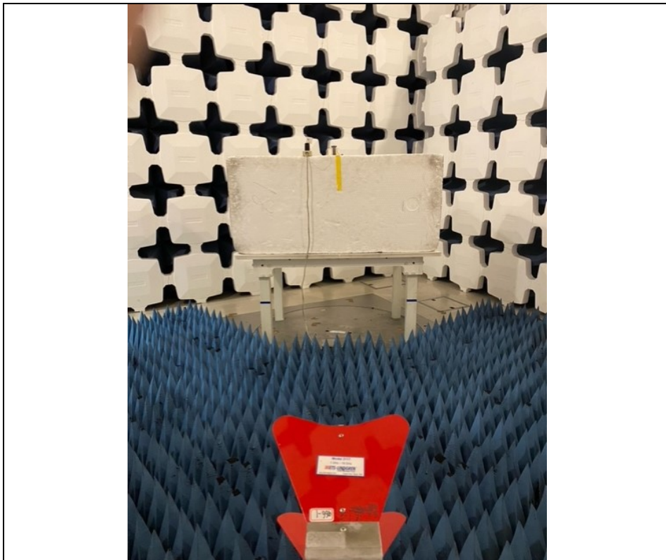
Radiated Emission above 1GHz Test
