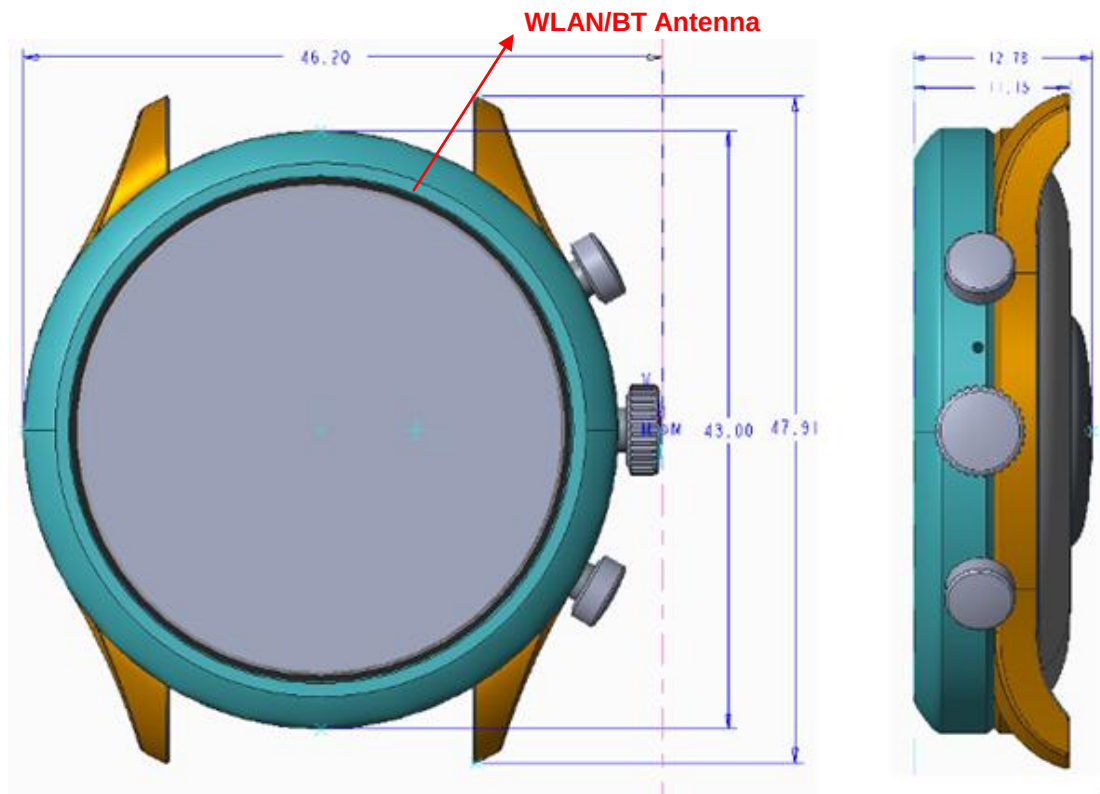
<EUT B Front View>
