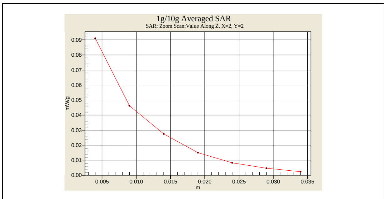
802.11b Wi-Fi body SAR of CH6(B/T on)
