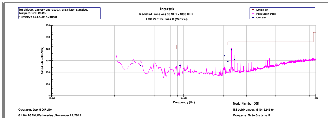
FCC part 15.209 Vertical 30-1000MHz
