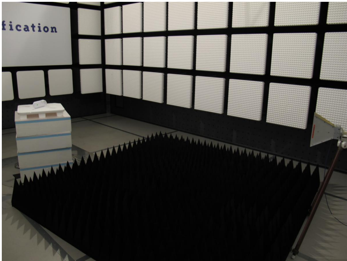
Photograph 3: Radiated emissions test set up > 1000 MHz
