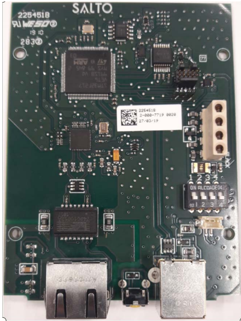
Top View
