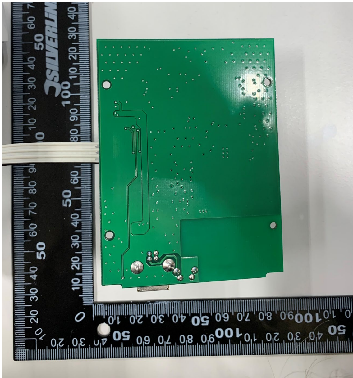
BOTTOM VIEW
