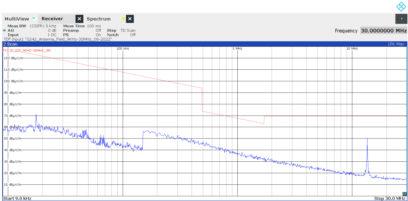
The highest peak is the RFID 13.56 MHz carrier frequency.
