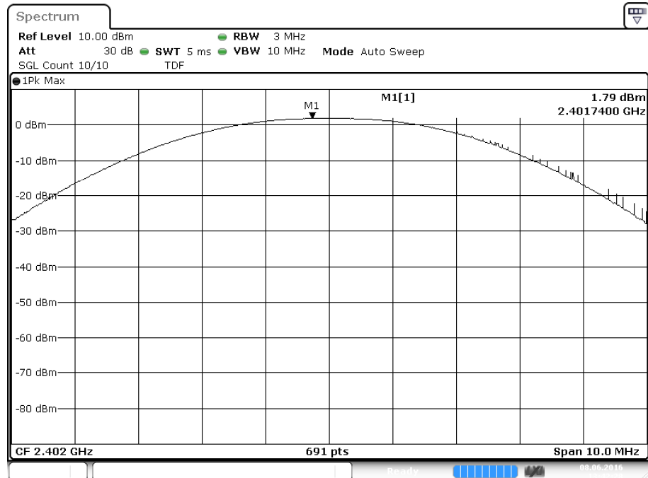
Peak Output Power (Channel 37)
