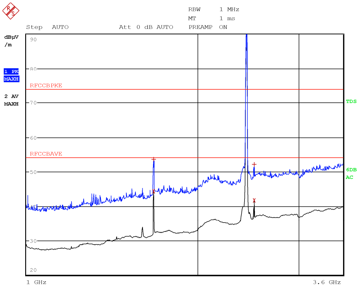
Figure 8.1-24: Radiated spurious emissions with WCDMA at 832.6 MHz and WIFI at 2437 MHz – antenna in vertical polarization
