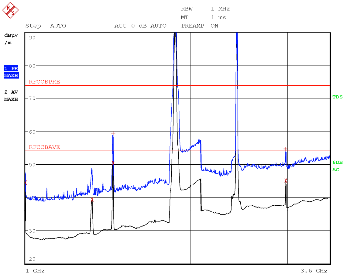
Figure 8.1-4: Radiated spurious emissions with WCDMA at 1880 MHz and WIFI at 2437 MHz – antenna in vertical polarization
