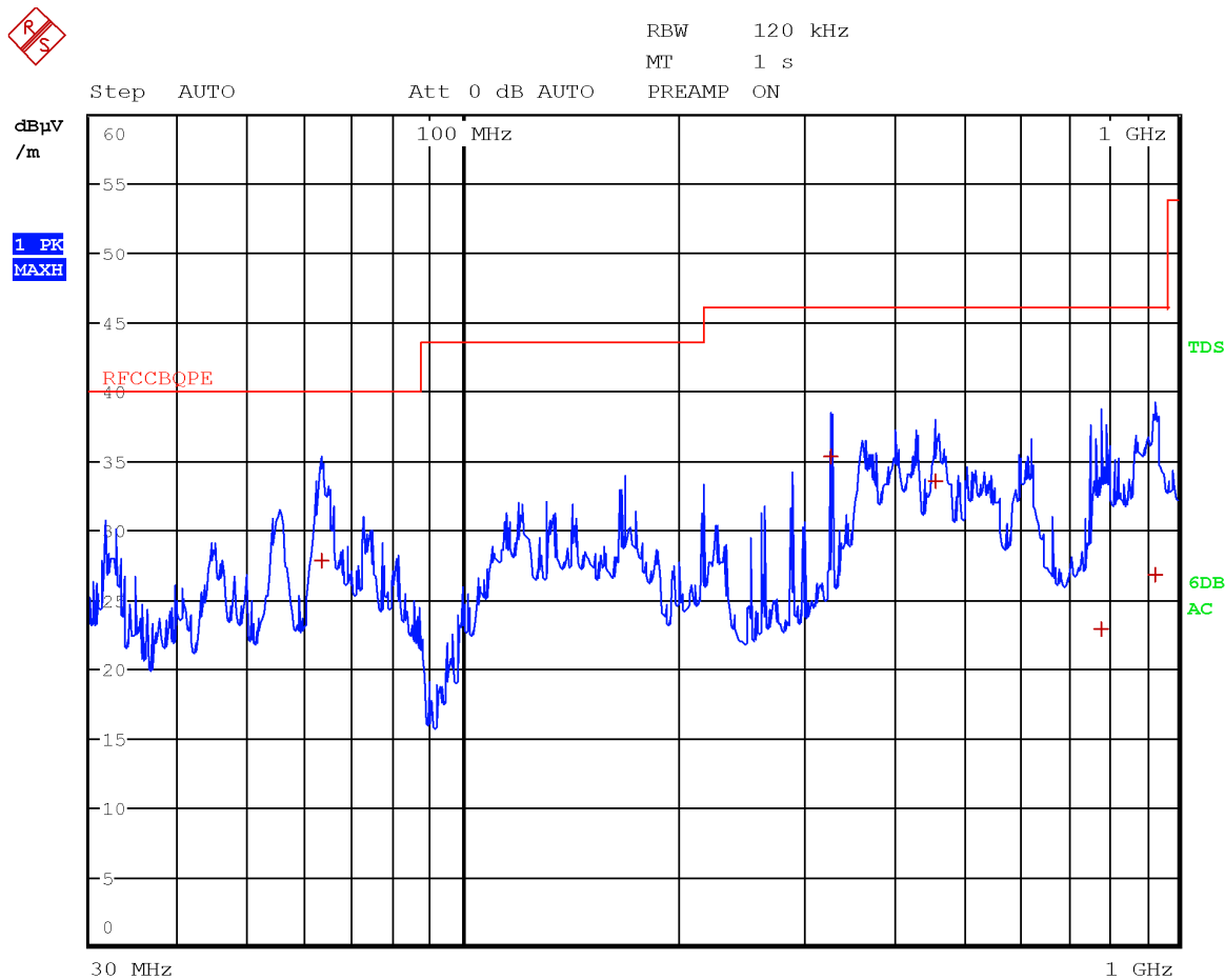
Figure 8.1-42: Radiated spurious emissions with WCDMA at 1732.6 MHz and WIFI at 5200 MHz – antenna in vertical polarization
