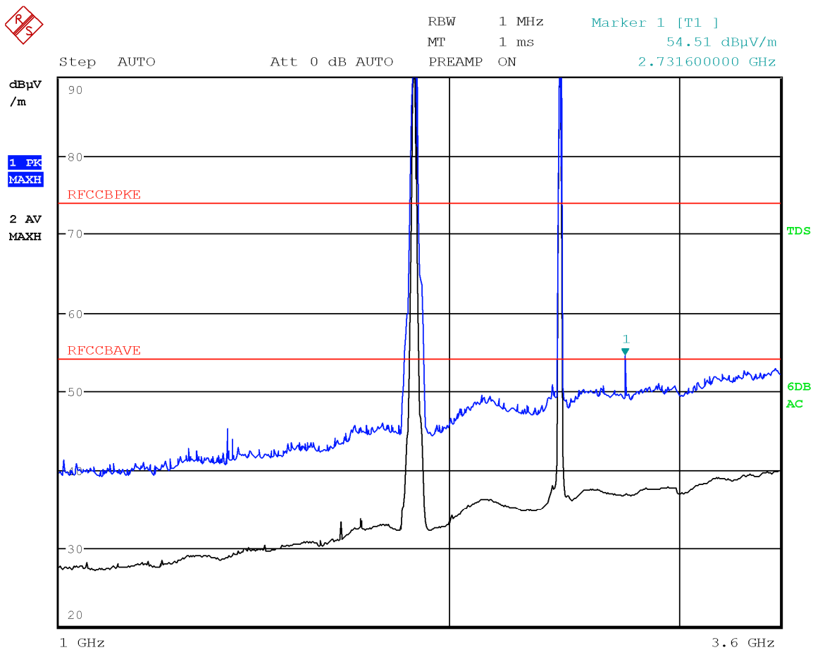
Figure 8.1-3: Radiated spurious emissions with WCDMA at 1880 MHz and WIFI at 2437 MHz – antenna in horizontal polarization
