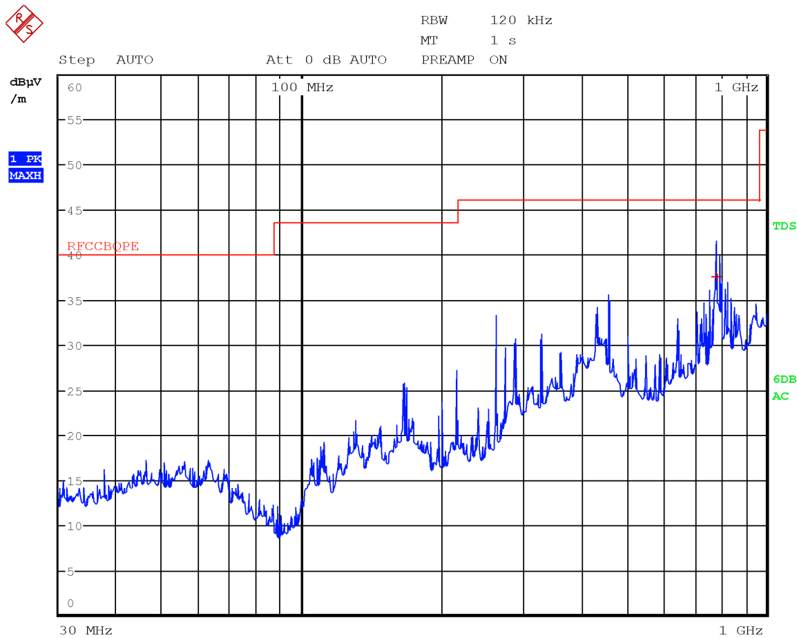
Figure 8.1-41: Radiated spurious emissions with WCDMA at 1732.6 MHz and WIFI at 5200 MHz – antenna in horizontal polarization
