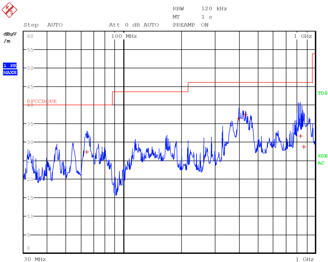
Figure 8.1-2: Radiated spurious emissions with WCDMA at 1880 MHz and WIFI at 2437 MHz – antenna in vertical polarization
