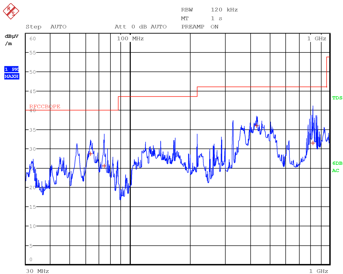
Figure 8.1-32: Radiated spurious emissions with WCDMA at 1880 MHz and WIFI at 5200 MHz – antenna in vertical polarization
