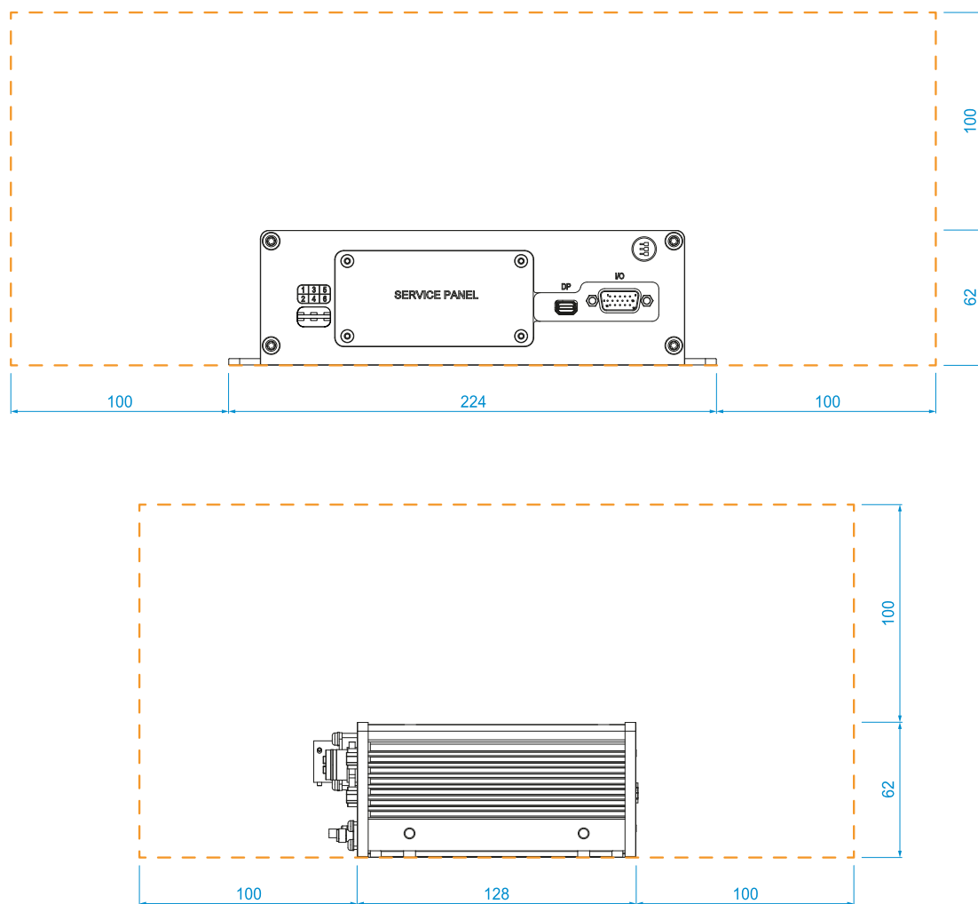
Figure 12.1 - Clearance space
