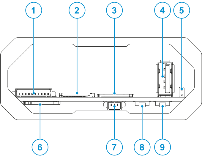
Figure 8.3 - Service Interfaces layout
