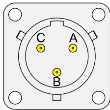
Connector Layout:
