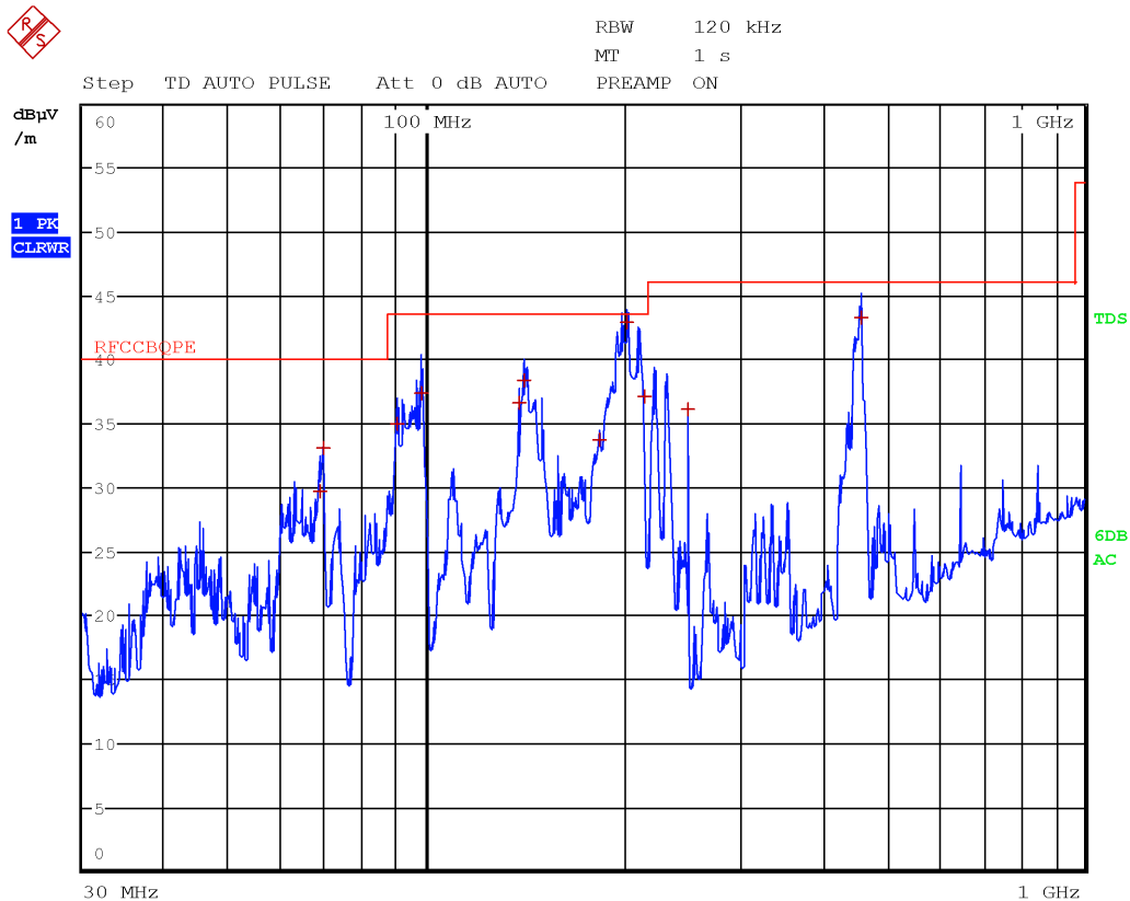
Figure 7.4-8: Radiated spurious emissions 30 to 1000 MHz, 5580 MHz with antenna in vertical polarization
