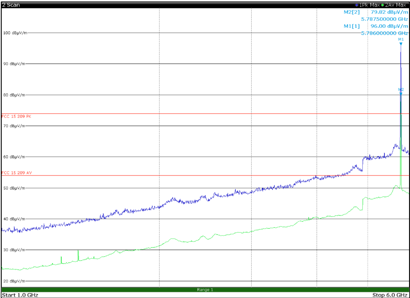
Figure 7.4-9: Radiated spurious emissions 1 to 6 GHz, 5785 MHz with antenna in horizontal polarization Limit exceeded by the carrier
