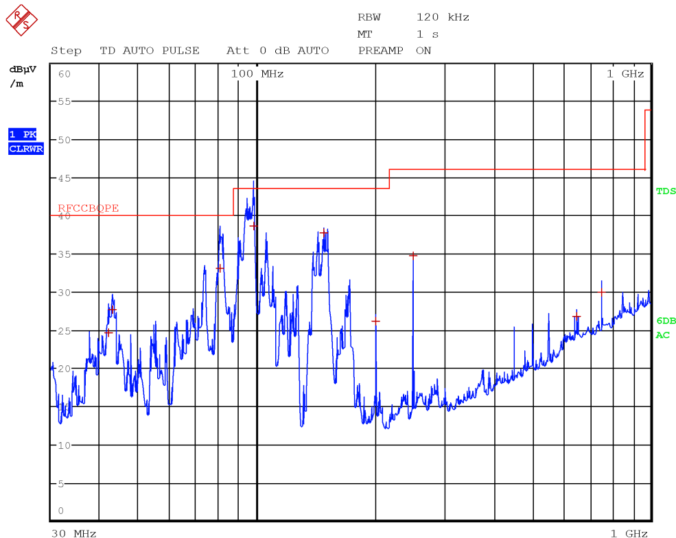
Figure 7.4-2: Radiated spurious emissions 30 to 1000 MHz, 5220 MHz with antenna in vertical polarization
