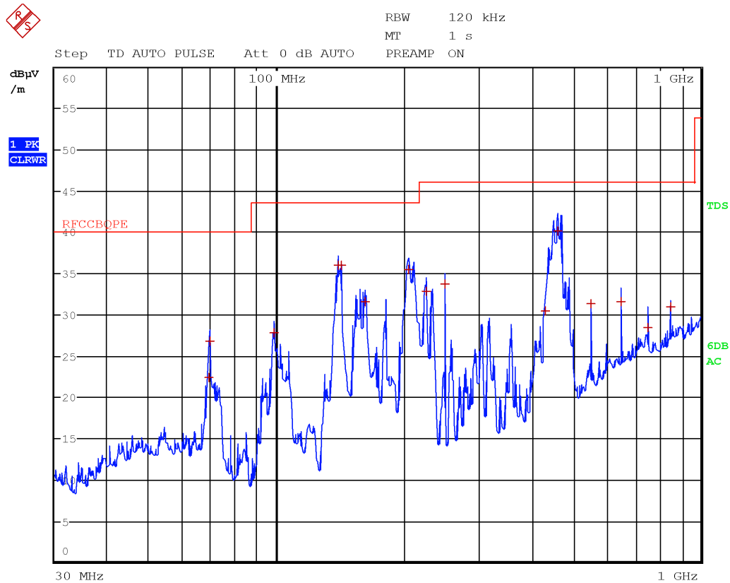
Figure 7.4-1: Radiated spurious emissions 30 to 1000 MHz, 5220 MHz with antenna in horizontal polarization
