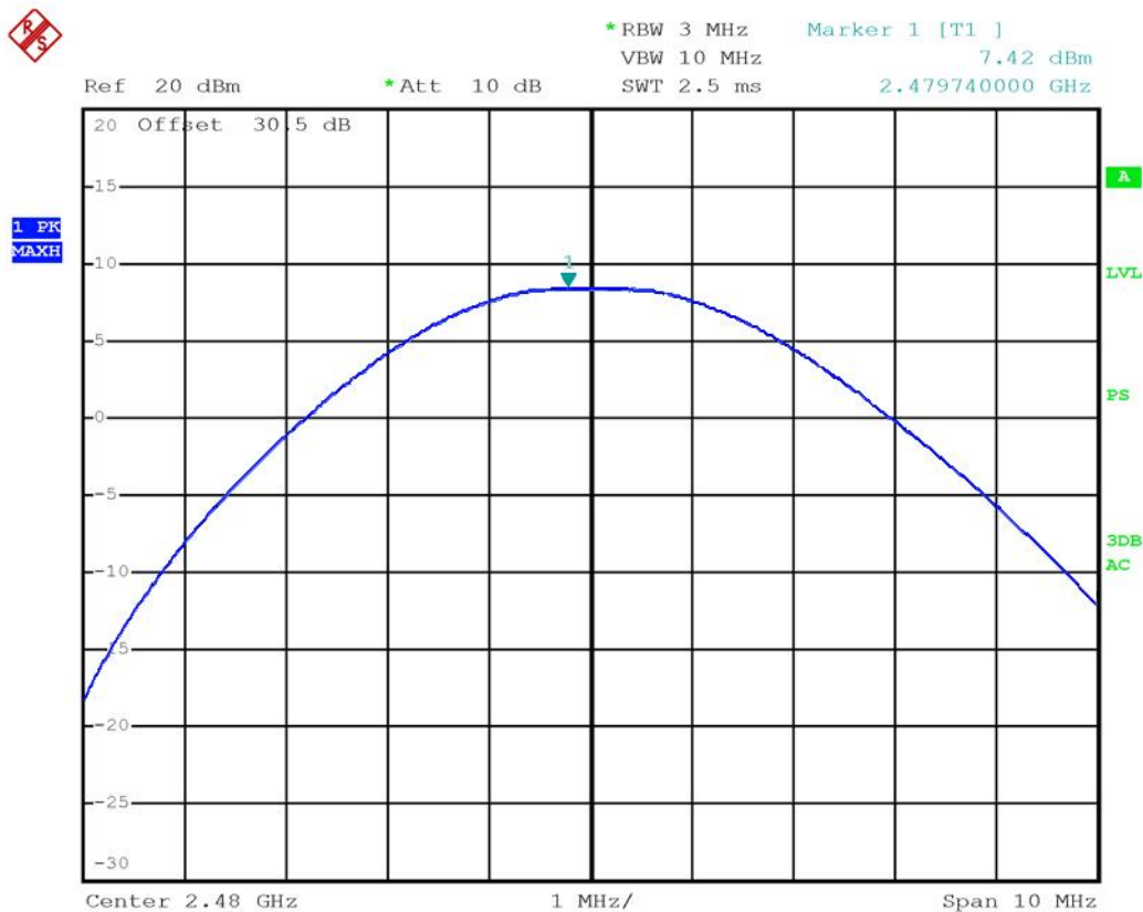
Figure 8.6-3: Output power of BLE, channel HIGH
