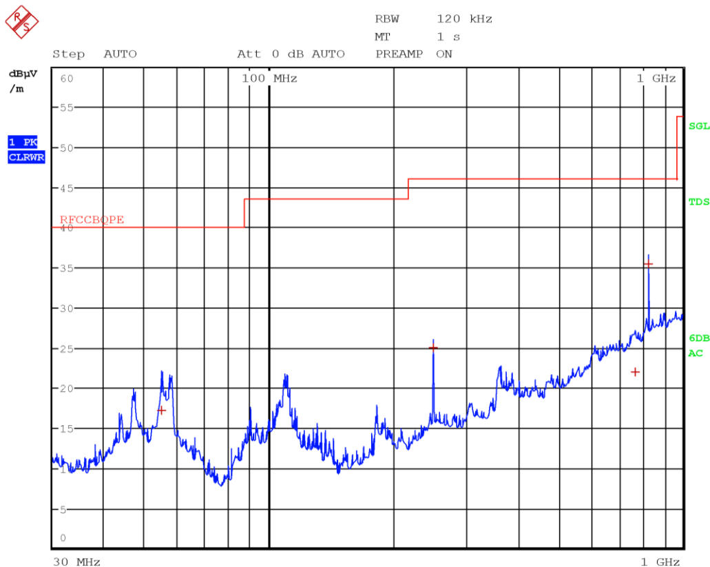
Figure 8.7-29: Radiated spurious emissions 30 to 1000 MHz, High channel with antenna in horizontal polarization
