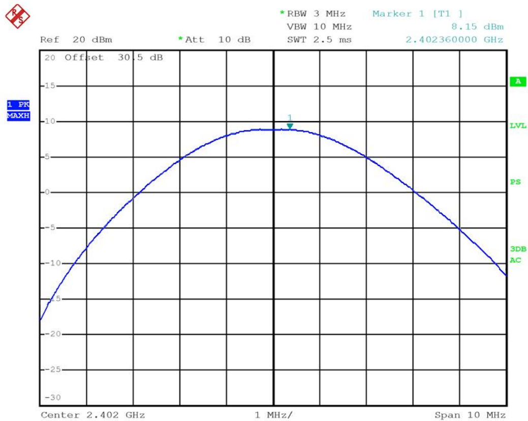
Figure 8.6-1: Output power of BLE, channel LOW
