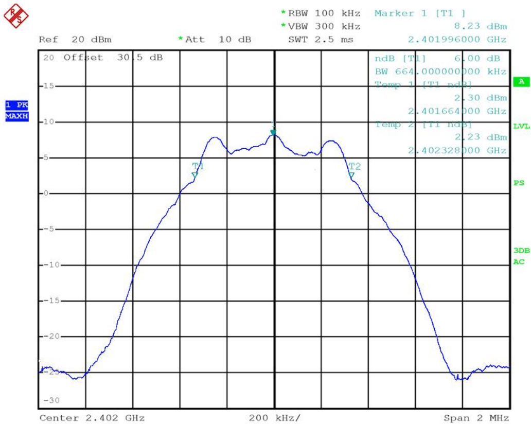
Figure 8.5-1: 6 dB bandwidth of BLE, channel LOW
