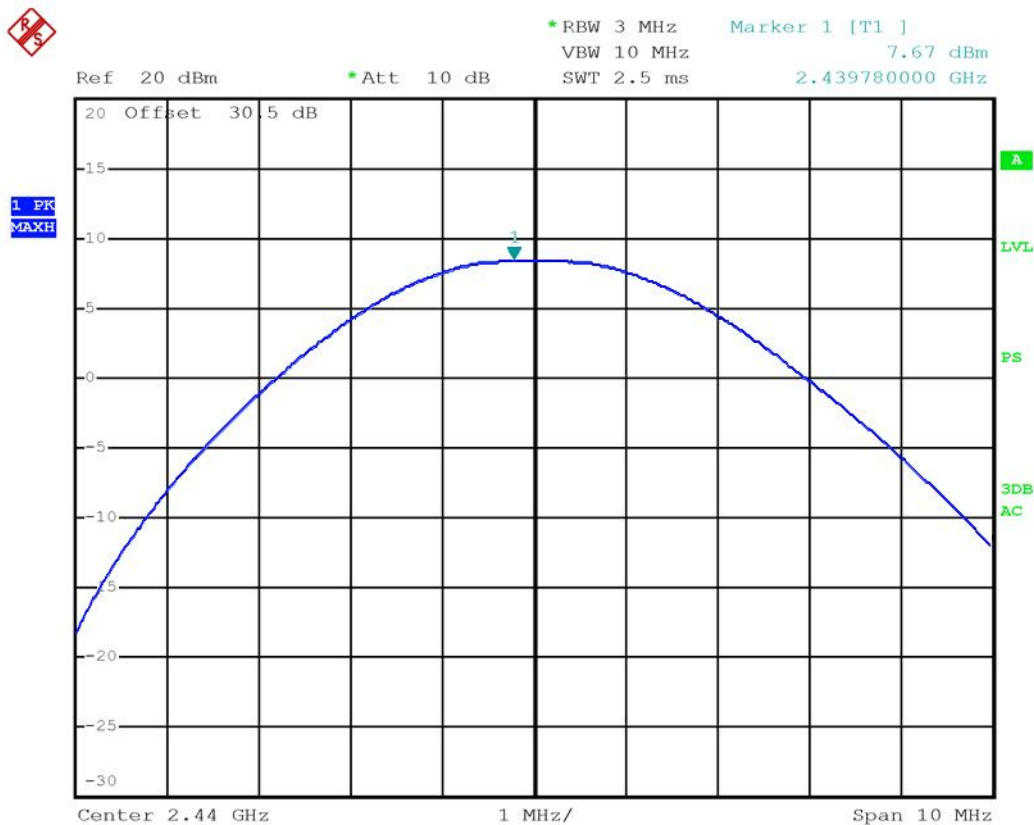
Figure 8.6-2: Output power of BLE, channel MID
