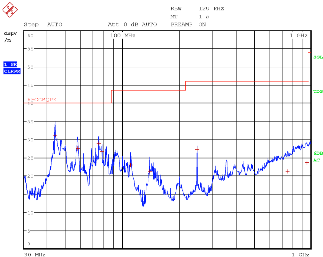
Figure 8.7-26: Radiated spurious emissions 30 to 1000 MHz, Low channel with antenna in vertical polarization
