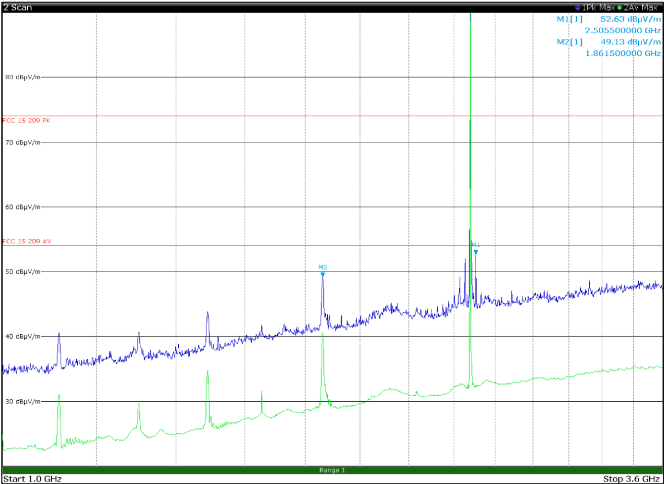
Figure 8.7-12: Radiated spurious emissions 1 to 3.6 GHz, High channel with antenna in vertical polarization
