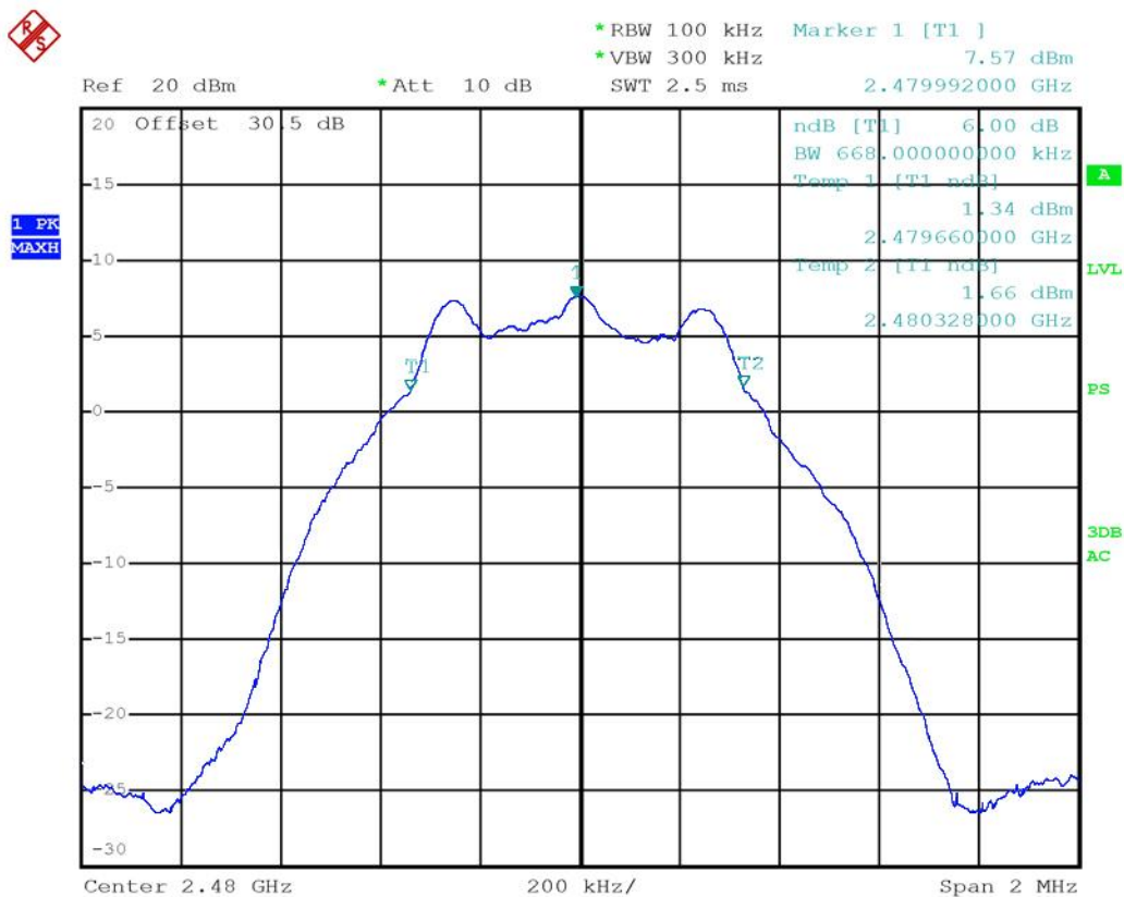
Figure 8.5-3: 6 dB bandwidth of BLE, channel HIGH
