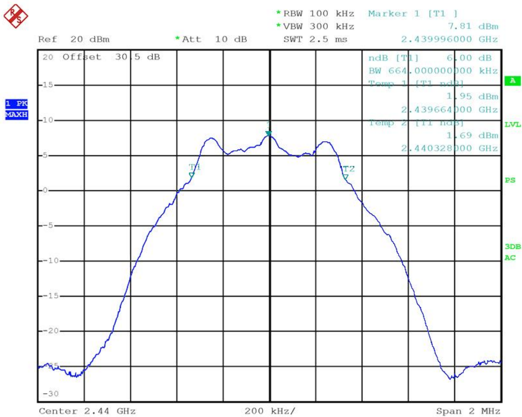
Figure 8.5-2: 6 dB bandwidth of BLE, channel MID
