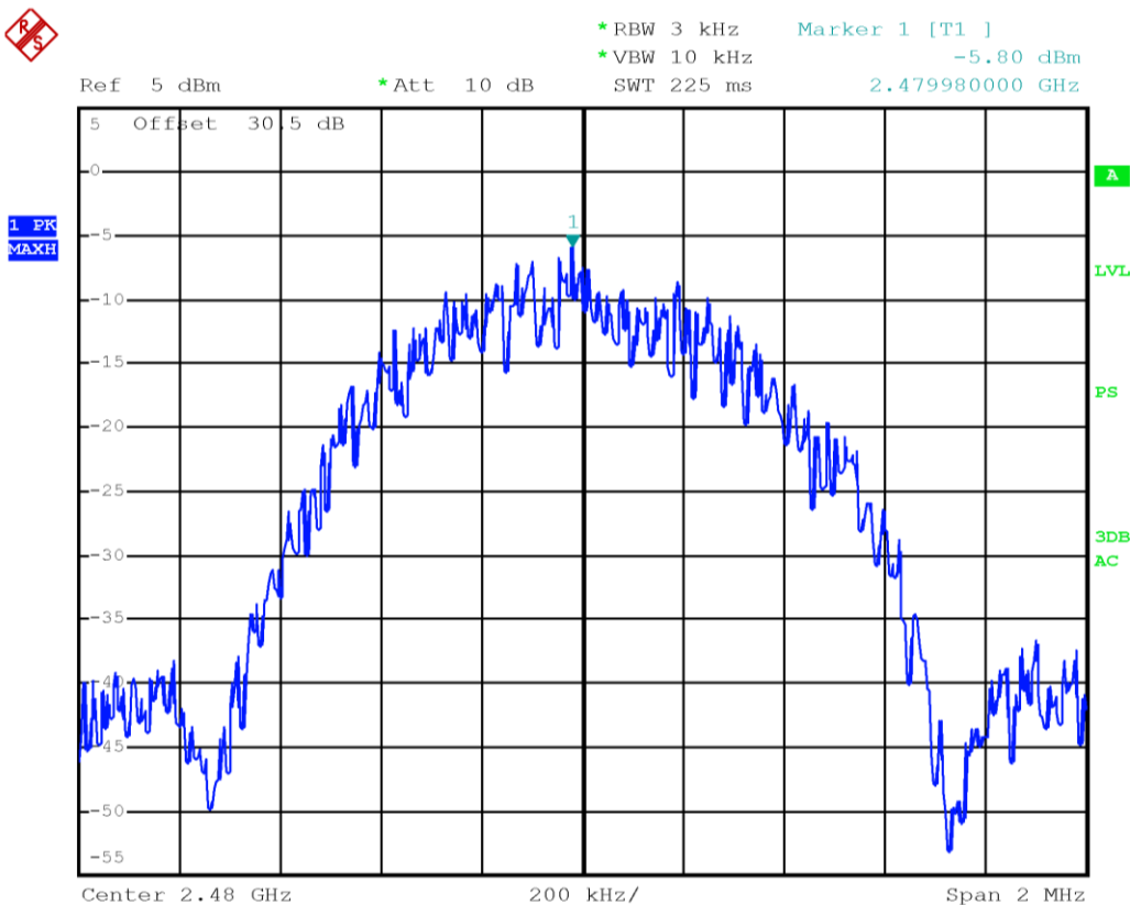
Figure 8.8-3: PSD sample plot on BLE - High channel
