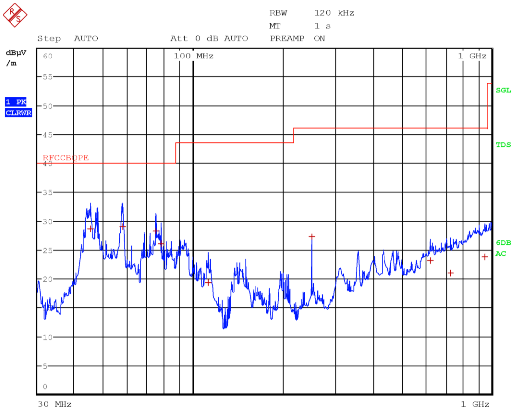
Figure 8.4-26: Radiated spurious emissions 30 to 1000 MHz, Low channel with antenna in vertical polarization
