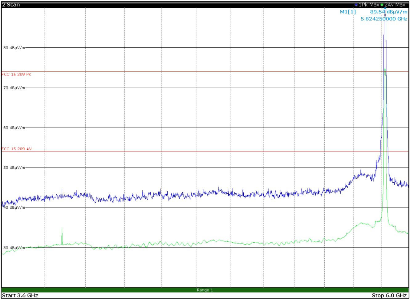
Figure 8.4-41: Radiated spurious emissions 3.6 to 6 GHz, high channel with antenna in horizontal polarization
