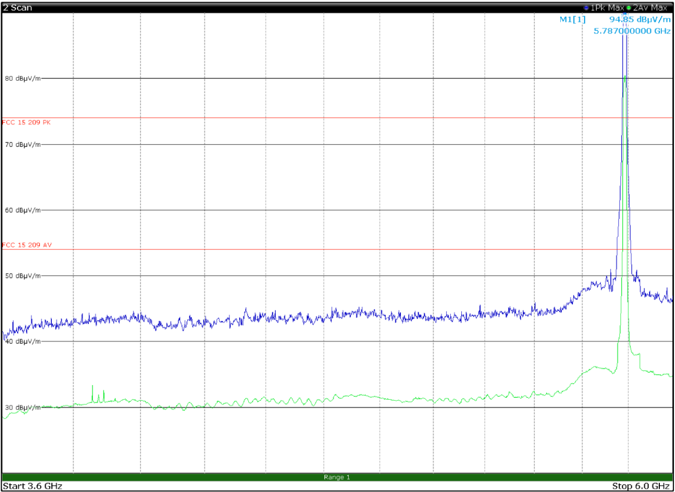
Figure 8.4-39: Radiated spurious emissions 3.6 to 6 GHz, mid channel with antenna in horizontal polarization Limit exceeded by the carrier
