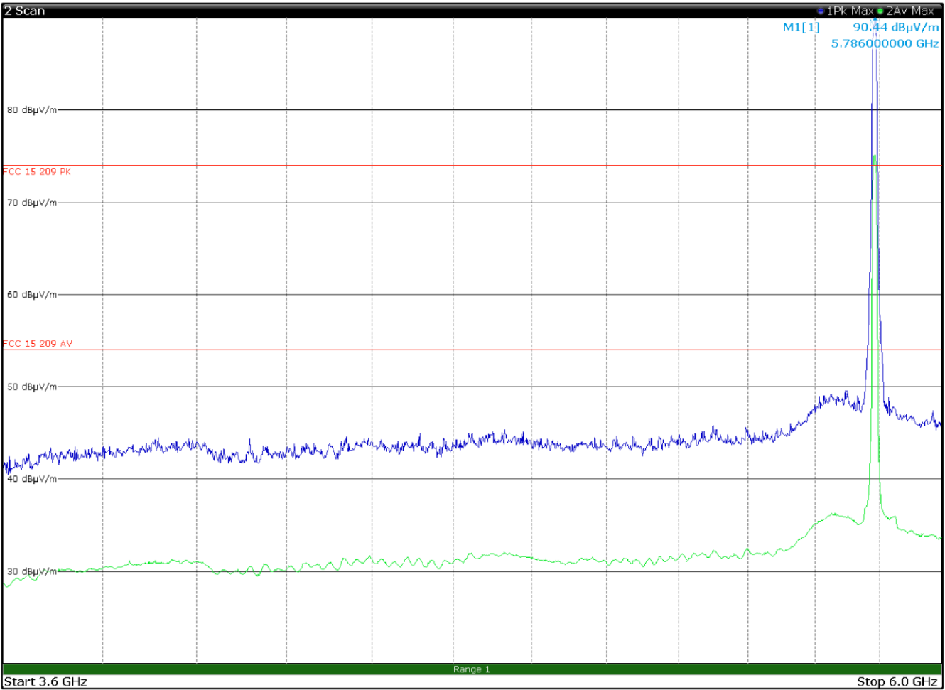
Figure 8.4-40: Radiated spurious emissions 3.6 to 6 GHz, mid channel with antenna in vertical polarization
