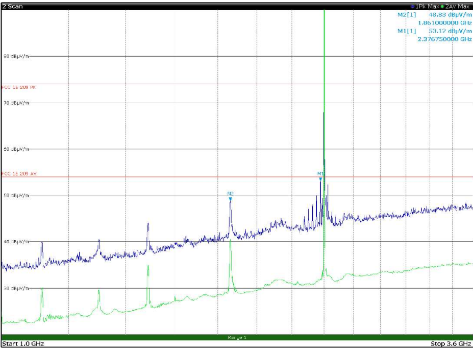
Figure 8.7-32: Radiated spurious emissions 1 to 3.6 GHz, Low channel with antenna in vertical polarization Limit exceeded by the carrier
