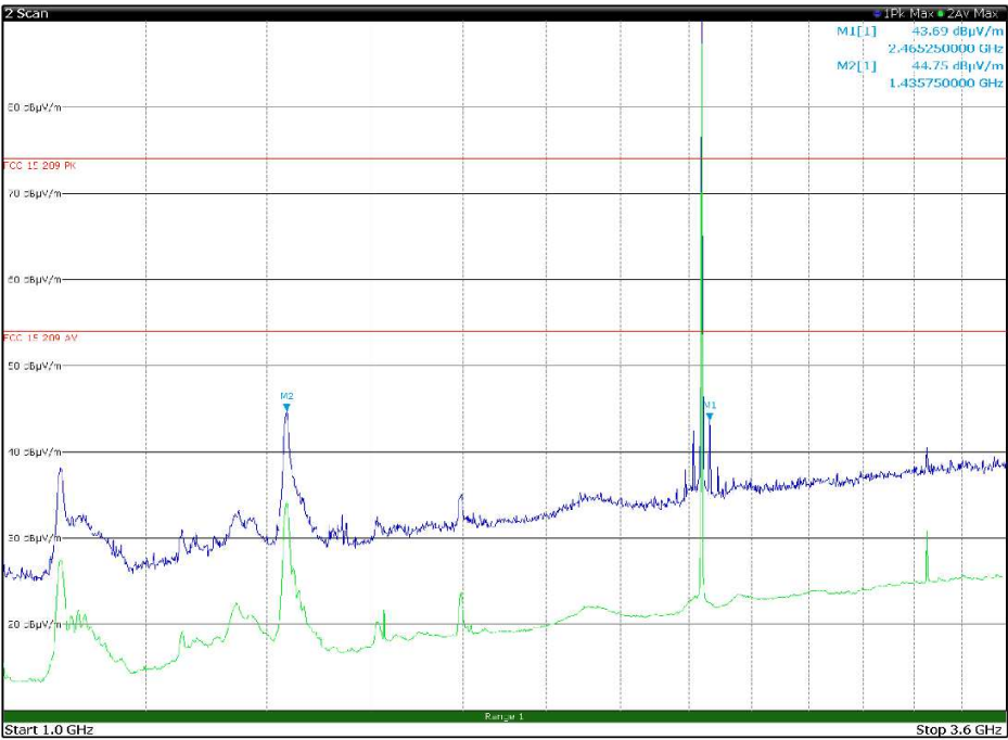
Figure 8.7-57: Radiated spurious emissions 1 to 3.6 GHz, Mid channel with antenna in horizontal polarization Limit exceeded by the carrier
