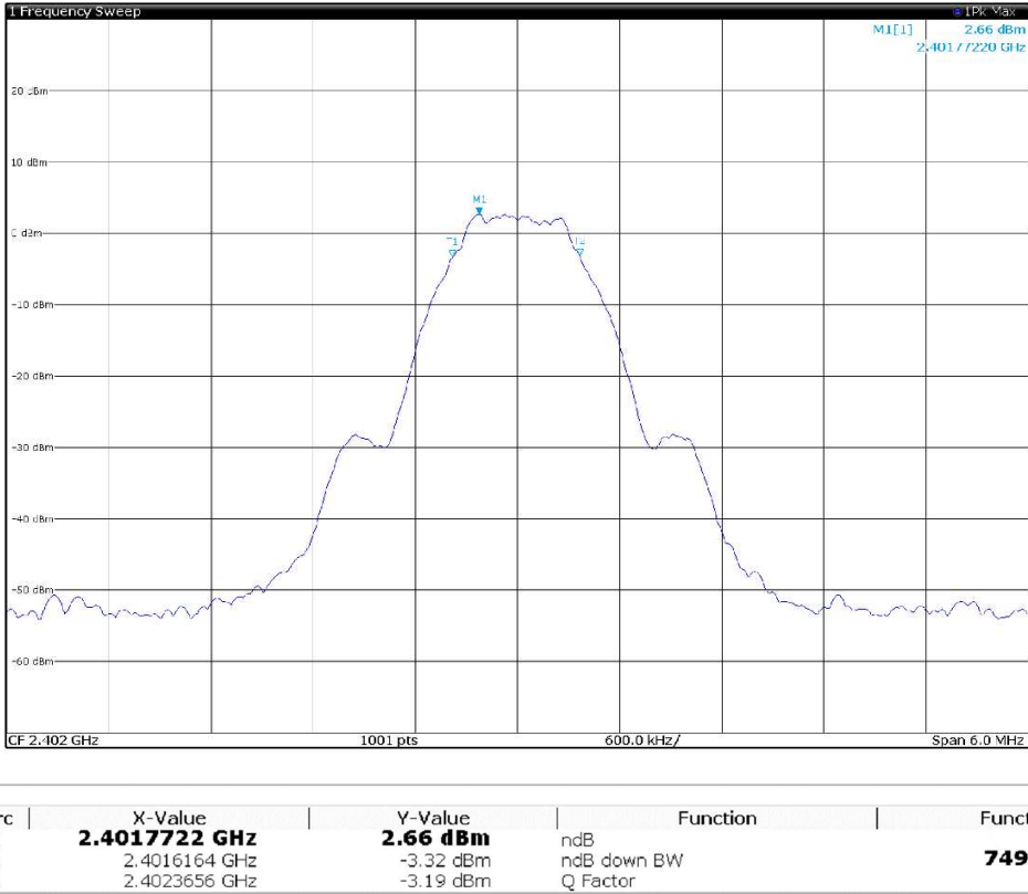
Figure 8.5-1: 6 dB bandwidth of BLE, channel LOW
