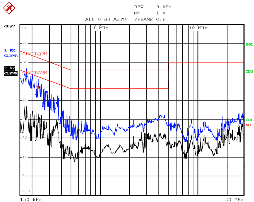
Plot 8.4-1: Conducted emissions on phase line
