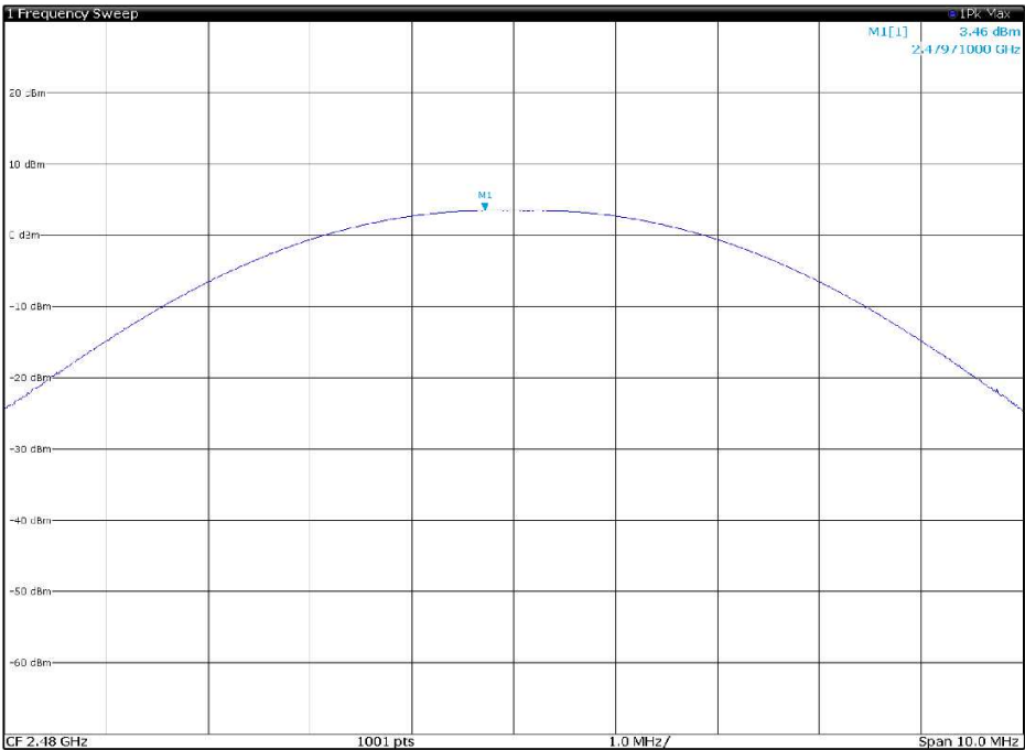
Figure 8.6-3: Output power of BLE, channel HIGH
