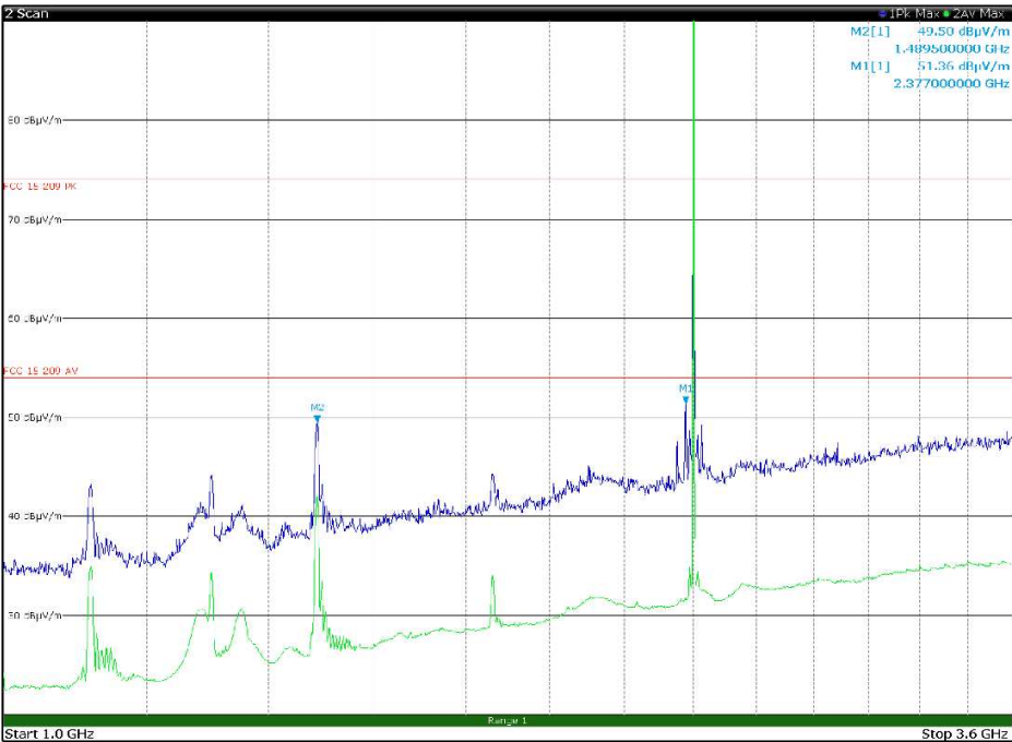
Figure 8.7-31: Radiated spurious emissions 1 to 3.6 GHz, Low channel with antenna in horizontal polarization Limit exceeded by the carrier
