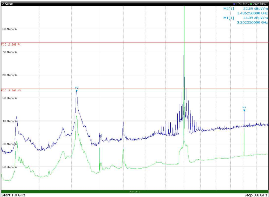
Figure 8.7-56: Radiated spurious emissions 1 to 3.6 GHz, Low channel with antenna in vertical polarization
