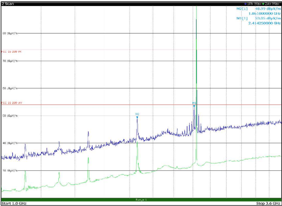
Figure 8.7-34: Radiated spurious emissions 1 to 3.6 GHz, Mid channel with antenna in vertical polarization Limit exceeded by the carrier
