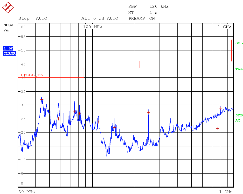
Figure 8.7-52: Radiated spurious emissions 30 to 1000 MHz, Mid channel with antenna in vertical polarization
