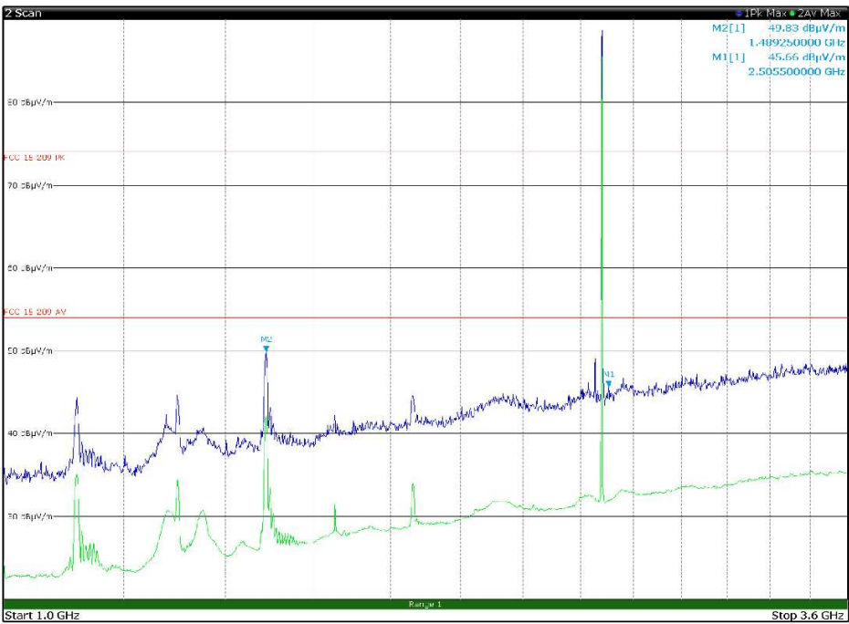
Figure 8.7-35: Radiated spurious emissions 1 to 3.6 GHz, High channel with antenna in horizontal polarization Limit exceeded by the carrier
