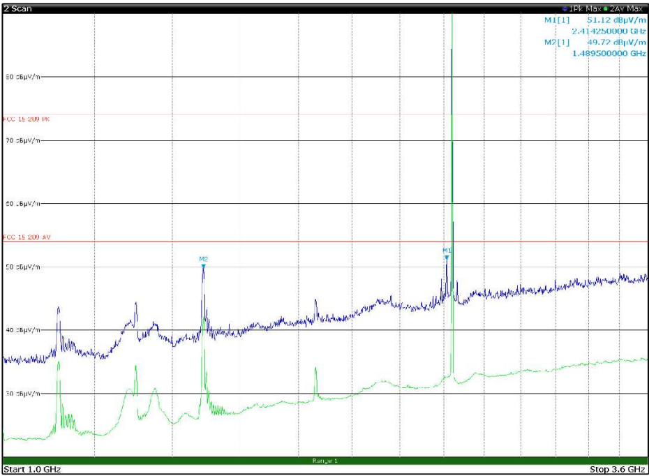
Figure 8.7-33: Radiated spurious emissions 1 to 3.6 GHz, Mid channel with antenna in horizontal polarization Limit exceeded by the carrier
