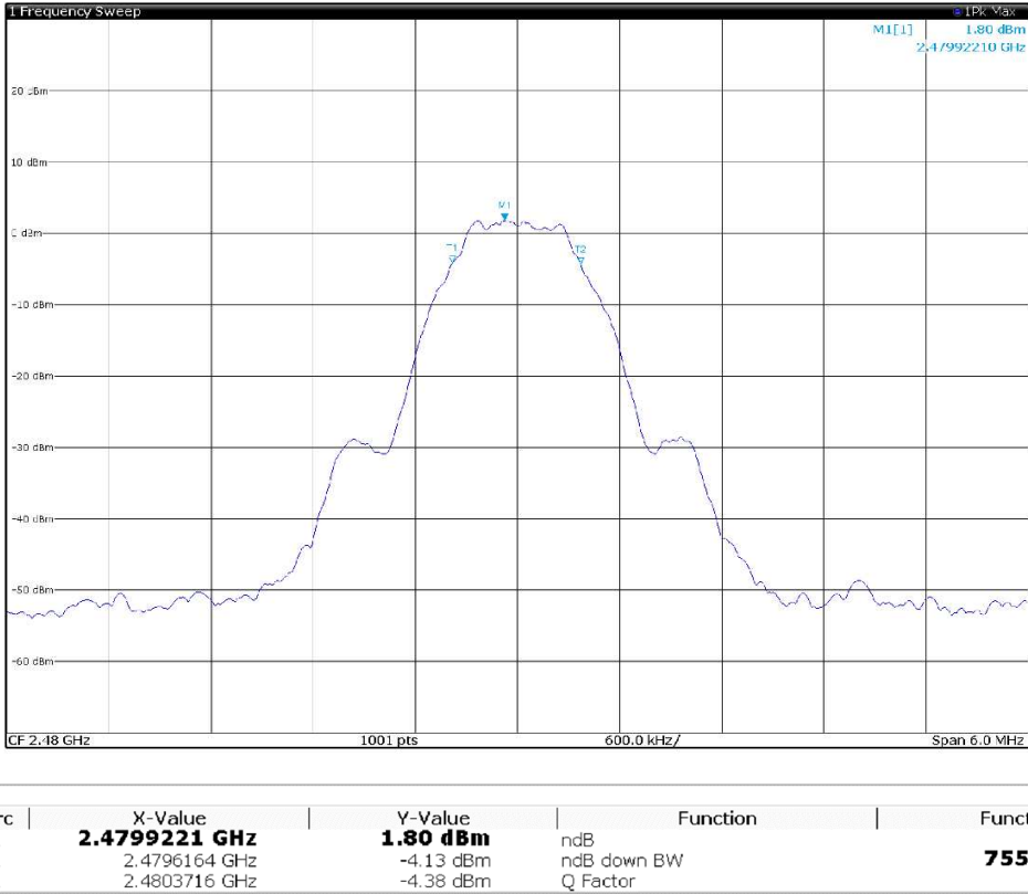
Figure 8.5-3: 6 dB bandwidth of BLE, channel HIGH
