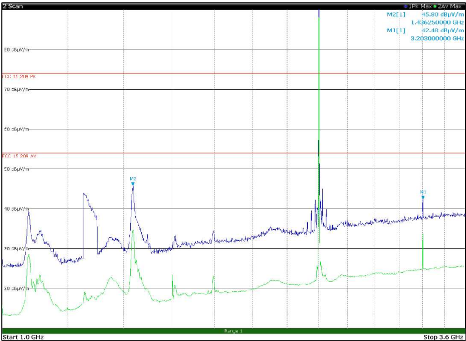
Figure 8.7-55: Radiated spurious emissions 1 to 3.6 GHz, Low channel with antenna in horizontal polarization
