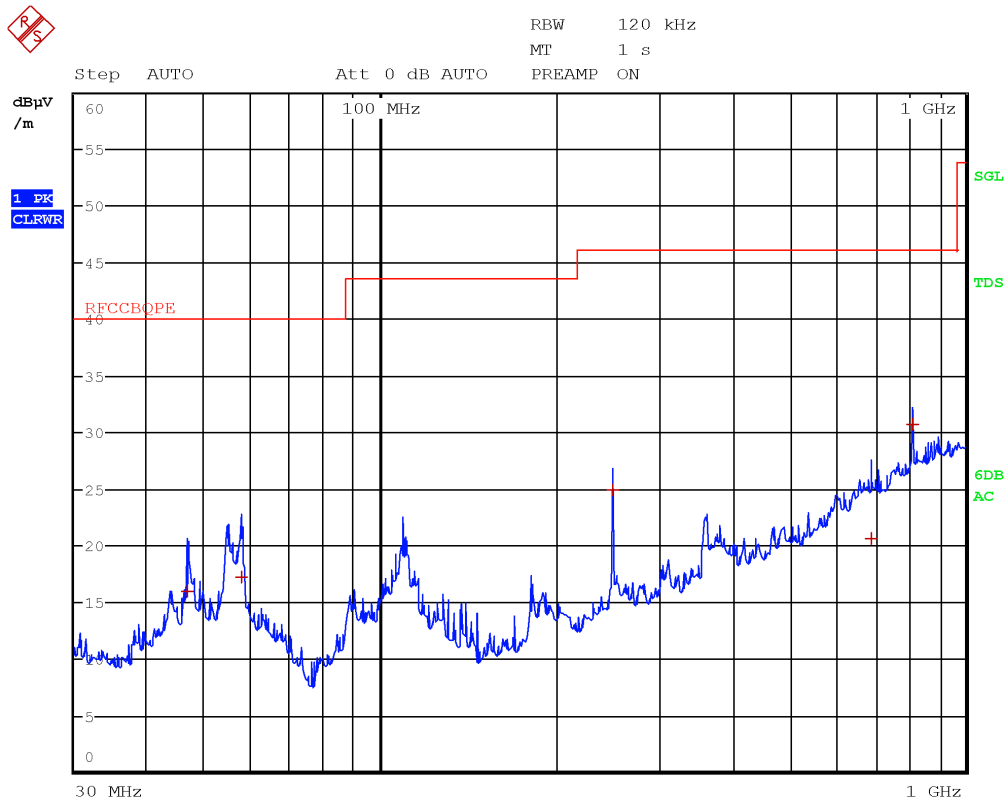
Figure 8.7-51: Radiated spurious emissions 30 to 1000 MHz, Mid channel with antenna in horizontal polarization
