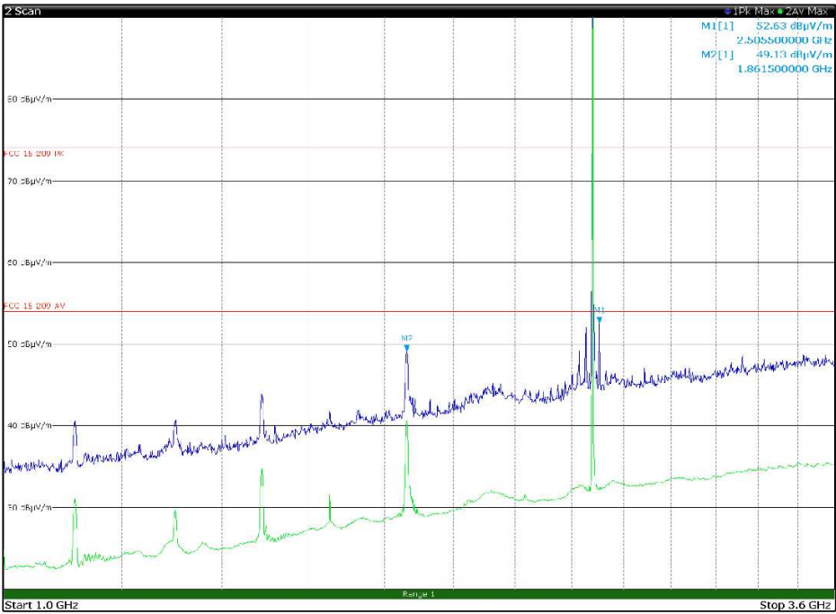
Figure 8.7-36: Radiated spurious emissions 1 to 3.6 GHz, High channel with antenna in vertical polarization Limit exceeded by the carrier
