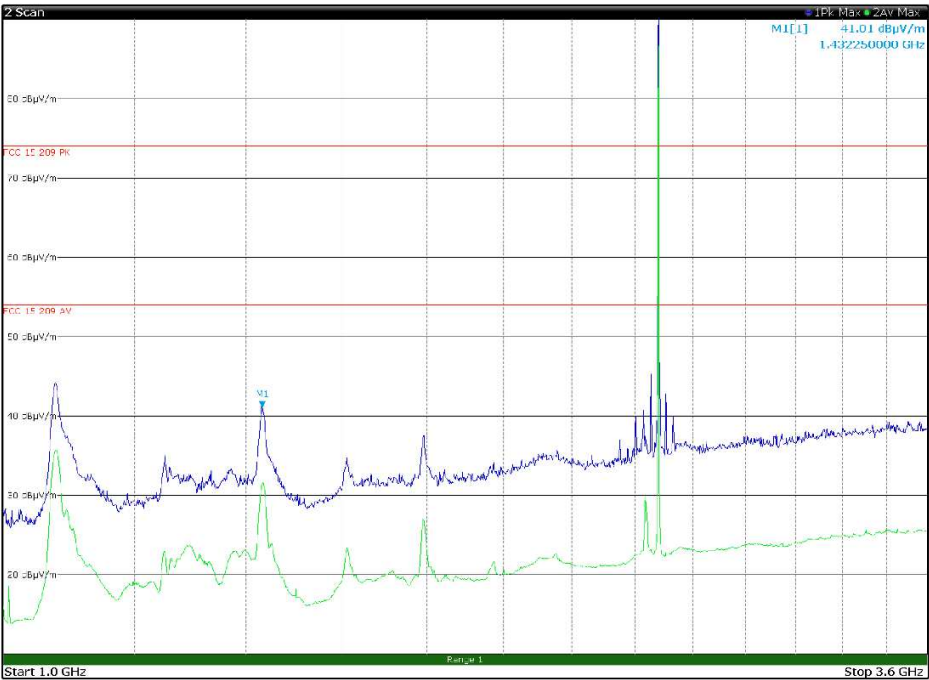
Figure 8.7-11: Radiated spurious emissions 1 to 3.6 GHz, High channel with antenna in horizontal polarization Limit exceeded by the carrier
