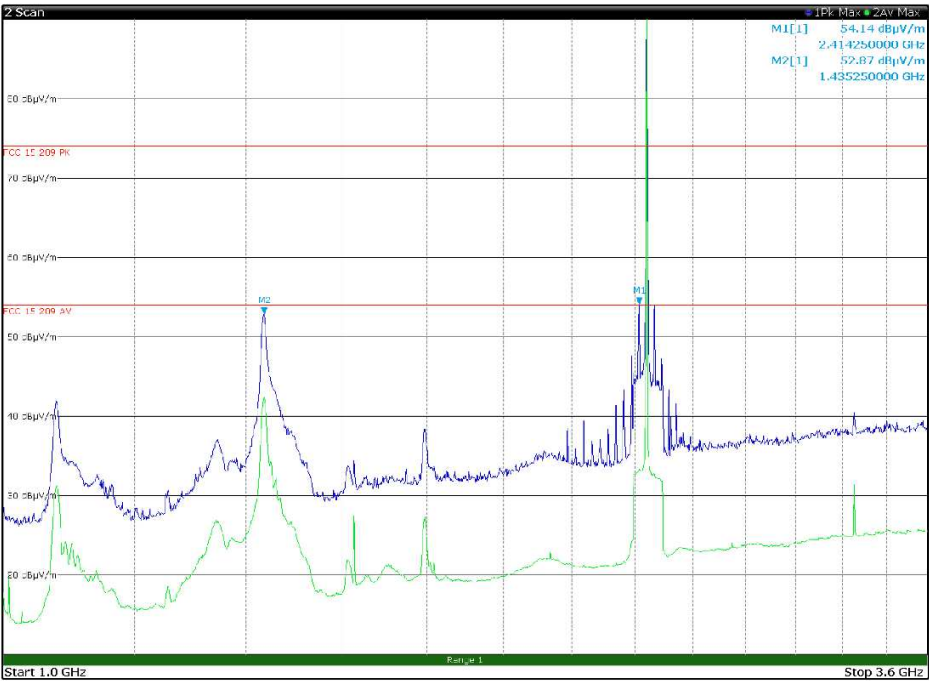
Figure 8.7-58: Radiated spurious emissions 1 to 3.6 GHz, Mid channel with antenna in vertical polarization Limit exceeded by the carrier
