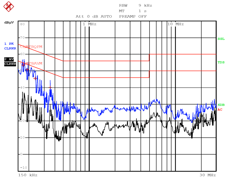
Plot 8.4-2: Conducted emissions on neutral line
