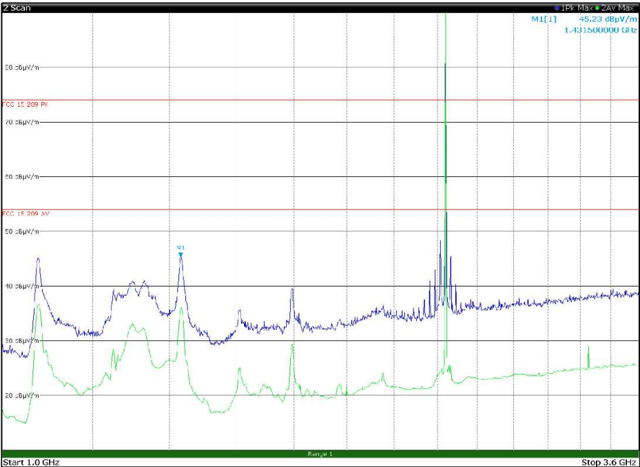
Figure 8.7-10: Radiated spurious emissions 1 to 3.6 GHz, Mid channel with antenna in vertical polarization Limit exceeded by the carrier
