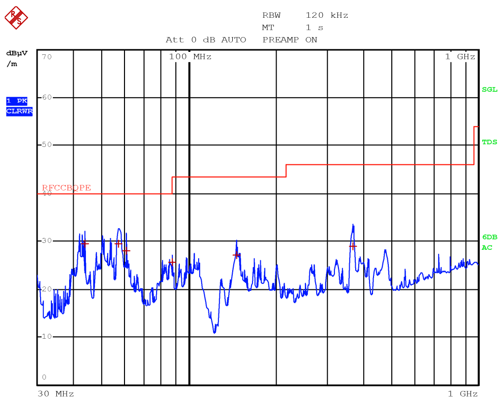
Figure 8.7-2: Radiated spurious emissions 30 to 1000 MHz, Low channel with antenna in vertical polarization
