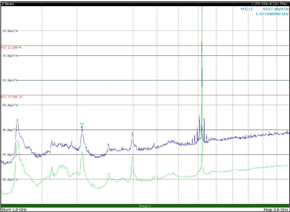
Figure 8.7-9: Radiated spurious emissions 1 to 3.6 GHz, Mid channel with antenna in horizontal polarization Limit exceeded by the carrier
