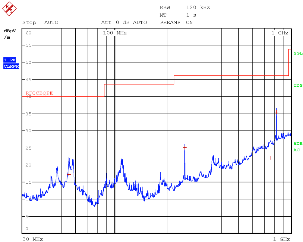
Figure 8.7-53: Radiated spurious emissions 30 to 1000 MHz, High channel with antenna in horizontal polarization
