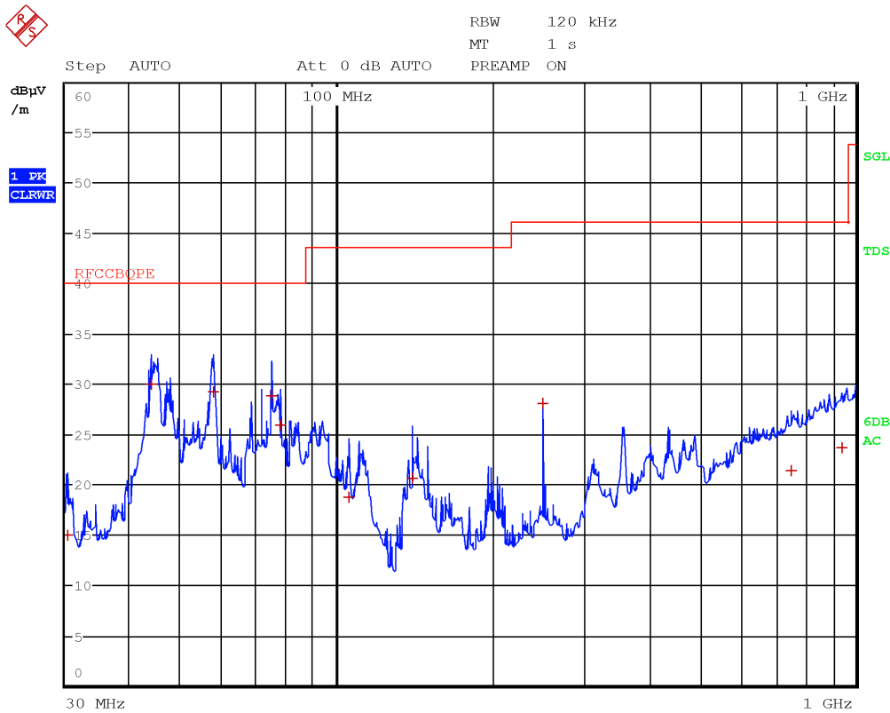
Figure 8.4-78: Radiated spurious emissions 30 to 1000 MHz, high channel with antenna in vertical polarization
