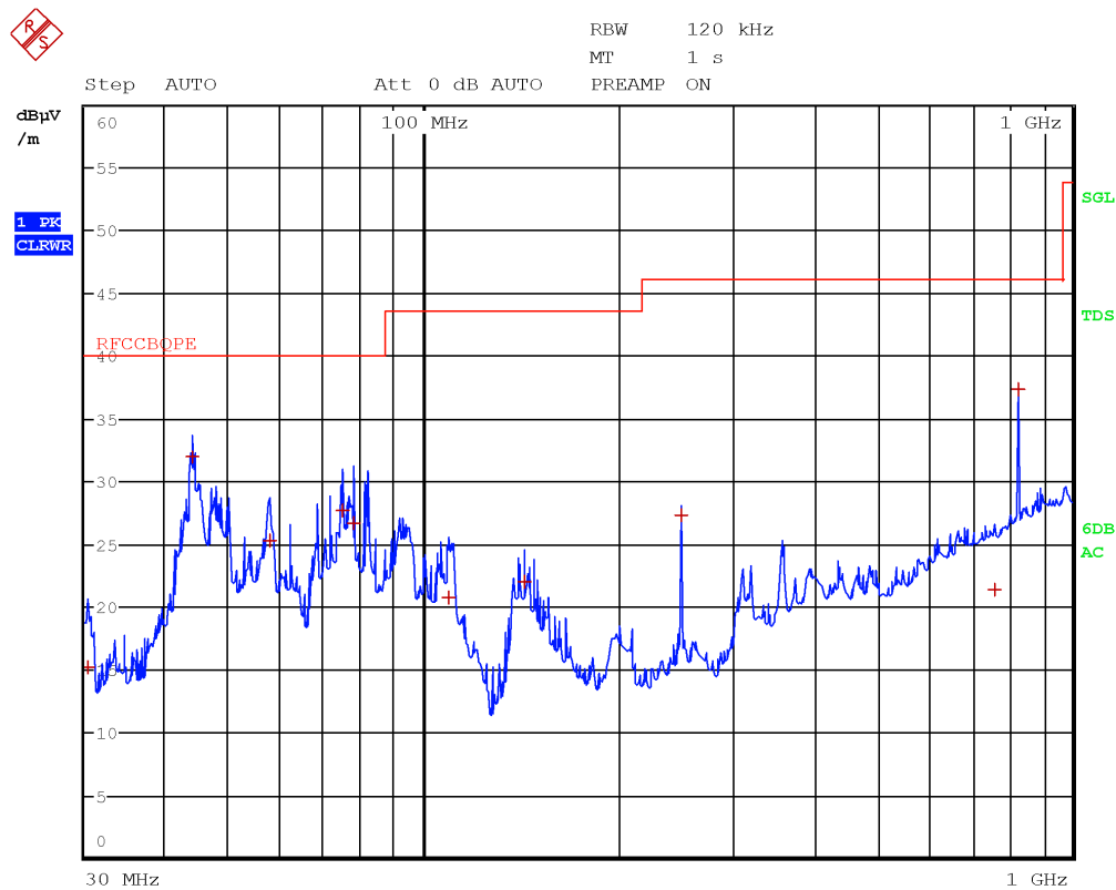
Figure 8.7-78: Radiated spurious emissions 30 to 1000 MHz, High channel with antenna in vertical polarization
