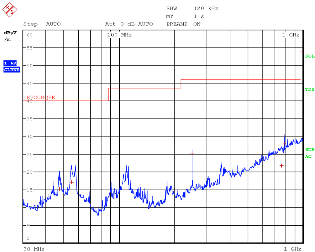
Figure 8.7-73: Radiated spurious emissions 30 to 1000 MHz, Low channel with antenna in horizontal polarization
