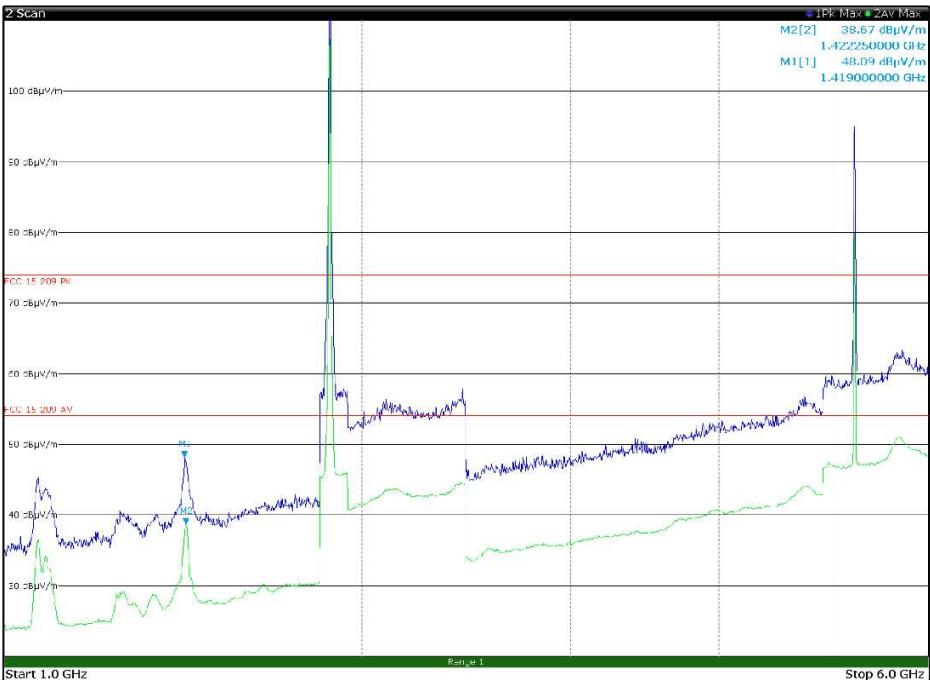
Figure 8.1-28: Radiated spurious emissions, LTE Tx at 1883 MHz, WIFI Tx at 5200 MHz – antenna in vertical polarization – EUT in configuration 1
