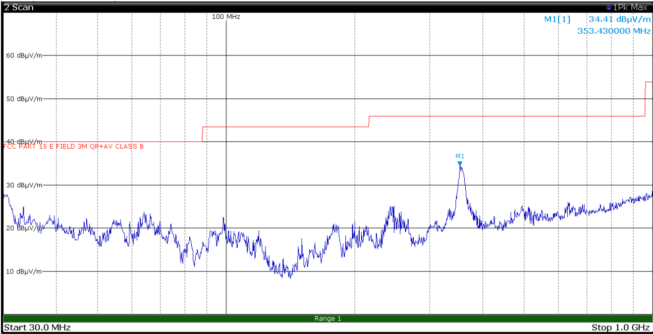
Figure 8.1-18: Radiated spurious emissions, LTE Tx at 1883 MHz, WIFI Tx at 2412 MHz – antenna in vertical polarization – EUT in configuration 1
