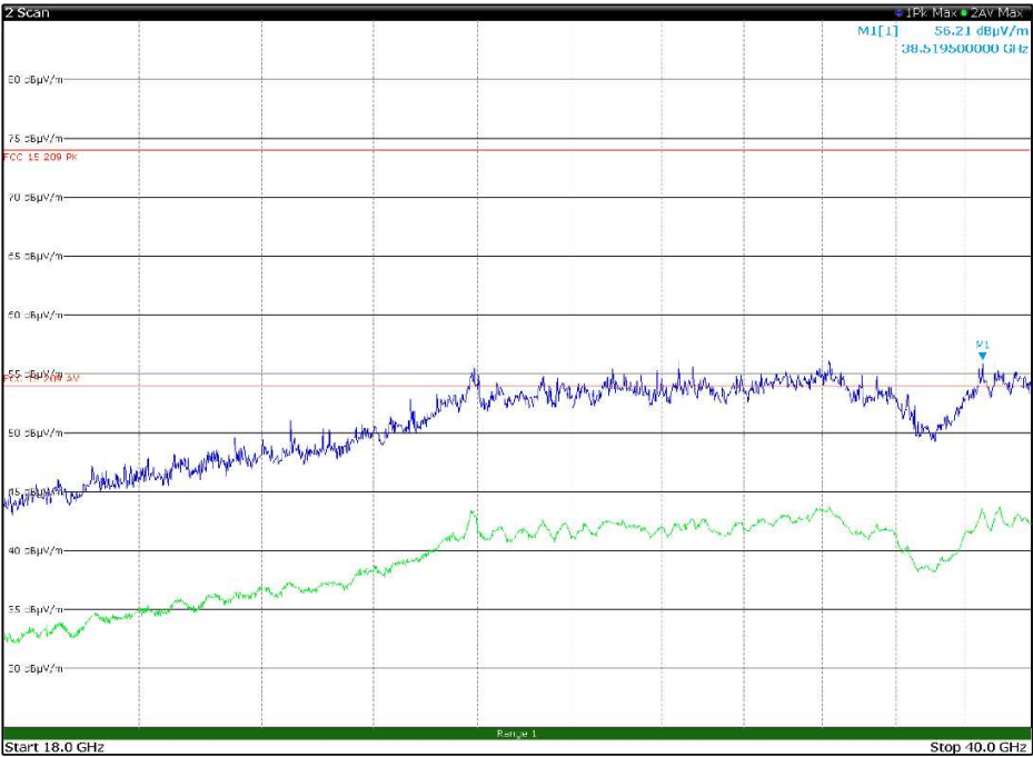
Figure 8.1-64: Radiated spurious emissions, LTE Tx at 1883 MHz, WIFI Tx at 5200 MHz – antenna in vertical polarization – EUT in configuration 2
