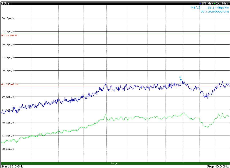
Figure 8.1-47: Radiated spurious emissions, LTE Tx at 782 MHz, WIFI Tx at 5200 MHz – antenna in horizontal polarization – EUT in configuration 2
