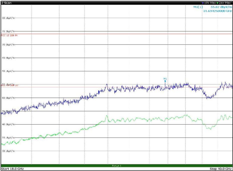
Figure 8.1-48: Radiated spurious emissions, LTE Tx at 782 MHz, WIFI Tx at 5200 MHz – antenna in vertical polarization – EUT in configuration 2
