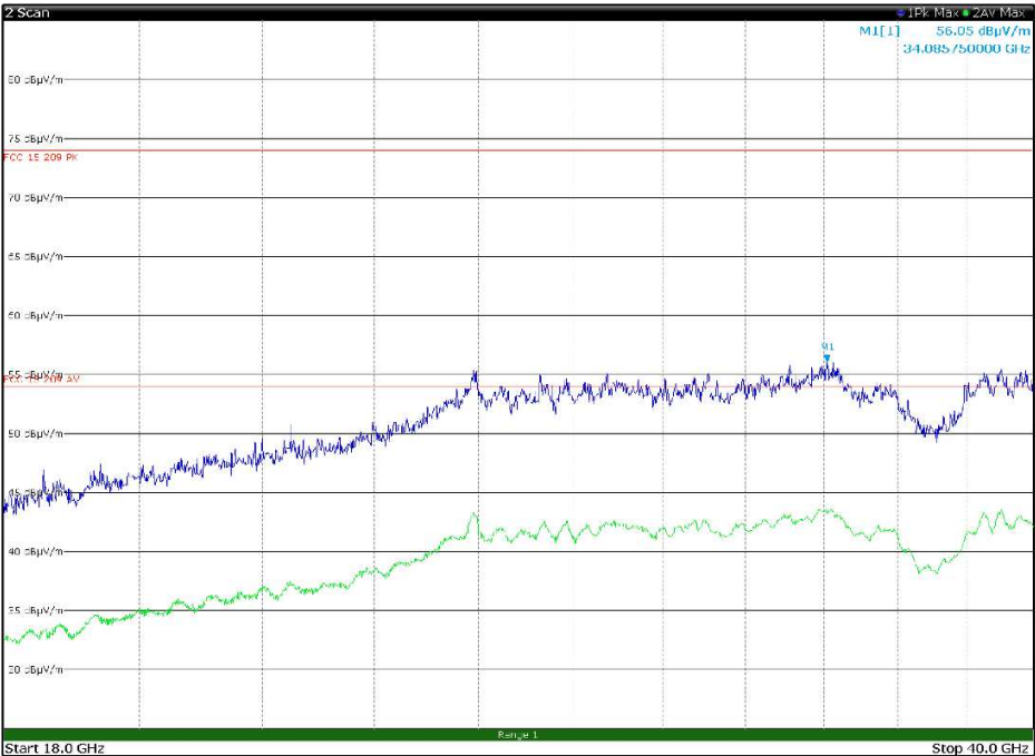
Figure 8.1-39: Radiated spurious emissions, LTE Tx at 782 MHz, WIFI Tx at 2412 MHz – antenna in horizontal polarization – EUT in configuration 2
