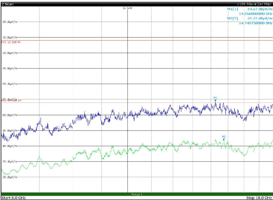
Figure 8.1-61: Radiated spurious emissions, LTE Tx at 1883 MHz, WIFI Tx at 5200 MHz – antenna in horizontal polarization – EUT in configuration 2
