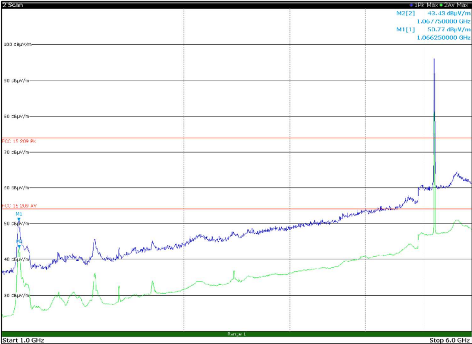
Figure 8.1-43: Radiated spurious emissions, LTE Tx at 782 MHz, WIFI Tx at 5200 MHz – antenna in horizontal polarization – EUT in configuration 2
