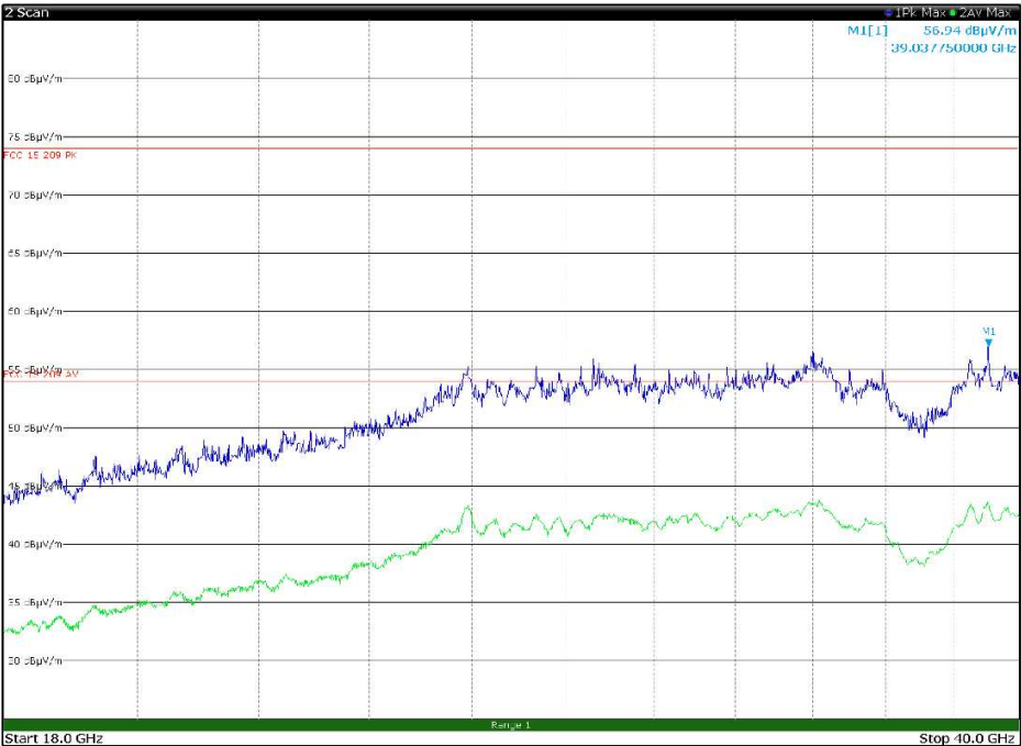
Figure 8.1-31: Radiated spurious emissions, LTE Tx at 1883 MHz, WIFI Tx at 5200 MHz – antenna in horizontal polarization – EUT in configuration 1
