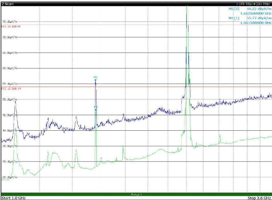
Figure 8.1-36: Radiated spurious emissions, LTE Tx at 782 MHz, WIFI Tx at 2412 MHz – antenna in vertical polarization – EUT in configuration 2
