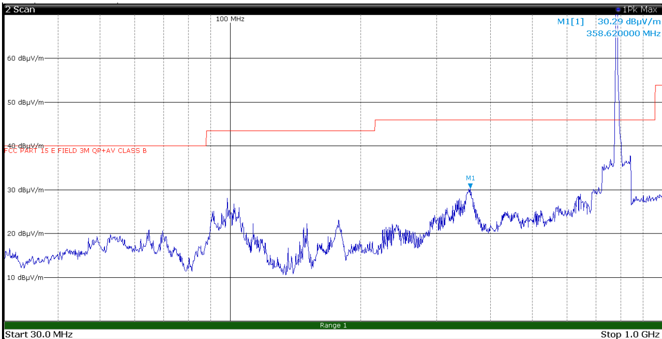
Figure 8.1-1: Radiated spurious emissions, LTE Tx at 782 MHz, WIFI Tx at 2412 MHz – antenna in horizontal polarization – EUT in configuration 1
