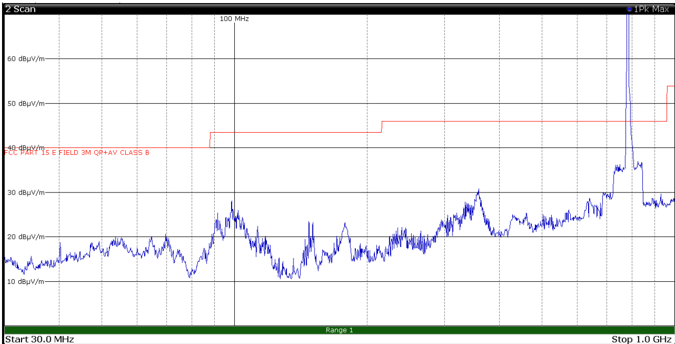
Figure 8.1-65: Radiated spurious emissions, LTE Tx at 782 MHz, WIFI Tx at 2412 MHz – antenna in horizontal polarization – EUT in configuration 1
