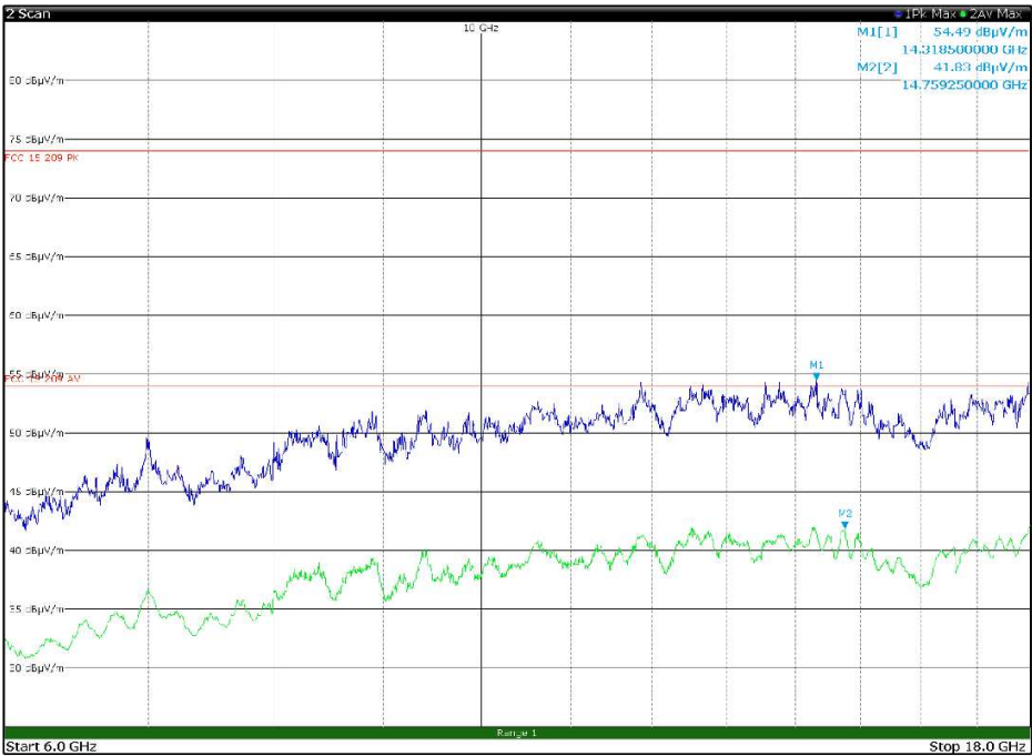
Figure 8.1-30: Radiated spurious emissions, LTE Tx at 1883 MHz, WIFI Tx at 5200 MHz – antenna in vertical polarization – EUT in configuration 1
