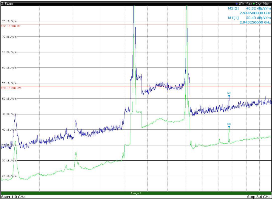
Figure 8.1-52: Radiated spurious emissions, LTE Tx at 1883 MHz, WIFI Tx at 2412 MHz – antenna in vertical polarization – EUT in configuration 2
