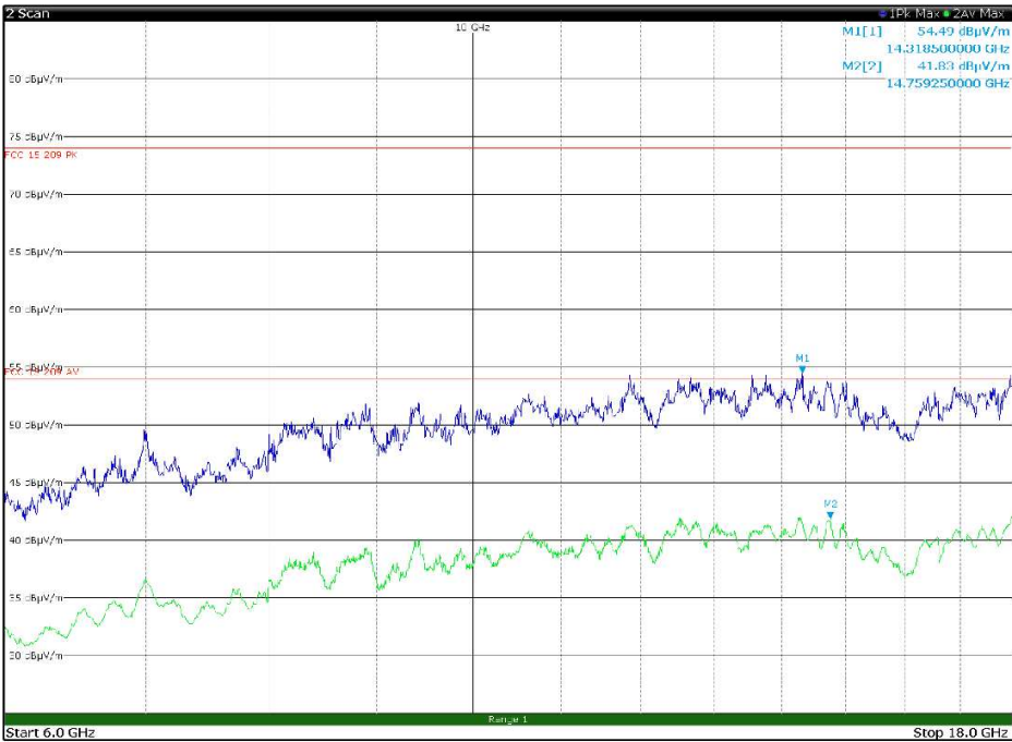
Figure 8.1-62: Radiated spurious emissions, LTE Tx at 1883 MHz, WIFI Tx at 5200 MHz – antenna in vertical polarization – EUT in configuration 2
