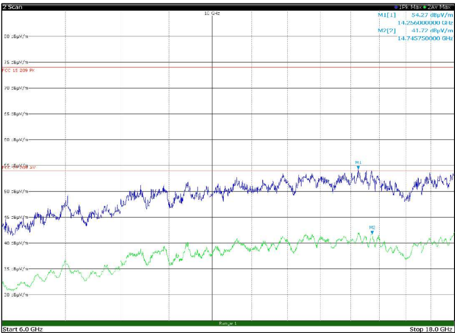
Figure 8.1-29: Radiated spurious emissions, LTE Tx at 1883 MHz, WIFI Tx at 5200 MHz – antenna in horizontal polarization – EUT in configuration 1
