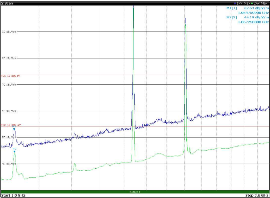
Figure 8.1-19: Radiated spurious emissions, LTE Tx at 1883 MHz, WIFI Tx at 2412 MHz – antenna in horizontal polarization – EUT in configuration 1
