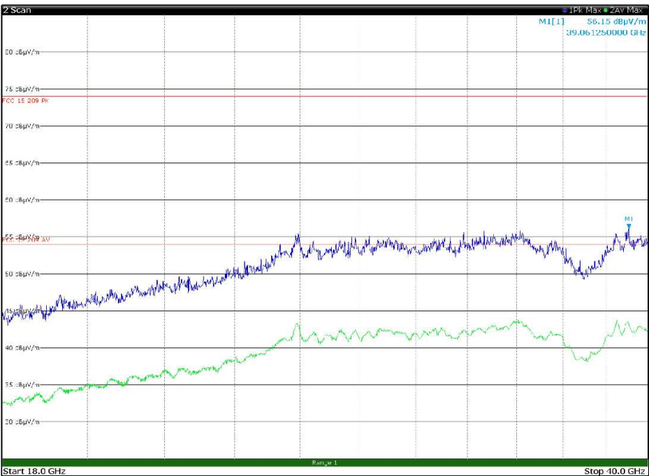
Figure 8.1-63: Radiated spurious emissions, LTE Tx at 1883 MHz, WIFI Tx at 5200 MHz – antenna in horizontal polarization – EUT in configuration 2
