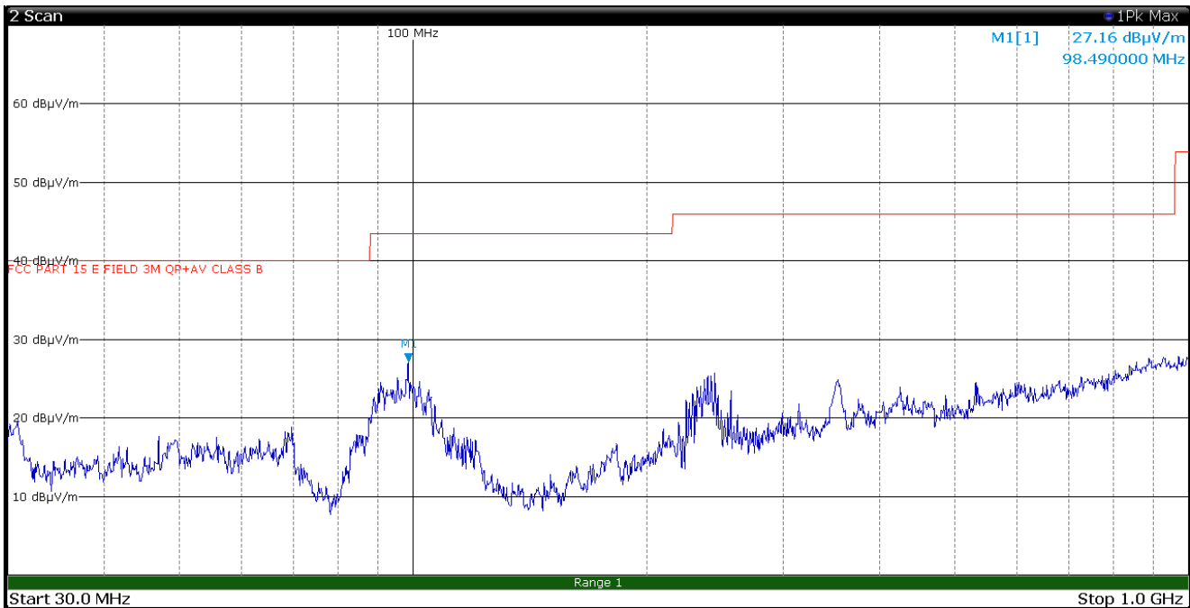
Figure 8.1-25: Radiated spurious emissions, LTE Tx at 1883 MHz, WIFI Tx at 5200 MHz – antenna in horizontal polarization – EUT in configuration 1
