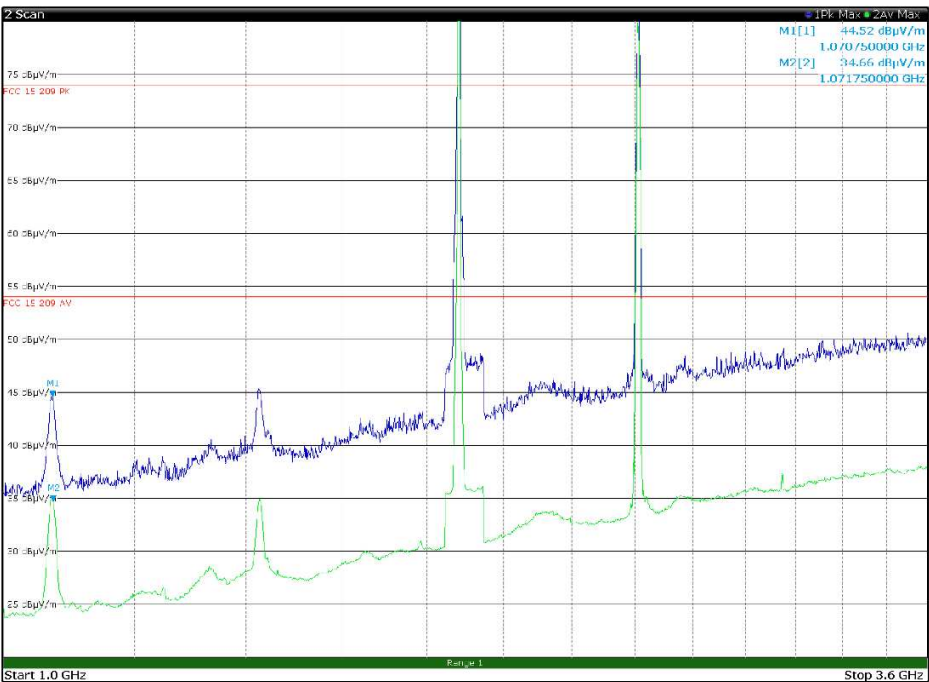
Figure 8.1-51: Radiated spurious emissions, LTE Tx at 1883 MHz, WIFI Tx at 2412 MHz – antenna in horizontal polarization – EUT in configuration 2
