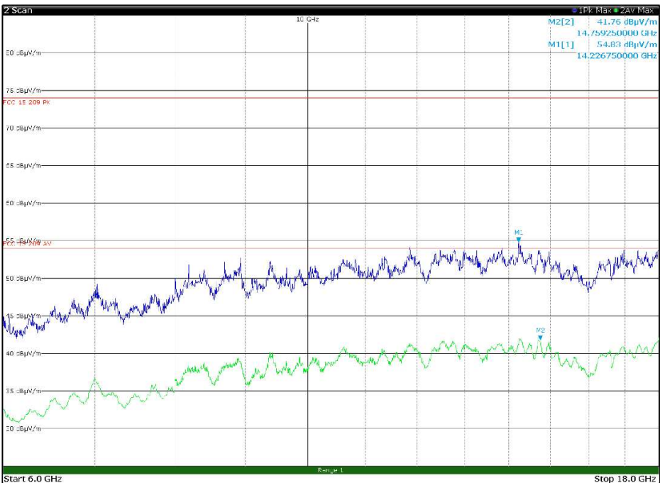
Figure 8.1-46: Radiated spurious emissions, LTE Tx at 782 MHz, WIFI Tx at 5200 MHz – antenna in vertical polarization – EUT in configuration 2
