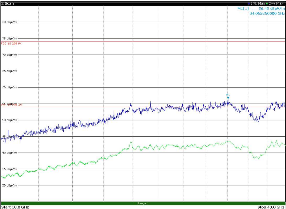
Figure 8.1-32: Radiated spurious emissions, LTE Tx at 1883 MHz, WIFI Tx at 5200 MHz – antenna in vertical polarization – EUT in configuration 1
