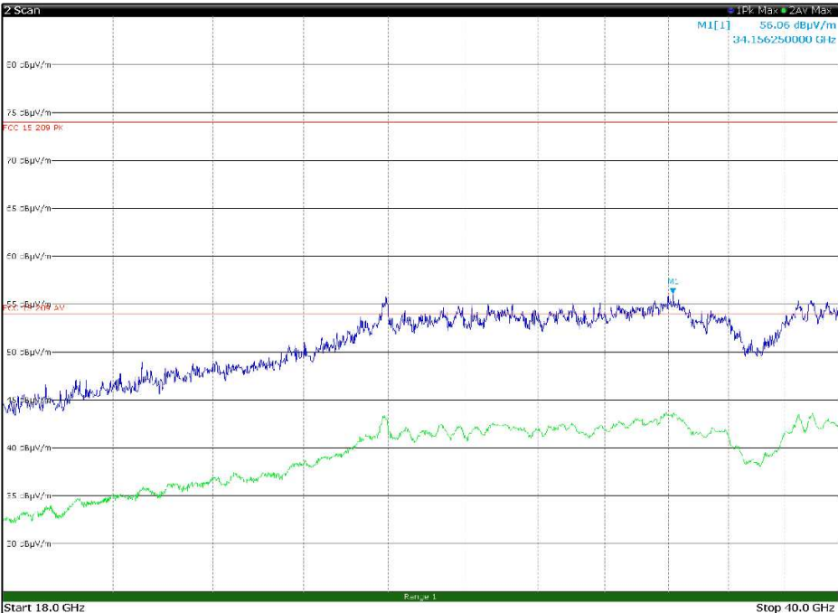
Figure 8.1-56: Radiated spurious emissions, LTE Tx at 1883 MHz, WIFI Tx at 2412 MHz – antenna in vertical polarization – EUT in configuration 2
