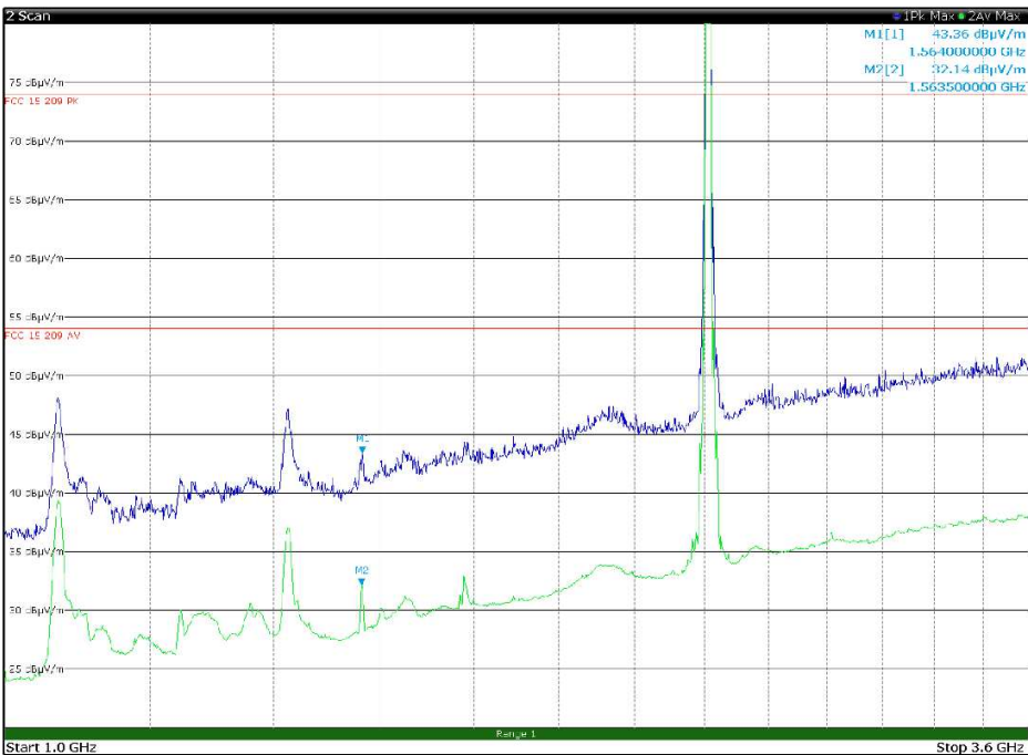
Figure 8.1-35: Radiated spurious emissions, LTE Tx at 782 MHz, WIFI Tx at 2412 MHz – antenna in horizontal polarization – EUT in configuration 2
