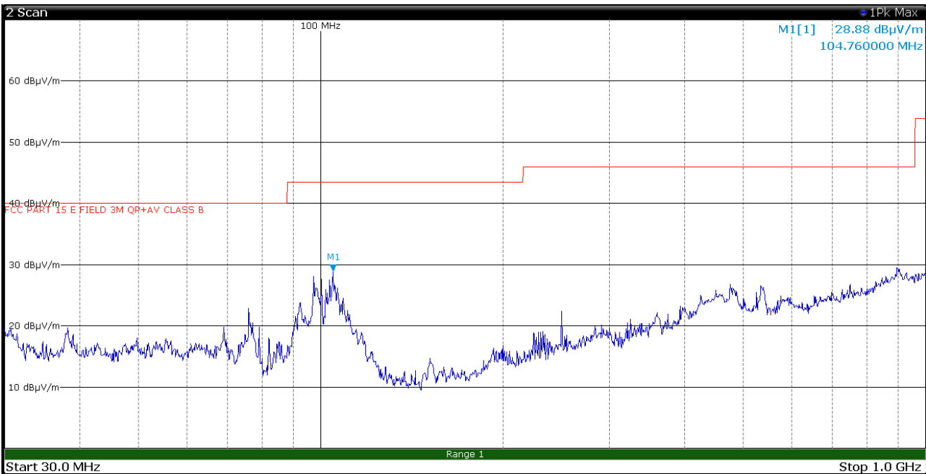
Figure 8.1-57: Radiated spurious emissions, LTE Tx at 1883 MHz, WIFI Tx at 5200 MHz – antenna in horizontal polarization – EUT in configuration 2
