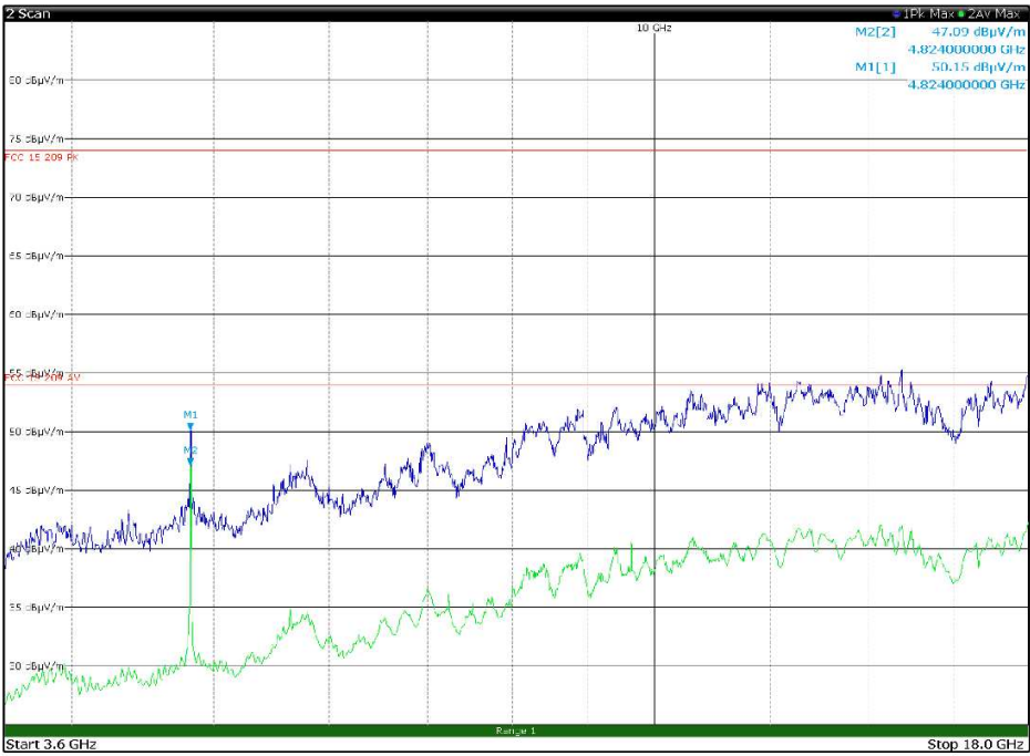
Figure 8.1-22: Radiated spurious emissions, LTE Tx at 1883 MHz, WIFI Tx at 2412 MHz – antenna in vertical polarization – EUT in configuration 1
