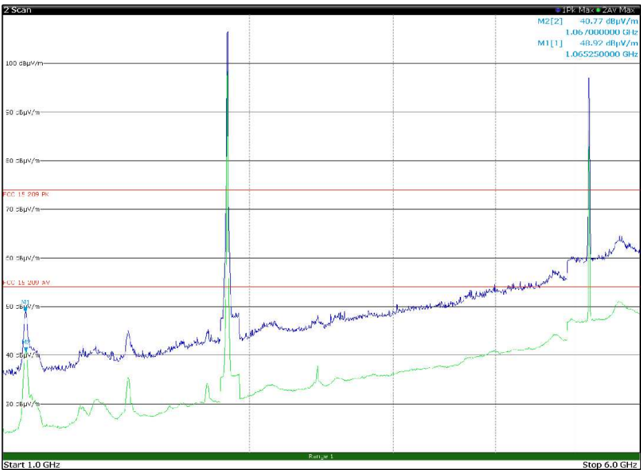
Figure 8.1-27: Radiated spurious emissions, LTE Tx at 1883 MHz, WIFI Tx at 5200 MHz – antenna in horizontal polarization – EUT in configuration 1
