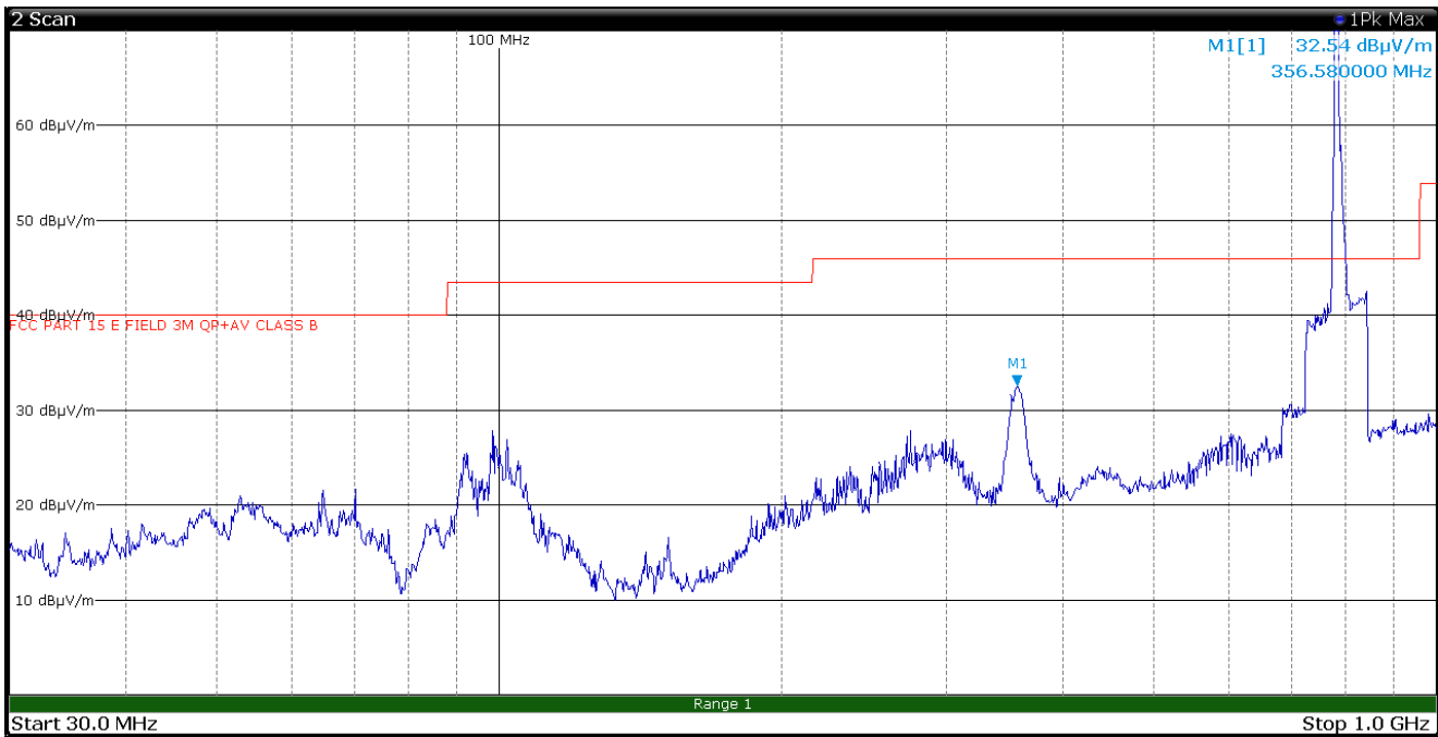
Figure 8.1-33: Radiated spurious emissions, LTE Tx at 782 MHz, WIFI Tx at 2412 MHz – antenna in horizontal polarization – EUT in configuration 2
