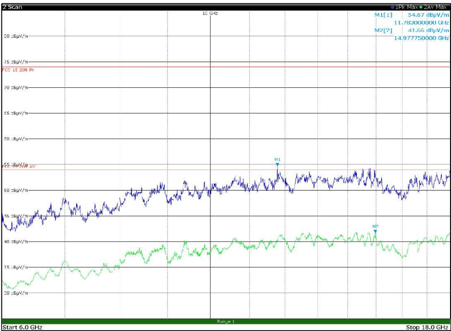
Figure 8.1-45: Radiated spurious emissions, LTE Tx at 782 MHz, WIFI Tx at 5200 MHz – antenna in horizontal polarization – EUT in configuration 2
