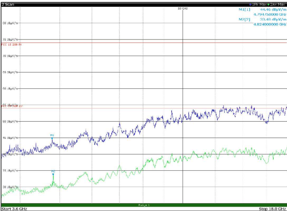
Figure 8.1-37: Radiated spurious emissions, LTE Tx at 782 MHz, WIFI Tx at 2412 MHz – antenna in horizontal polarization – EUT in configuration 2
