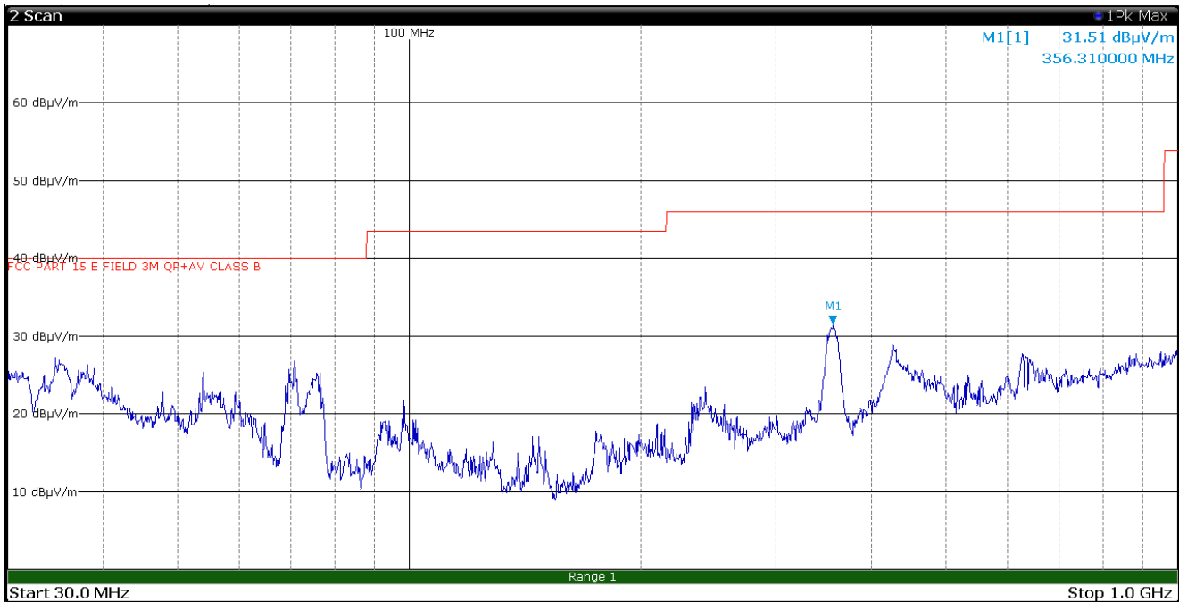
Figure 8.1-26: Radiated spurious emissions, LTE Tx at 1883 MHz, WIFI Tx at 5200 MHz – antenna in vertical polarization – EUT in configuration 1
