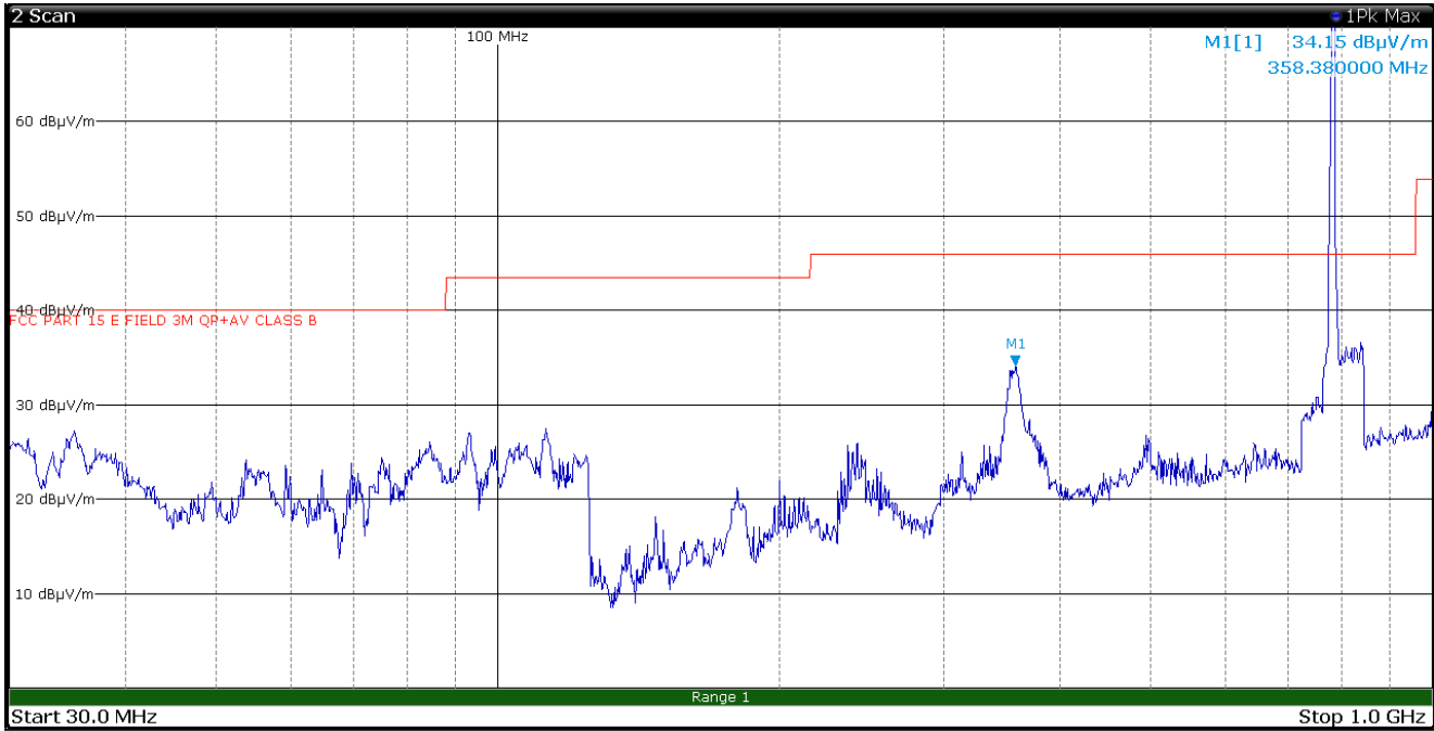
Figure 8.1-10: Radiated spurious emissions, LTE Tx at 782 MHz, WIFI Tx at 5200 MHz – antenna in vertical polarization – EUT in configuration 1
