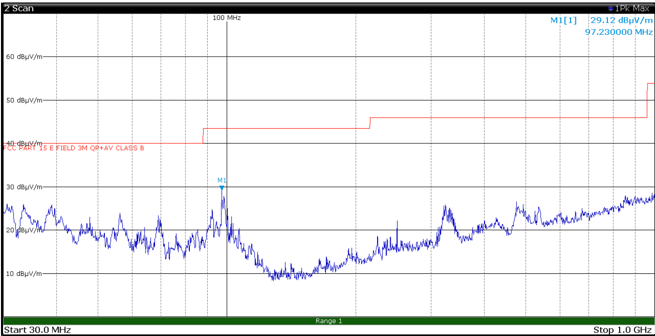
Figure 8.1-58: Radiated spurious emissions, LTE Tx at 1883 MHz, WIFI Tx at 5200 MHz – antenna in vertical polarization – EUT in configuration 2
