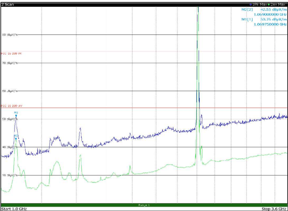
Figure 8.1-67: Radiated spurious emissions, LTE Tx at 782 MHz, WIFI Tx at 2412 MHz – antenna in horizontal polarization – EUT in configuration 1
