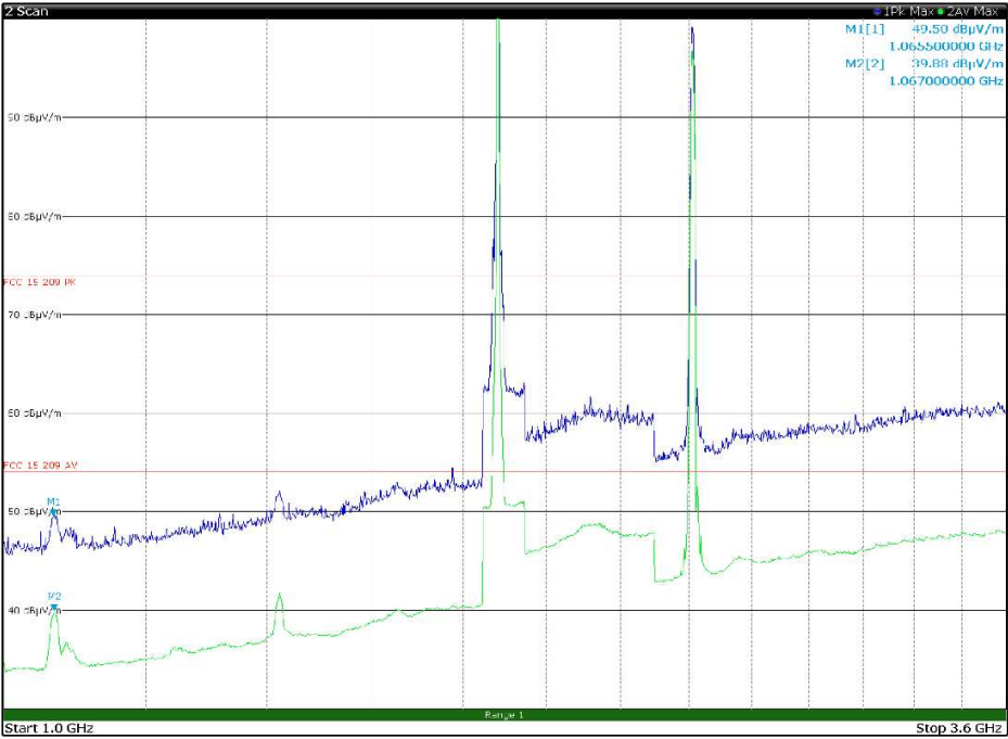
Figure 8.1-20: Radiated spurious emissions, LTE Tx at 1883 MHz, WIFI Tx at 2412 MHz – antenna in vertical polarization – EUT in configuration 1
