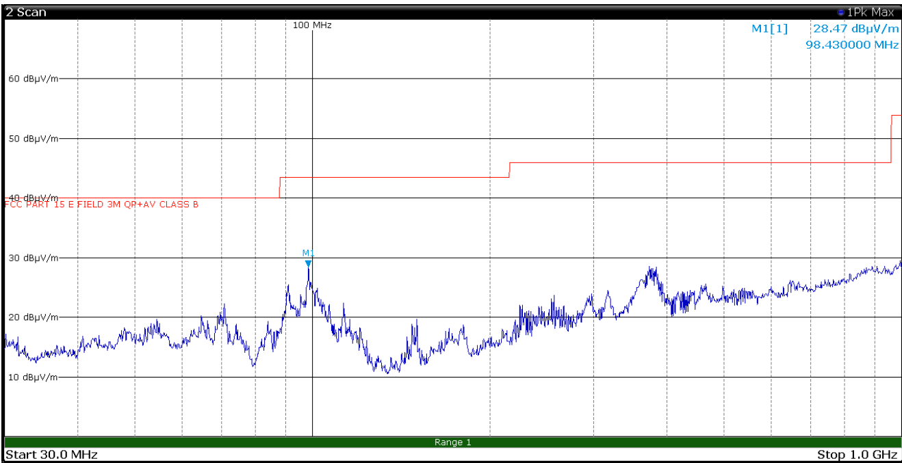
Figure 8.1-17: Radiated spurious emissions, LTE Tx at 1883 MHz, WIFI Tx at 2412 MHz – antenna in horizontal polarization – EUT in configuration 1
