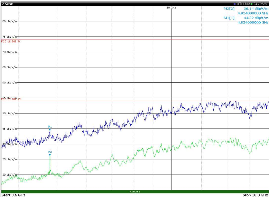
Figure 8.1-38: Radiated spurious emissions, LTE Tx at 782 MHz, WIFI Tx at 2412 MHz – antenna in vertical polarization – EUT in configuration 2
