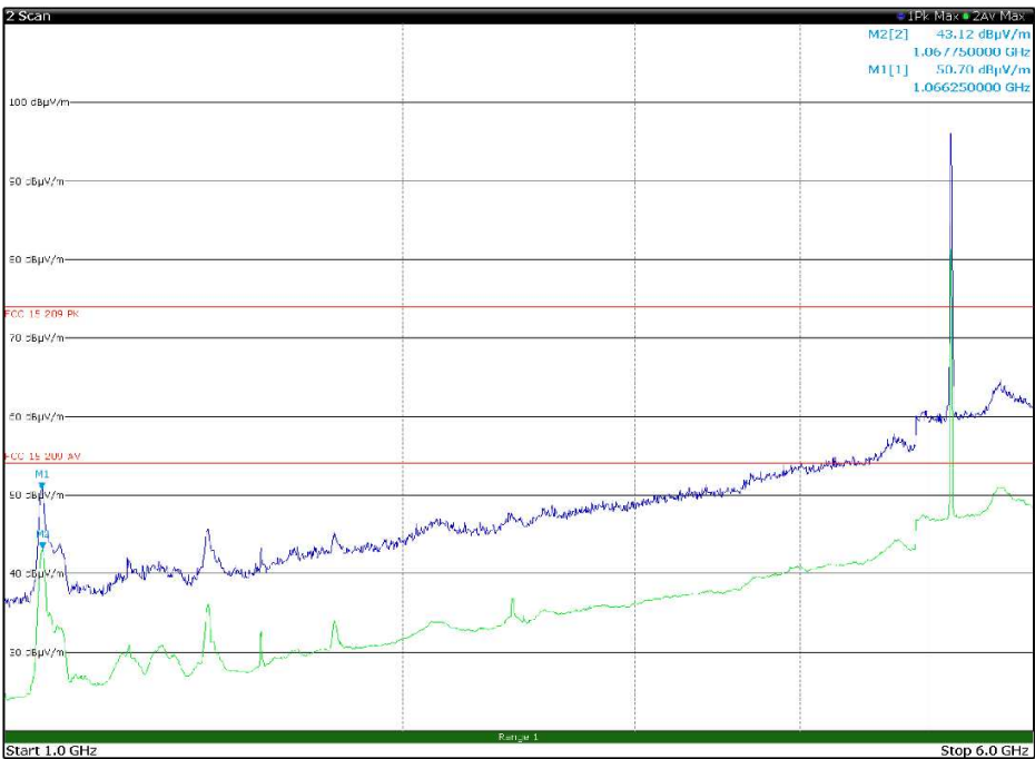
Figure 8.1-11: Radiated spurious emissions, LTE Tx at 782 MHz, WIFI Tx at 5200 MHz – antenna in horizontal polarization – EUT in configuration 1
