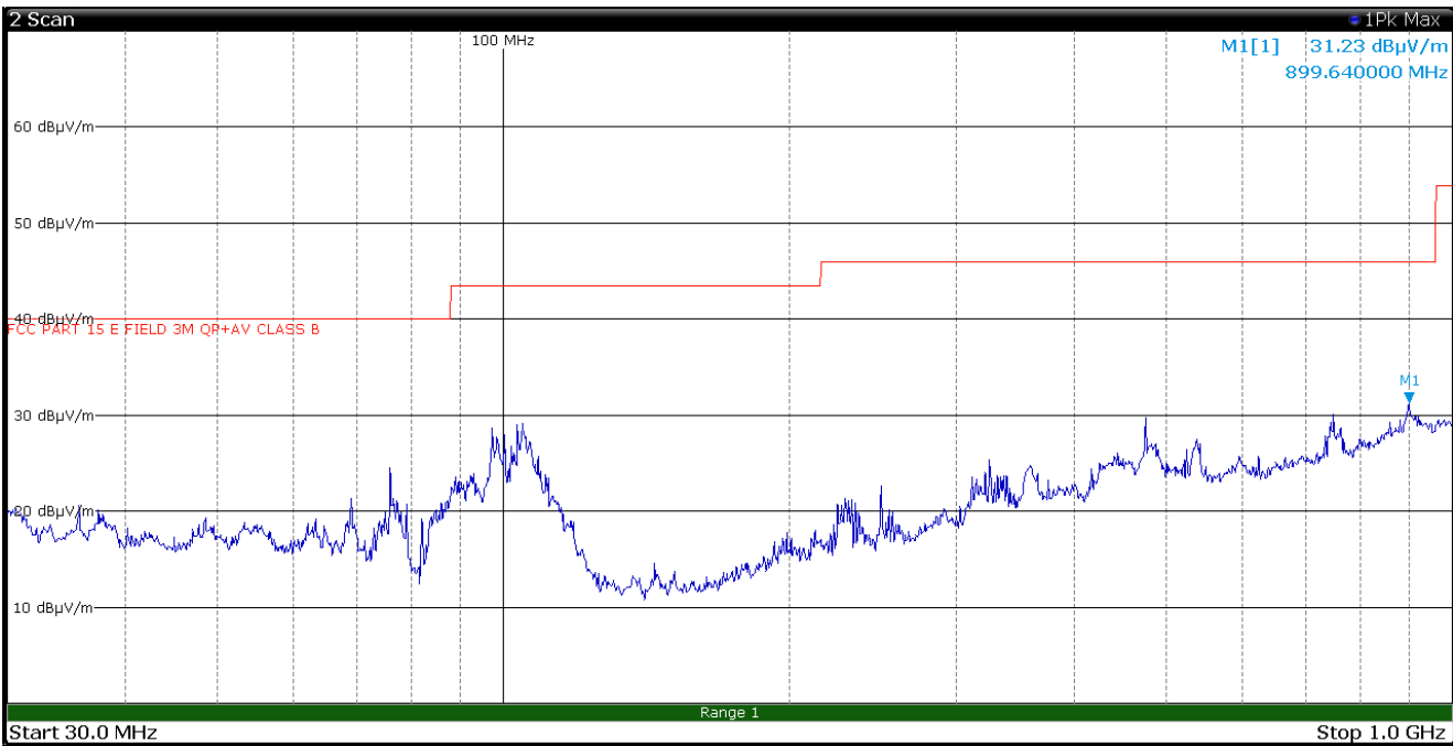
Figure 8.1-49: Radiated spurious emissions, LTE Tx at 1883 MHz, WIFI Tx at 2412 MHz – antenna in horizontal polarization – EUT in configuration 2
