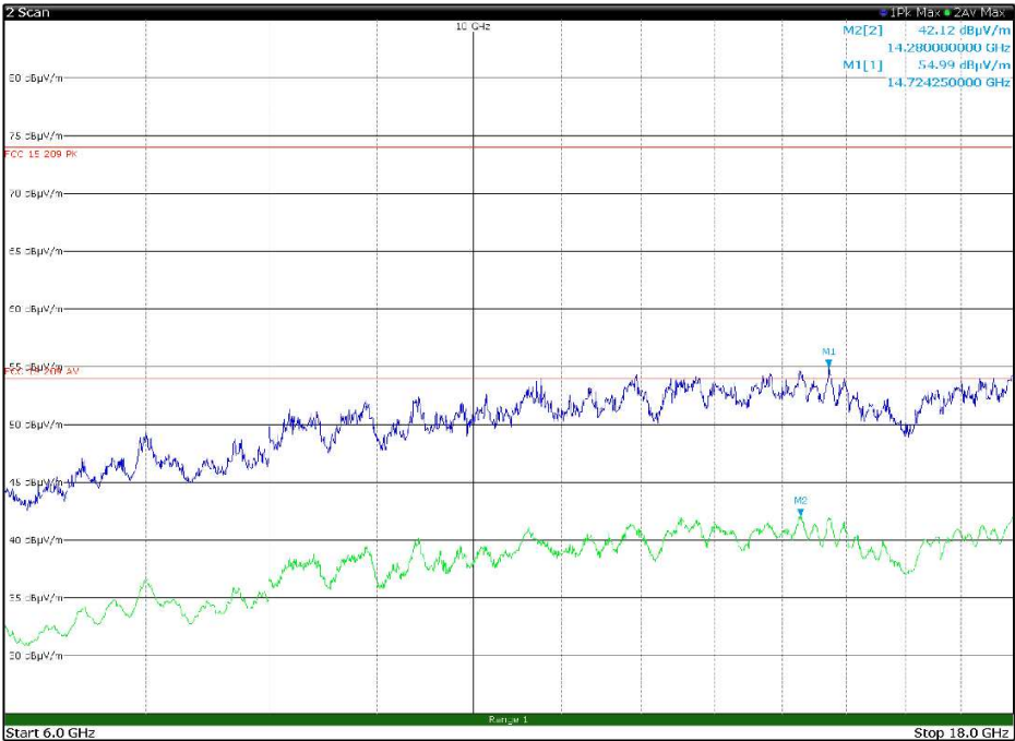
Figure 8.1-53: Radiated spurious emissions, LTE Tx at 1883 MHz, WIFI Tx at 2412 MHz – antenna in horizontal polarization – EUT in configuration 2
