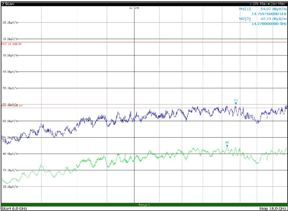
Figure 8.1-54: Radiated spurious emissions, LTE Tx at 1883 MHz, WIFI Tx at 2412 MHz – antenna in vertical polarization – EUT in configuration 2
