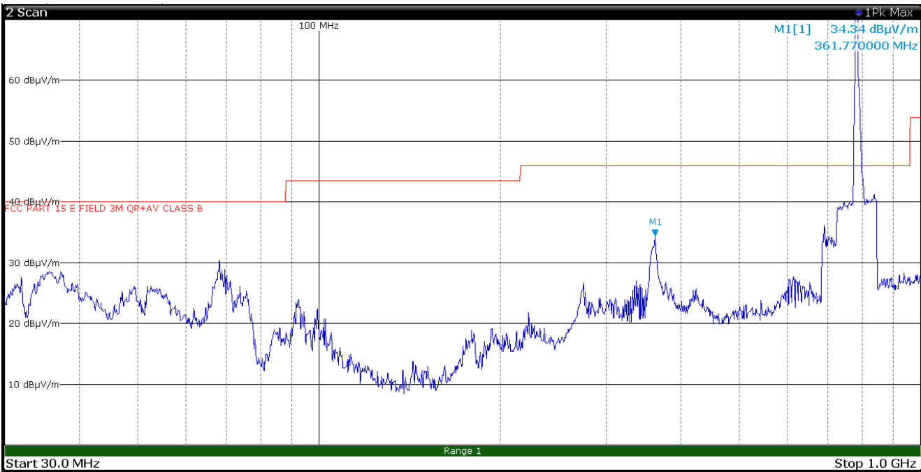
Figure 8.1-42: Radiated spurious emissions, LTE Tx at 782 MHz, WIFI Tx at 5200 MHz – antenna in vertical polarization – EUT in configuration 2
