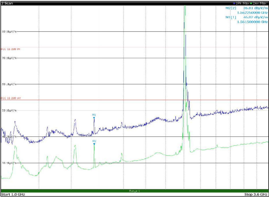
Figure 8.1-68: Radiated spurious emissions, LTE Tx at 782 MHz, WIFI Tx at 2412 MHz – antenna in vertical polarization – EUT in configuration 1
