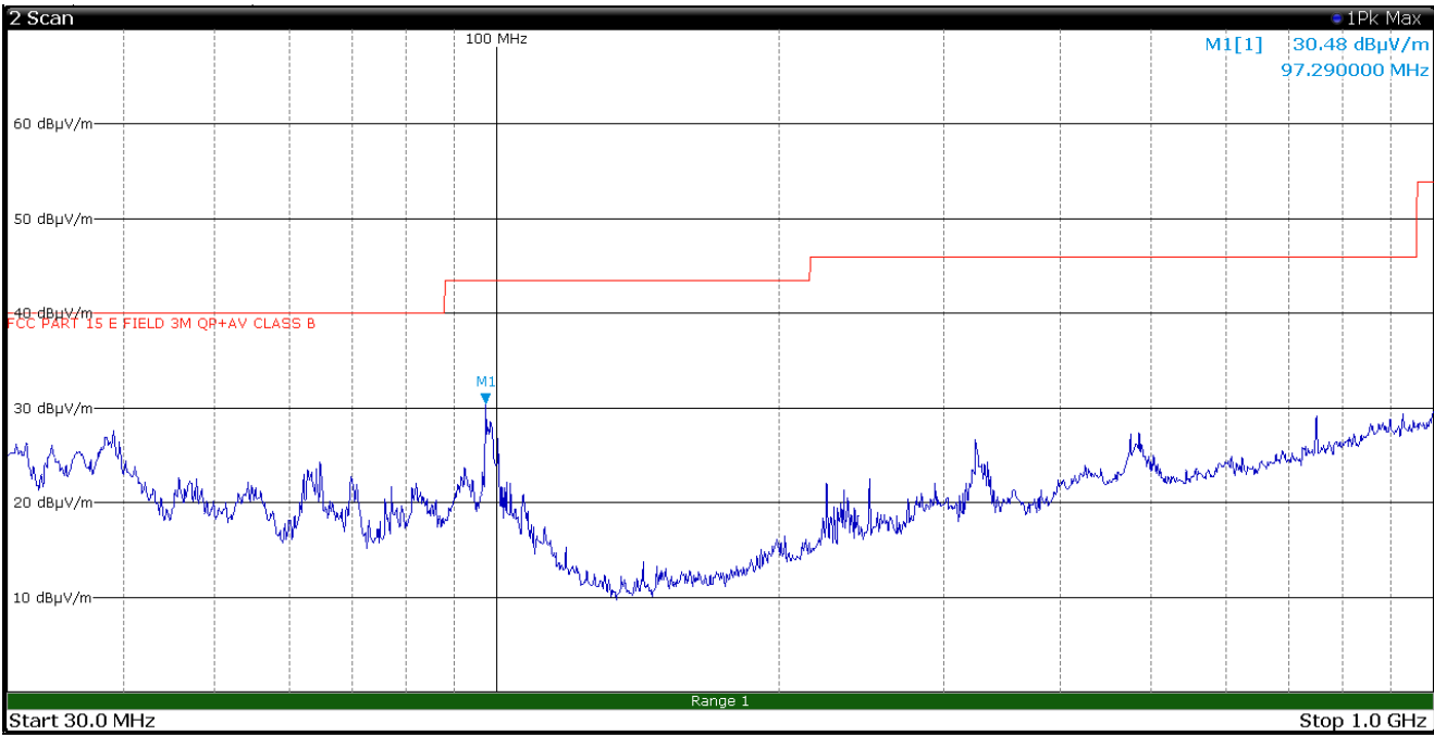
Figure 8.1-50: Radiated spurious emissions, LTE Tx at 1883 MHz, WIFI Tx at 2412 MHz – antenna in vertical polarization – EUT in configuration 2
