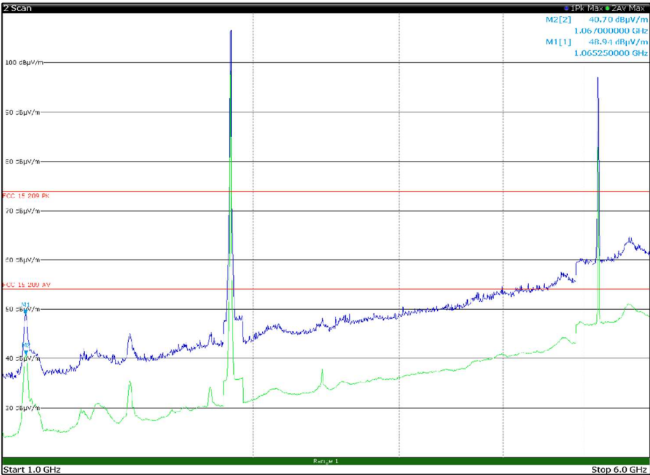
Figure 8.1-59: Radiated spurious emissions, LTE Tx at 1883 MHz, WIFI Tx at 5200 MHz – antenna in horizontal polarization – EUT in configuration 2
