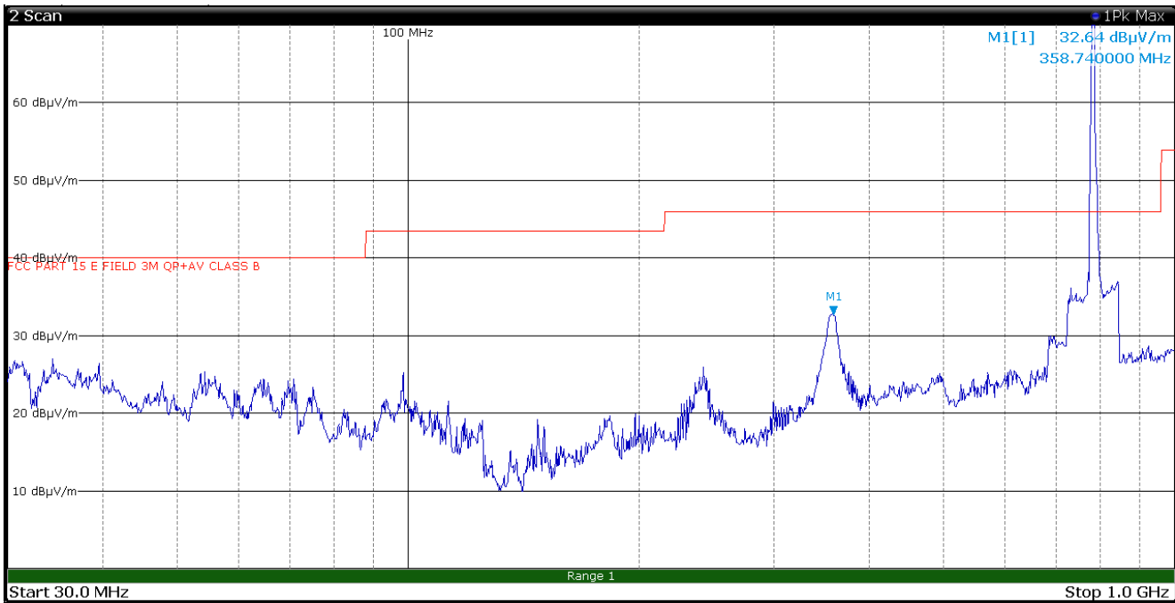
Figure 8.1-66: Radiated spurious emissions, LTE Tx at 782 MHz, WIFI Tx at 2412 MHz – antenna in vertical polarization – EUT in configuration 1
