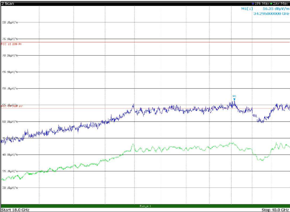
Figure 8.1-55: Radiated spurious emissions, LTE Tx at 1883 MHz, WIFI Tx at 2412 MHz – antenna in horizontal polarization – EUT in configuration 2
