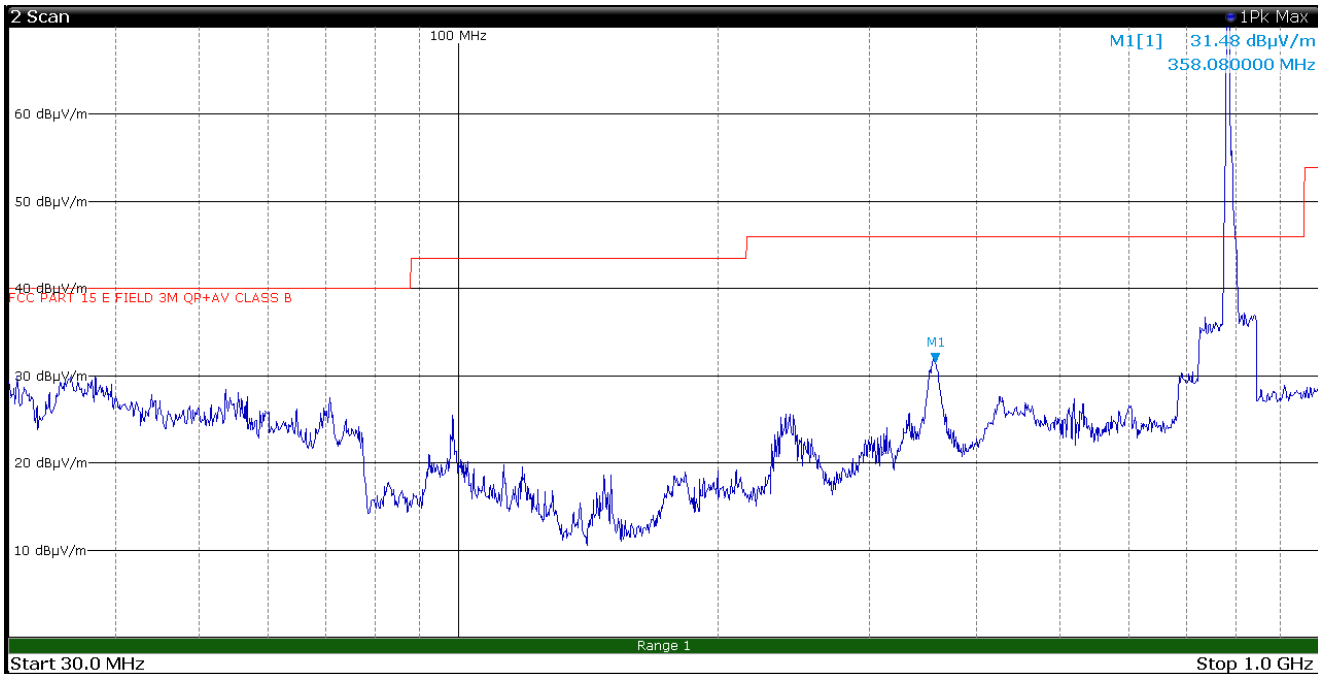
Figure 8.1-2: Radiated spurious emissions, LTE Tx at 782 MHz, WIFI Tx at 2412 MHz – antenna in vertical polarization – EUT in configuration 1
