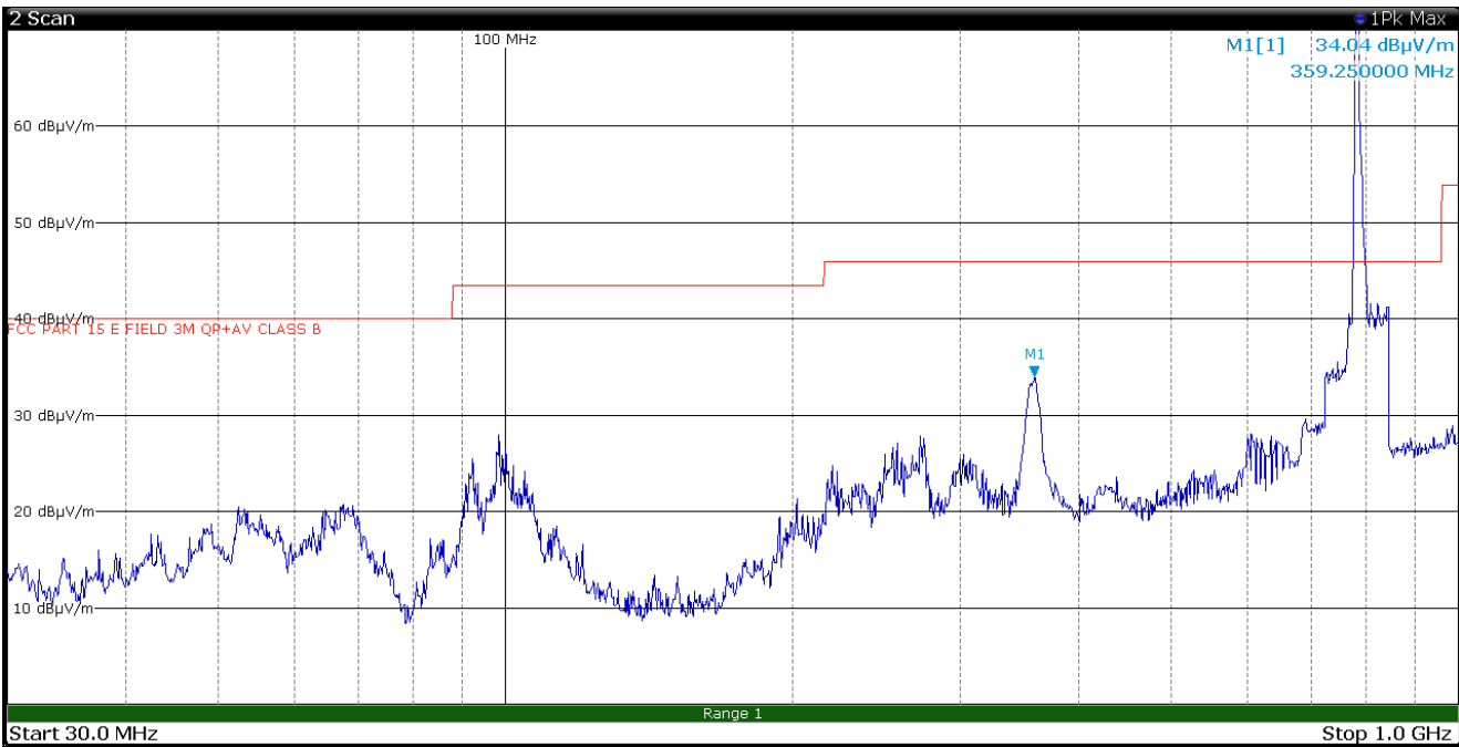
Figure 8.1-41: Radiated spurious emissions, LTE Tx at 782 MHz, WIFI Tx at 5200 MHz – antenna in horizontal polarization – EUT in configuration 2
