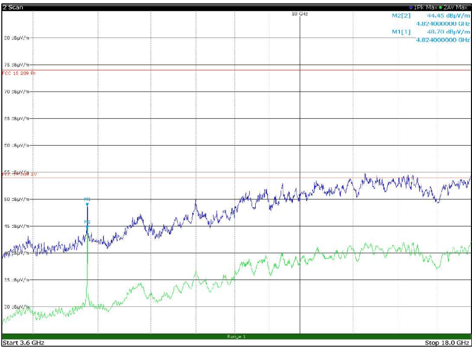
Figure 8.1-21: Radiated spurious emissions, LTE Tx at 1883 MHz, WIFI Tx at 2412 MHz – antenna in horizontal polarization – EUT in configuration 1
