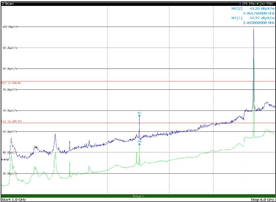
Figure 8.1-12: Radiated spurious emissions, LTE Tx at 782 MHz, WIFI Tx at 5200 MHz – antenna in vertical polarization – EUT in configuration 1
