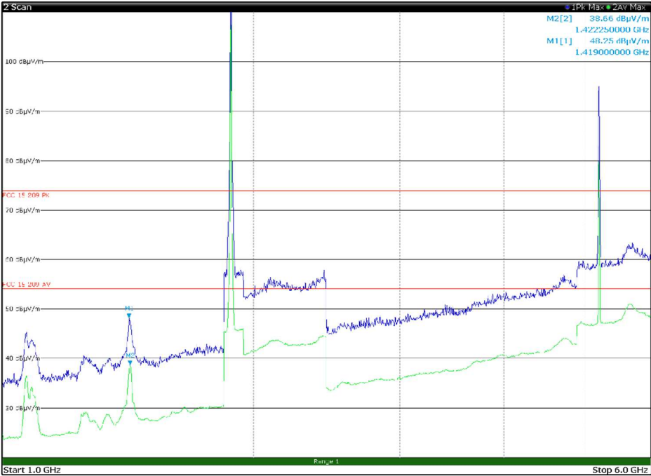
Figure 8.1-60: Radiated spurious emissions, LTE Tx at 1883 MHz, WIFI Tx at 5200 MHz – antenna in vertical polarization – EUT in configuration 2
