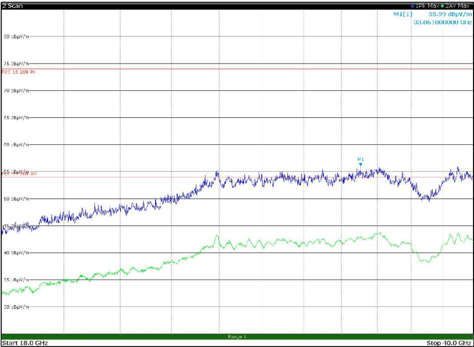
Figure 8.1-40: Radiated spurious emissions, LTE Tx at 782 MHz, WIFI Tx at 2412 MHz – antenna in vertical polarization – EUT in configuration 2
