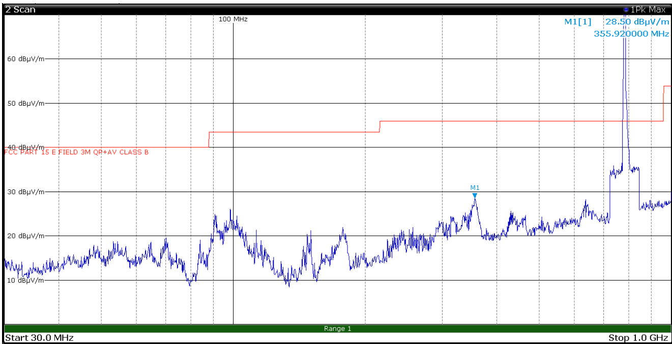
Figure 8.1-9: Radiated spurious emissions, LTE Tx at 782 MHz, WIFI Tx at 5200 MHz – antenna in horizontal polarization – EUT in configuration 1
