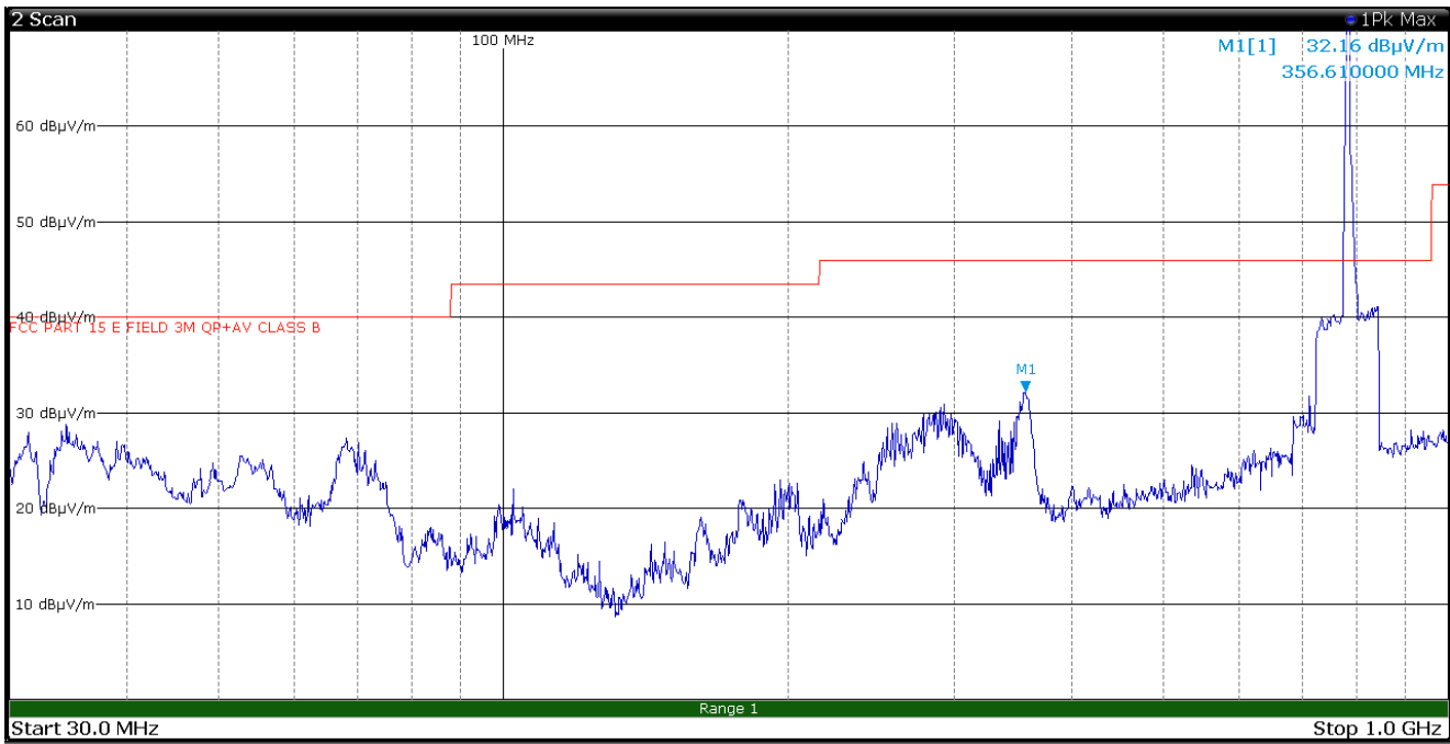
Figure 8.1-34: Radiated spurious emissions, LTE Tx at 782 MHz, WIFI Tx at 2412 MHz – antenna in vertical polarization – EUT in configuration 2
