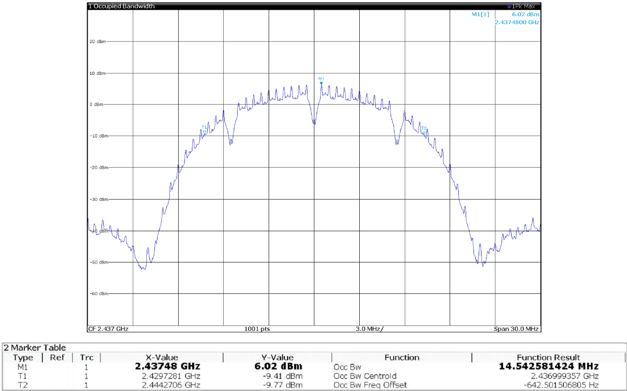
Figure 8.5-5: 99% bandwidth on 802.11b, channel MID
