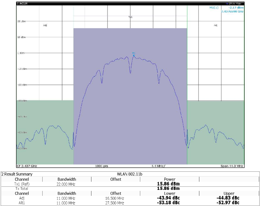
Figure 8.6-2: Output power of WIFI 802.11b, channel MID
