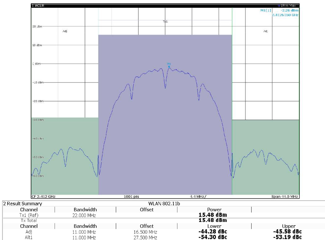
Figure 8.6-1: Output power of WIFI 802.11b, channel LOW
