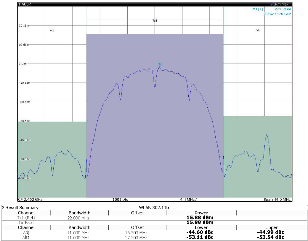
Figure 8.6-3: Output power of WIFI 802.11b, channel HIGH
