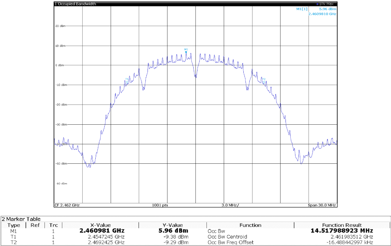
Figure 8.5-6: 99% bandwidth on 802.11b, channel HIGH
