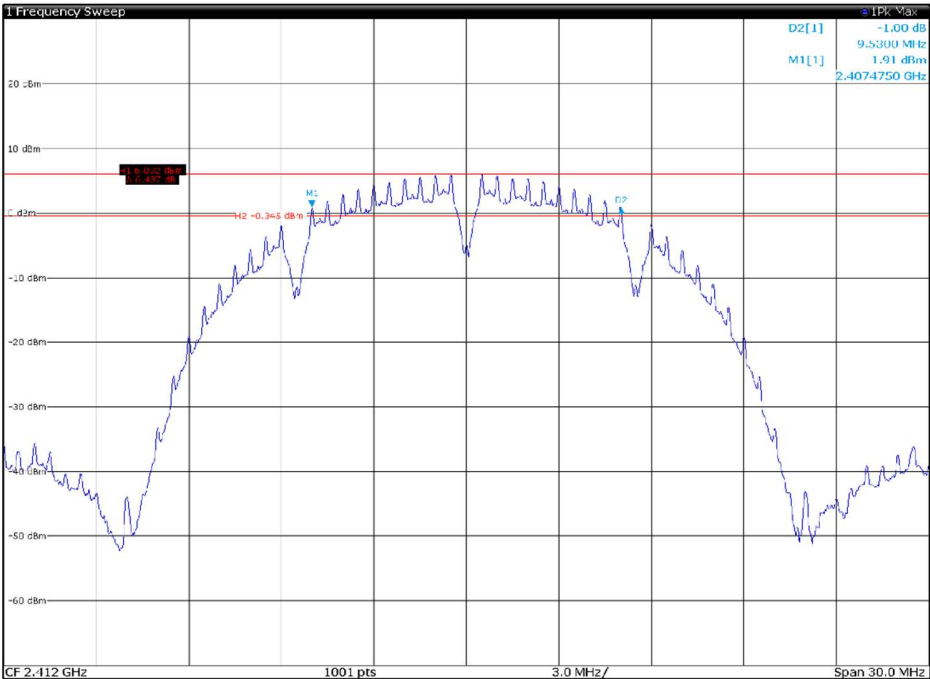
Figure 8.5-1: 6 dB bandwidth on 802.11b, channel LOW
