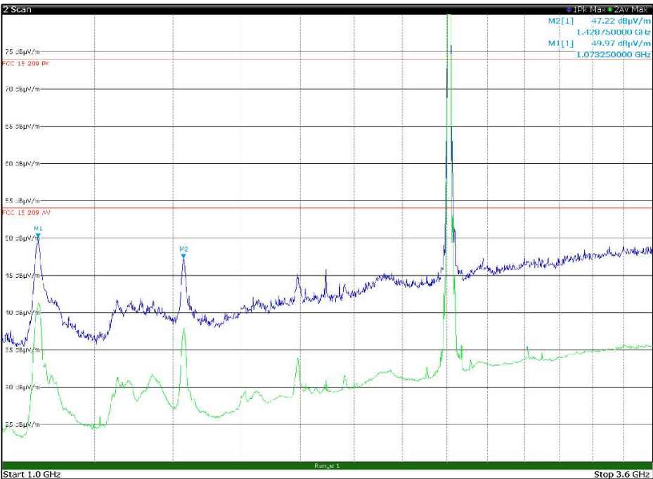
Figure 8.7-8: Radiated spurious emissions 1 to 3.6 GHz, Low channel with antenna in vertical polarization Limit exceeded by the carrier
