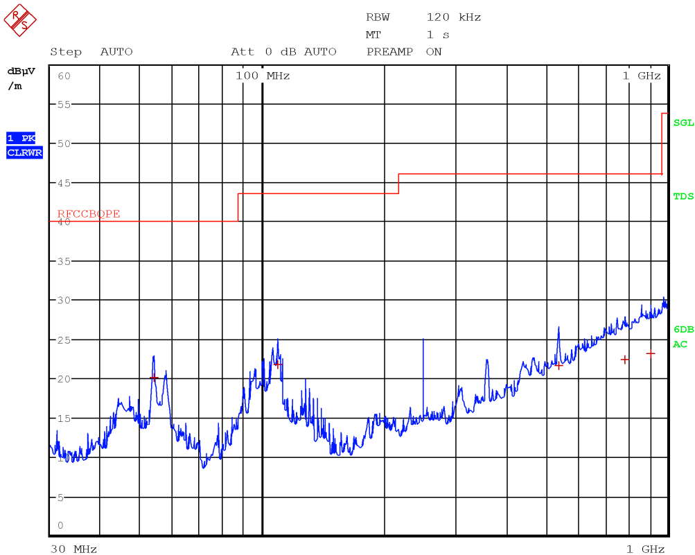
Figure 8.7-51: Radiated spurious emissions 30 to 1000 MHz, Mid channel with antenna in horizontal polarization
