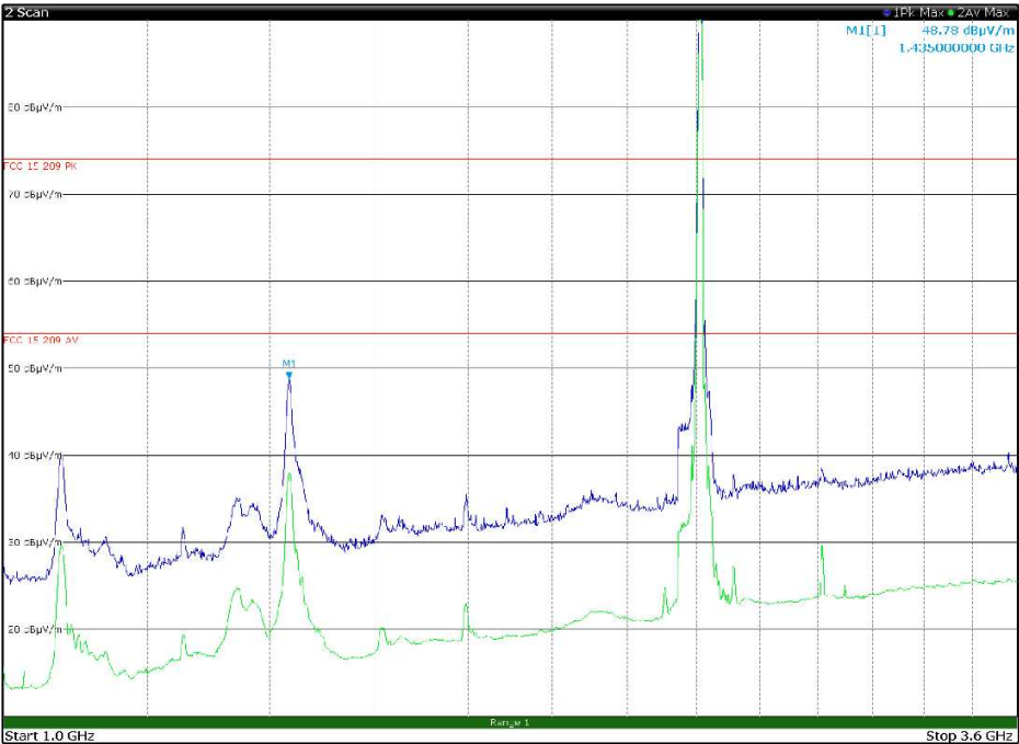
Figure 8.7-55: Radiated spurious emissions 1 to 3.6 GHz, Low channel with antenna in horizontal polarization Limit exceeded by the carrier
