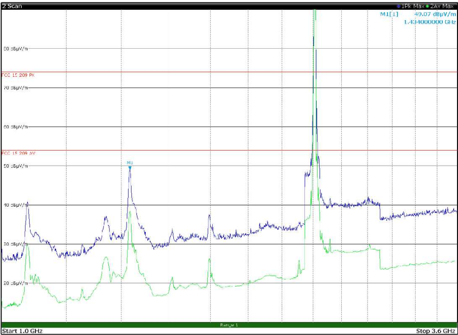
Figure 8.7-56: Radiated spurious emissions 1 to 3.6 GHz, Low channel with antenna in vertical polarization Limit exceeded by the carrier
