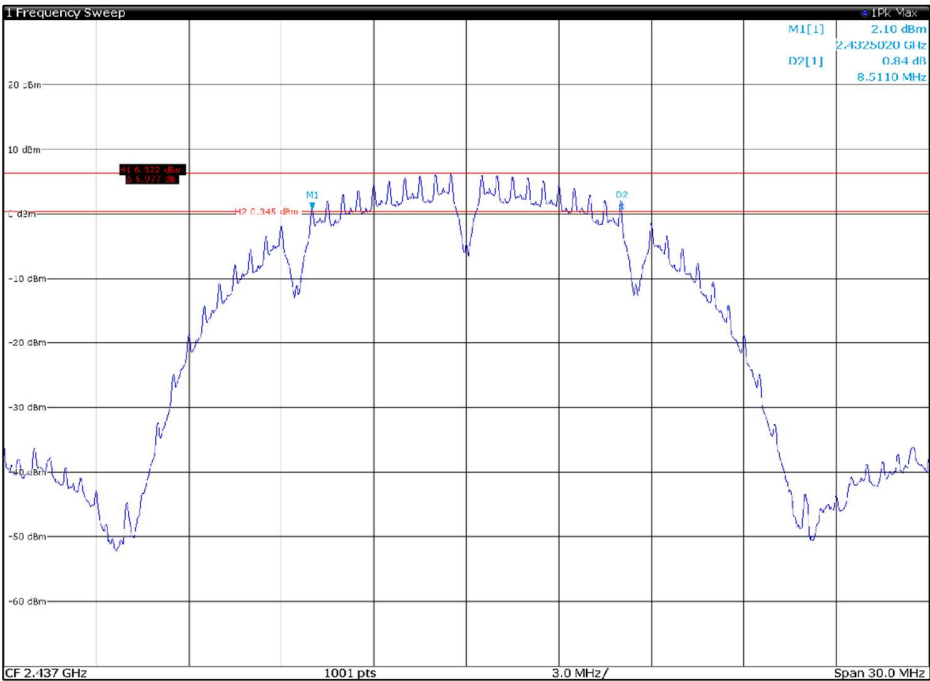
Figure 8.5-2: 6 dB bandwidth on 802.11b, channel MID
