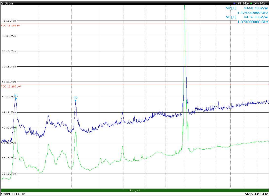
Figure 8.7-7: Radiated spurious emissions 1 to 3.6 GHz, Low channel with antenna in horizontal polarization Limit exceeded by the carrier
