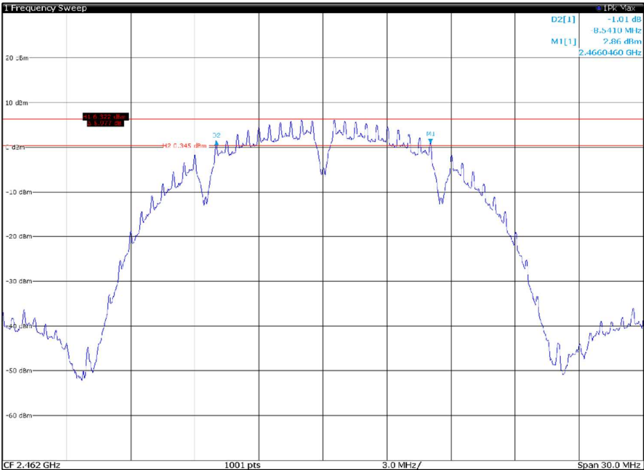
Figure 8.5-3: 6 dB bandwidth on 802.11b, channel HIGH
