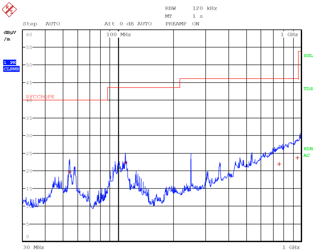
Figure 8.4-51: Radiated spurious emissions 30 to 1000 MHz, mid channel with antenna in horizontal polarization
