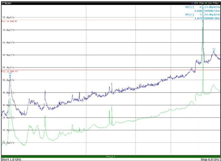
Figure 8.4-10: Radiated spurious emissions 1 to 6 GHz, mid channel with antenna in vertical polarization Limit exceeded by the carrier
