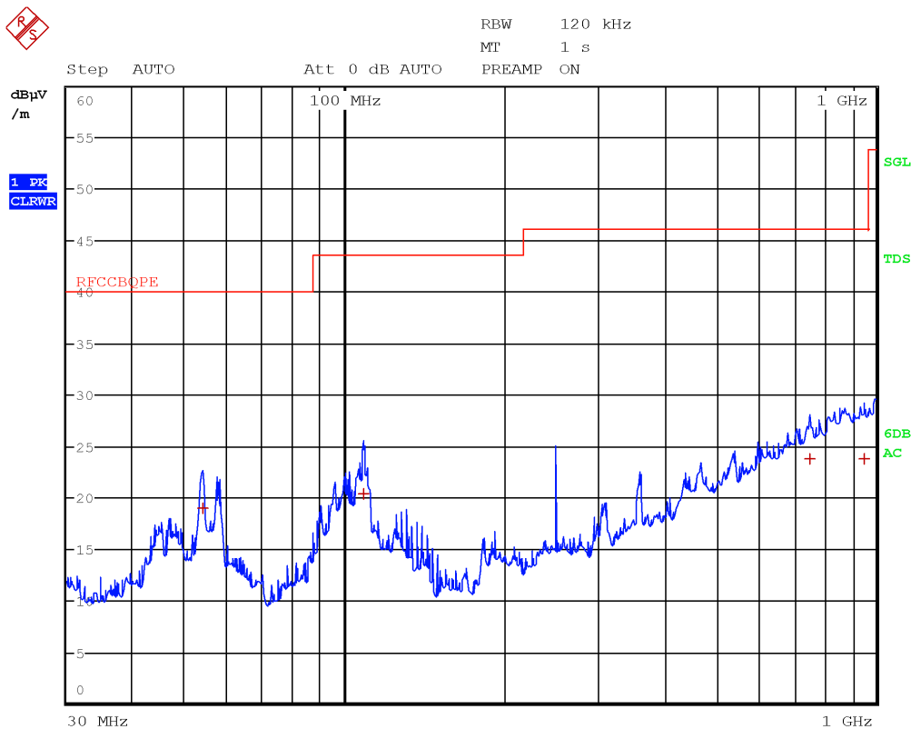
Figure 8.4-53: Radiated spurious emissions 30 to 1000 MHz, high channel with antenna in horizontal polarization
