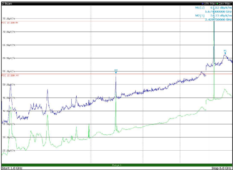
Figure 8.4-9: Radiated spurious emissions 1 to 6 GHz, mid channel with antenna in horizontal polarization Limit exceeded by the carrier
