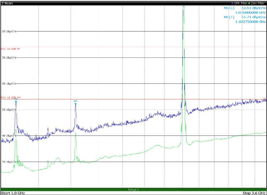
Figure 8.7-79: Radiated spurious emissions 1 to 3.6 GHz, Low channel with antenna in horizontal polarization Limit exceeded by the carrier
