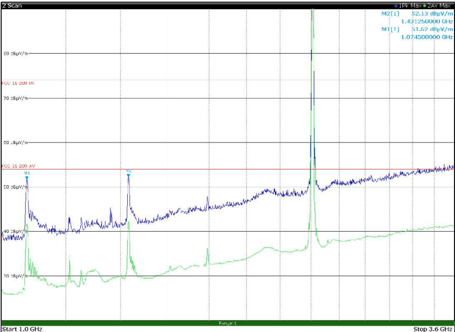
Figure 8.7-80: Radiated spurious emissions 1 to 3.6 GHz, Low channel with antenna in vertical polarization Limit exceeded by the carrier
