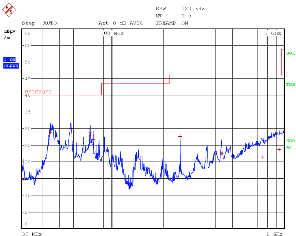
Figure 8.7-76: Radiated spurious emissions 30 to 1000 MHz, Mid channel with antenna in vertical polarization
