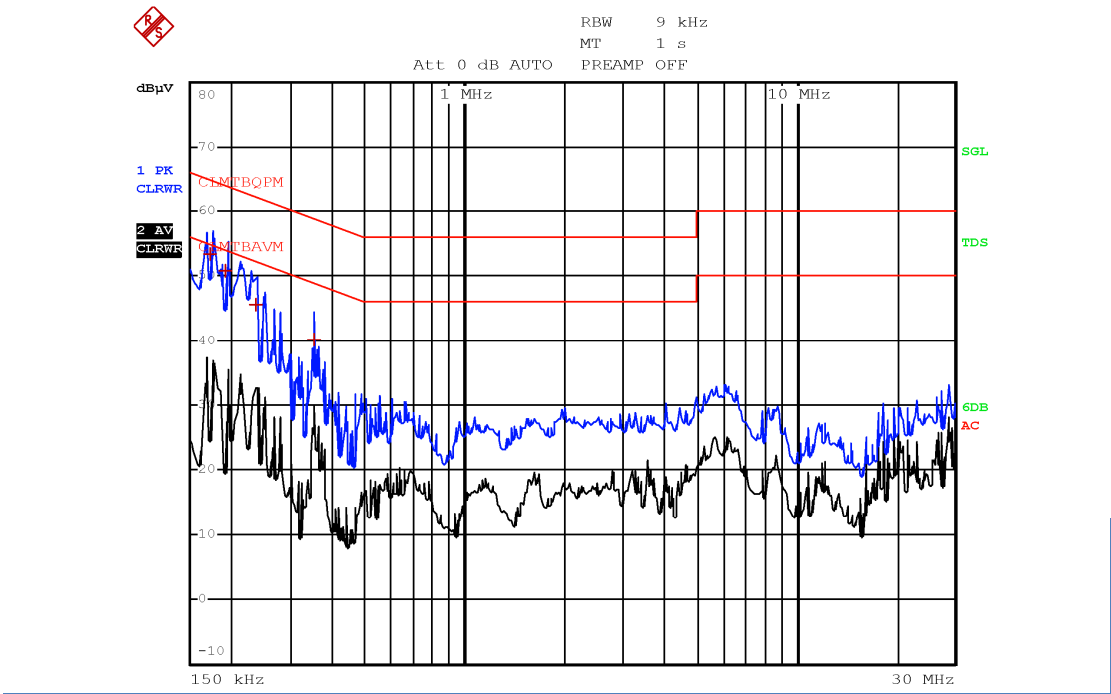
Plot 8.5-2: Conducted emissions on neutral line
