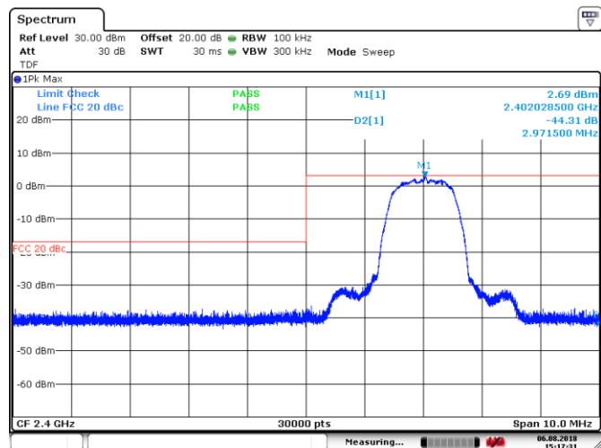
Figure 8.7-3: Conducted spurious emission at band edge outside restricted band, low channel, \pi/4 -DWPSK
