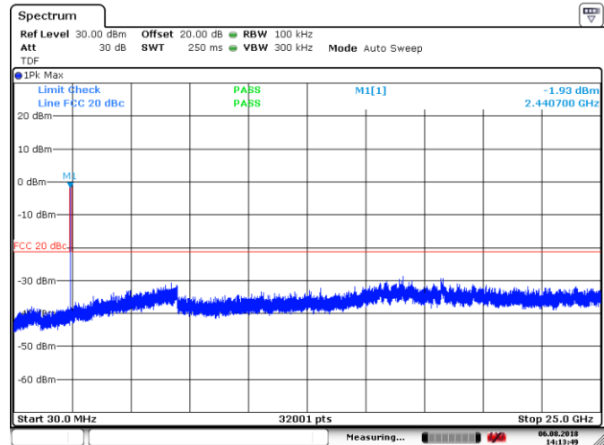
Figure 8.7-10: Conducted spurious emissions outside restricted band, Mid channel, GFSK
