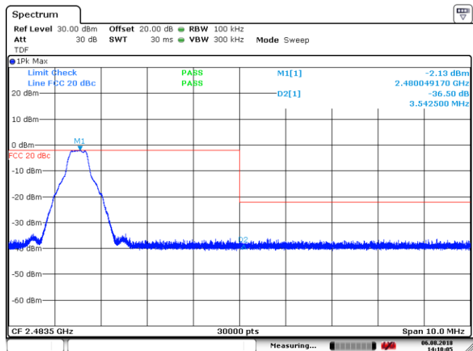
Figure 8.7-2: Conducted spurious emissions at band edge outside restricted band, High channel, GFSK
