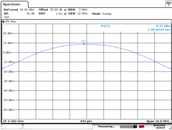
Figure 8.6-4: Output power of BLE, sample plot
