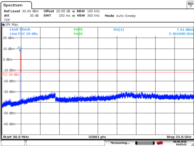
Figure 8.7-18: Conducted spurious emissions outside restricted band, Low channel, BLE
