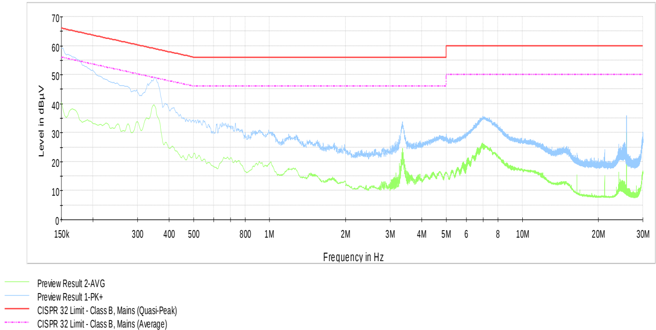
Plot 8.4-1: Conducted emissions on phase line
