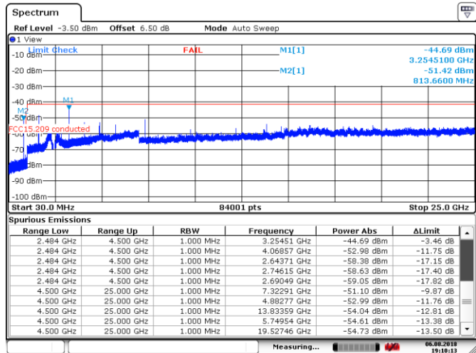
Figure 8.7-28: Conducted spurious emissions within restricted band, Mid channel, 8-DPSK
