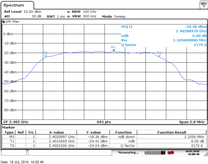
Figure 8.5-3: 6 dB bandwidth of 8-DPSK, sample plot
