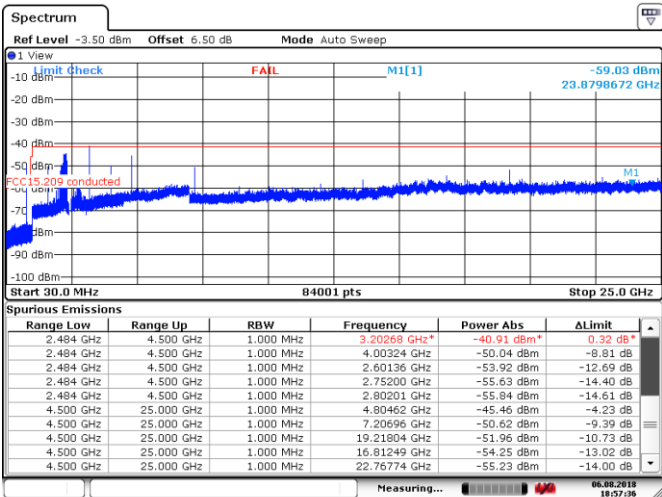
Figure 8.7-30: Conducted spurious emissions within restricted band, Low channel, BLE
