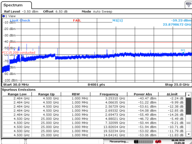
Figure 8.7-31: Conducted spurious emissions within restricted band, Mid channel, BLE
