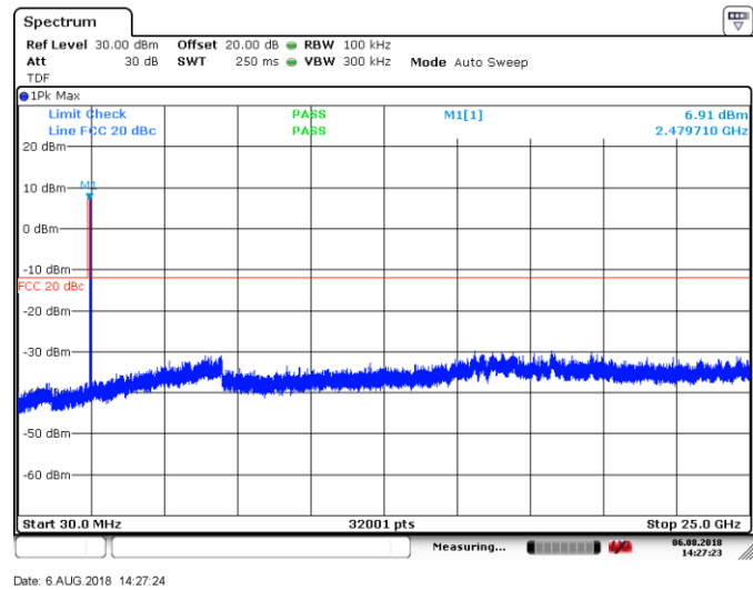
Figure 8.7-20: Conducted spurious emissions outside restricted band, High channel, BLE
