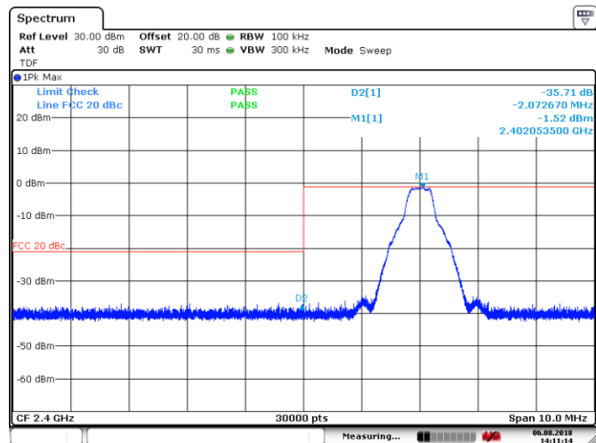
Figure 8.7-1: Conducted spurious emission at band edge outside restricted band, low channel, GFSK
