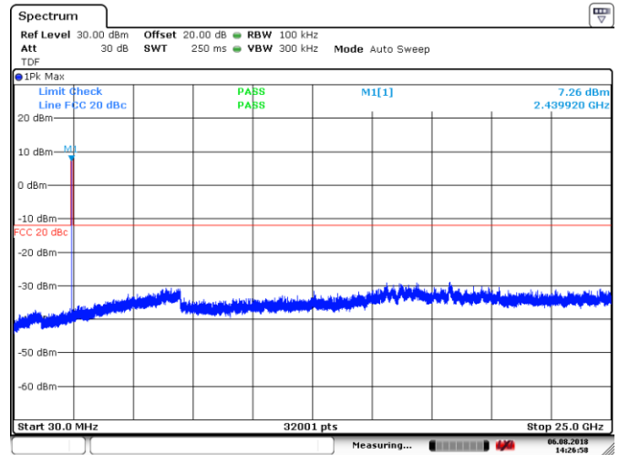
Figure 8.7-19: Conducted spurious emissions outside restricted band, Mid channel, BLE
