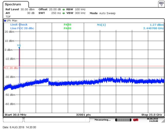
Figure 8.7-13: Conducted spurious emissions outside restricted band, Mid channel, \pi/4 -DWPSK
