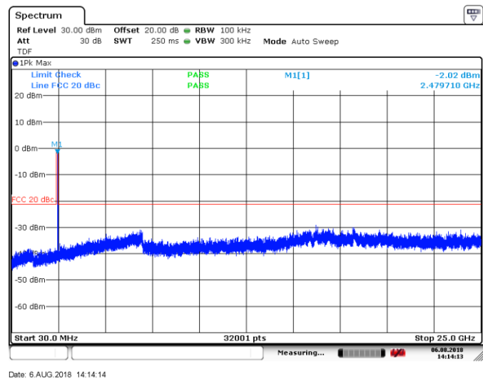
Figure 8.7-11: Conducted spurious emissions outside restricted band, High channel, GFSK
