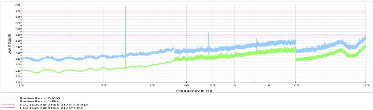
Figure 8.7-33: Cabinet Radiated spurious emissions 1 to 18 GHz, Low channel
