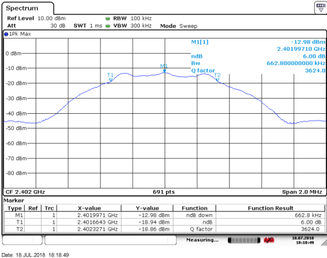
Figure 8.5-4: 6 dB bandwidth of BLE, sample plot
