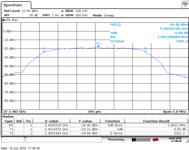
Figure 8.5-2: 6 dB bandwidth of \pi/4 -DWPSK, sample plot
