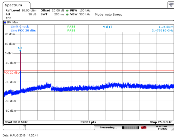
Figure 8.7-14: Conducted spurious emissions outside restricted band, High channel, \pi/4 -DWPSK
