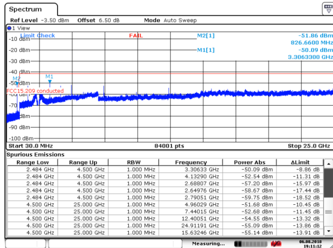
Figure 8.7-29: Conducted spurious emissions within restricted band, High channel, 8-DPSK
