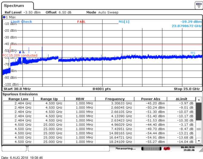
Figure 8.7-32: Conducted spurious emissions within restricted band, High channel, BLE
