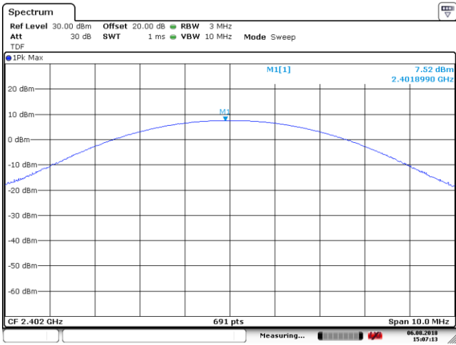
Figure 8.6-2: Output power of \pi/4 -DWPSK, sample plot
