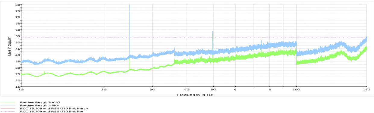
Figure 8.7-35: Cabinet Radiated spurious emissions 1 to 18 GHz, High channel
