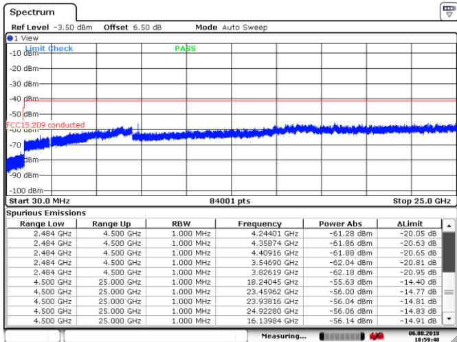
Figure 8.7-22: Conducted spurious emissions within restricted band, Mid channel, GFSK
