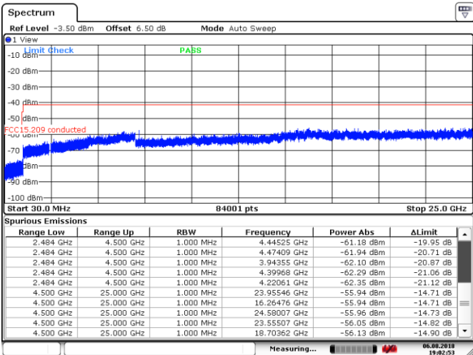
Figure 8.7-21: Conducted spurious emissions within restricted band, Low channel, GFSK
