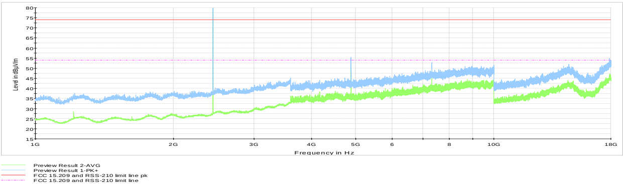
Figure 8.7-34: Cabinet Radiated spurious emissions 1 to 18 GHz, mid channel
