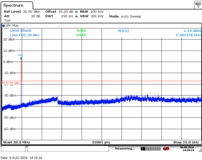
Figure 8.7-12: Conducted spurious emissions outside restricted band, Low channel, \pi/4 -DWPSK
