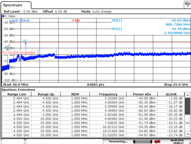
Figure 8.7-27: Conducted spurious emissions within restricted band, Low channel, 8-DPSK
