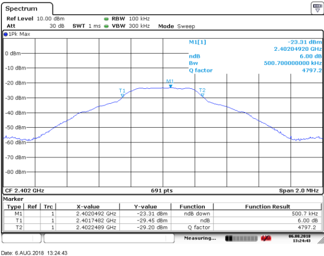
Figure 8.5-1: 6 dB bandwidth of GFSK, sample plot
