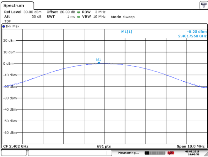
Figure 8.6-1: Output power of GFSK, sample plot
