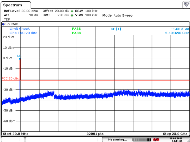
Figure 8.7-9: Conducted spurious emissions outside restricted band, Low channel, GFSK
