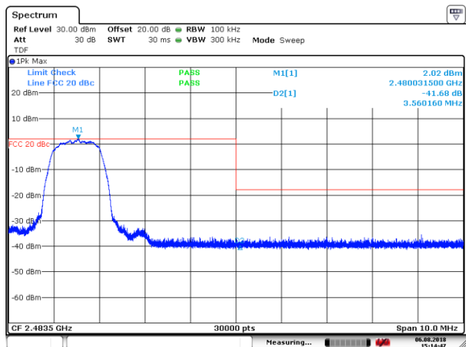
Figure 8.7-4: Conducted spurious emissions at band edge outside restricted band, High channel, \pi/4 -DWPSK
