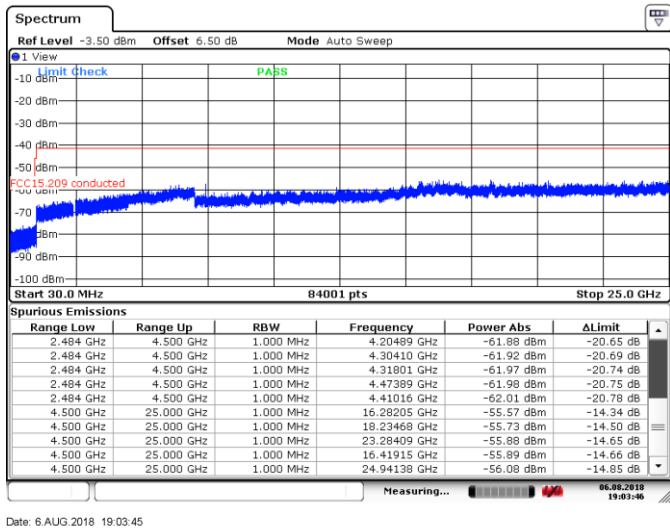
Figure 8.7-23: Conducted spurious emissions within restricted band, High channel, GFSK
