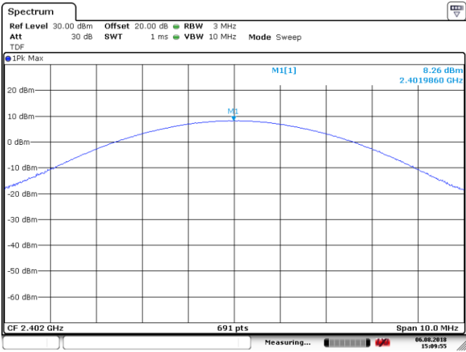
Figure 8.6-3: Output power of 8DPSK, sample plot
