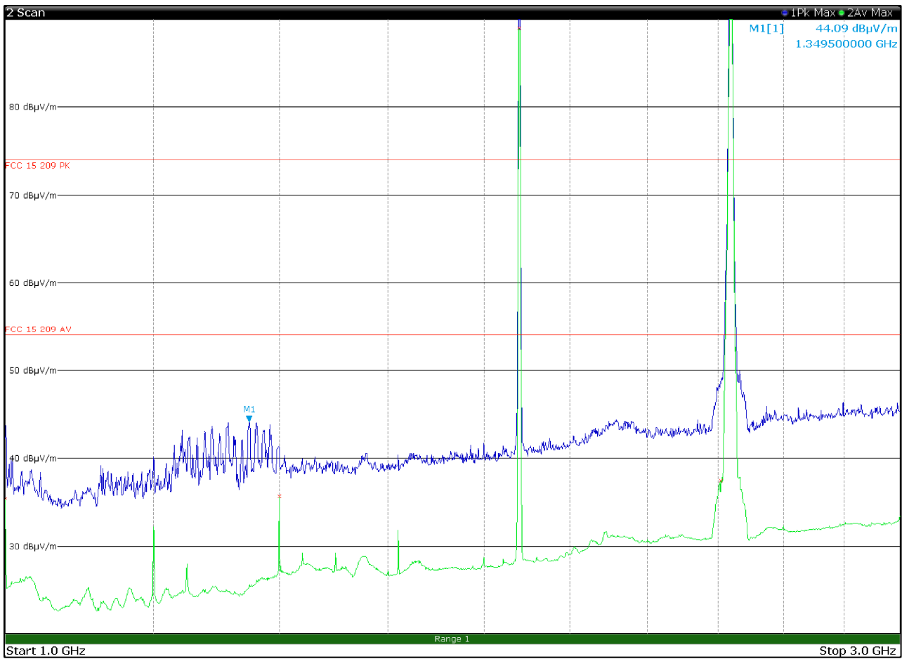
Figure 8.1-4: Radiated spurious emissions with WCDMA at 1880 MHz and WIFI at 2437 MHz – antenna in vertical polarization
