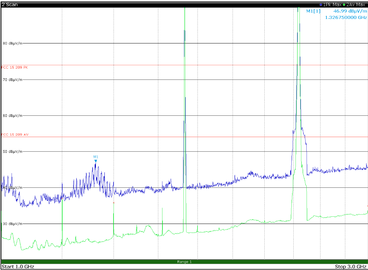
Figure 8.1-13: Radiated spurious emissions with WCDMA at 1732.6 MHz and WIFI at 2437 MHz – antenna in horizontal polarization
