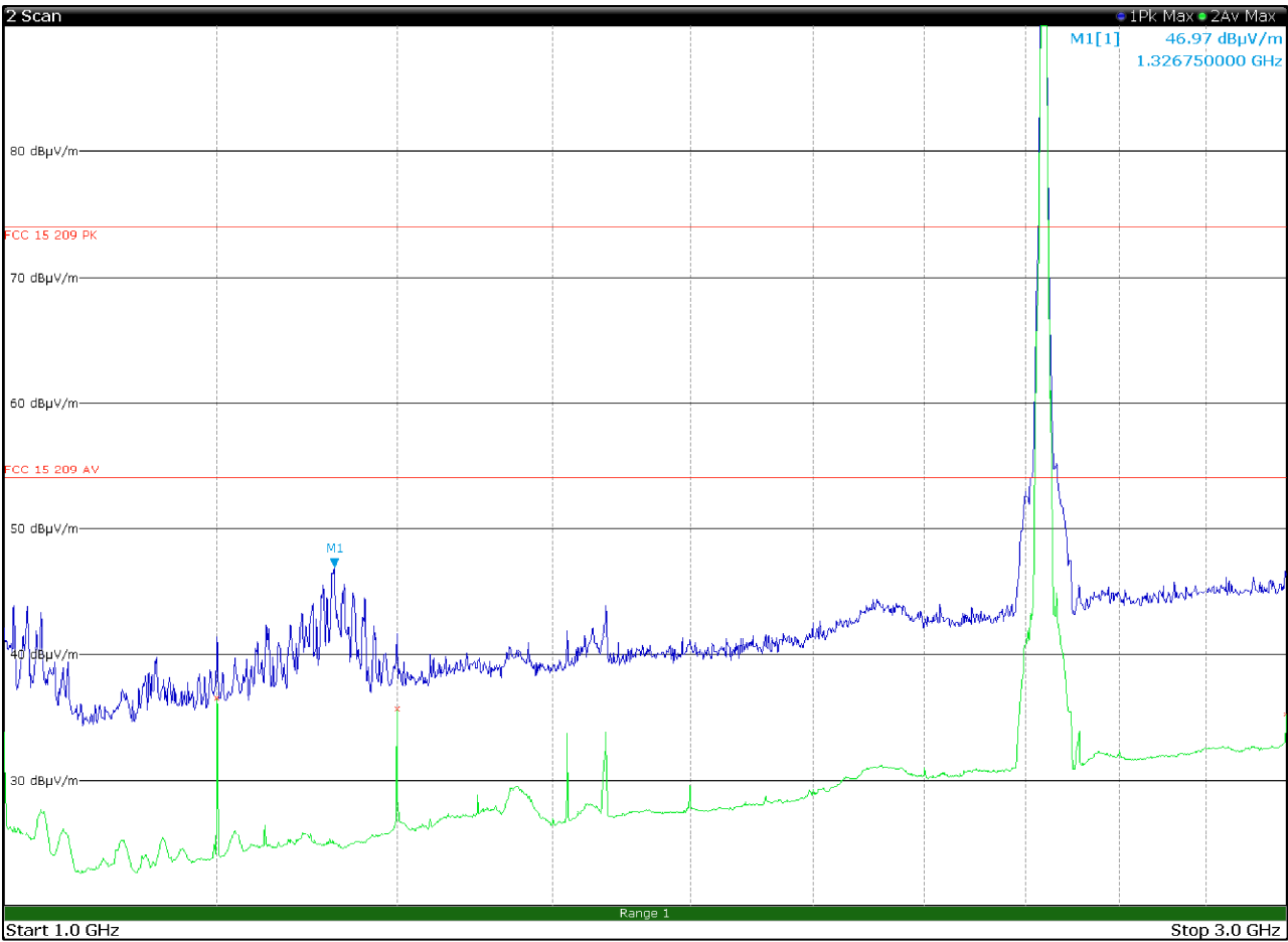
Figure 8.1-23: Radiated spurious emissions with WCDMA at 832.6 MHz and WIFI at 2437 MHz – antenna in horizontal polarization
