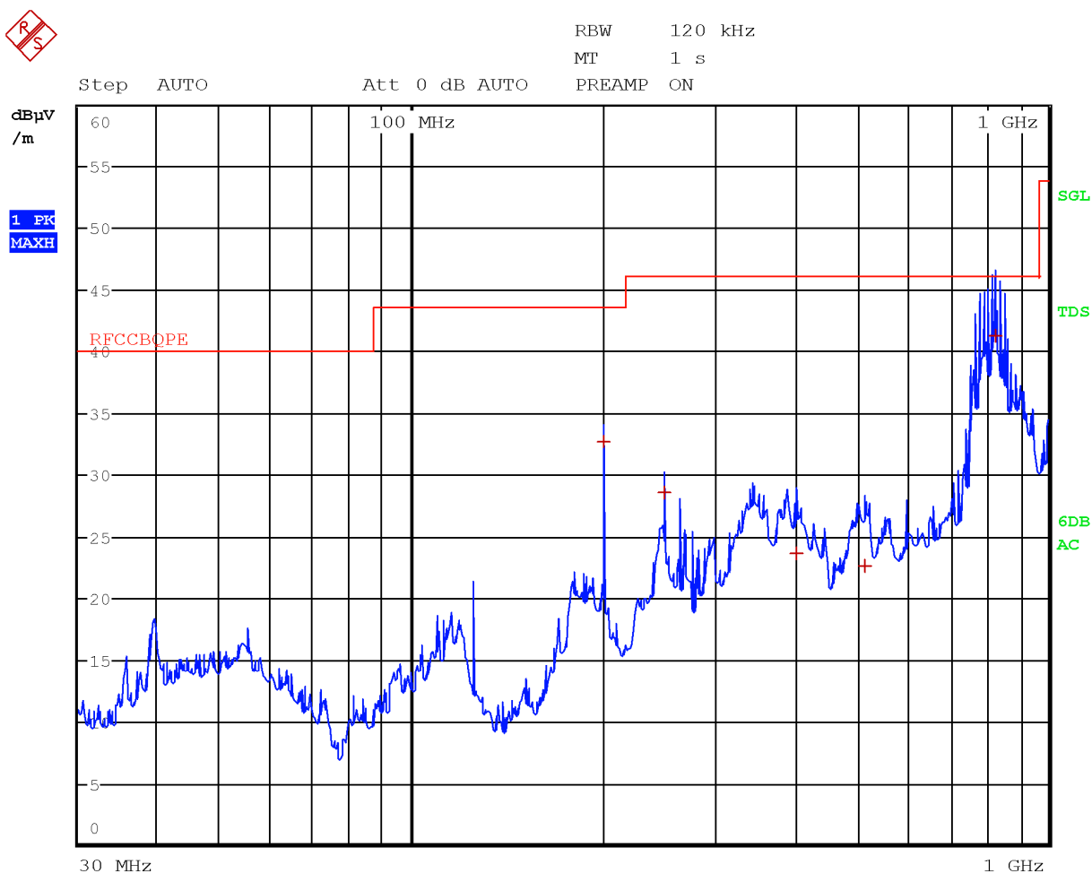
Figure 8.1-31: Radiated spurious emissions with WCDMA at 1880 MHz and WIFI at 5200 MHz – antenna in horizontal polarization
