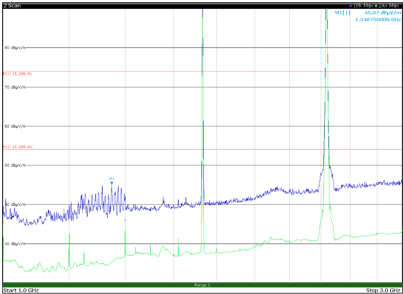
Figure 8.1-14: Radiated spurious emissions with WCDMA at 1732.6 MHz and WIFI at 2437 MHz – antenna in vertical polarization
