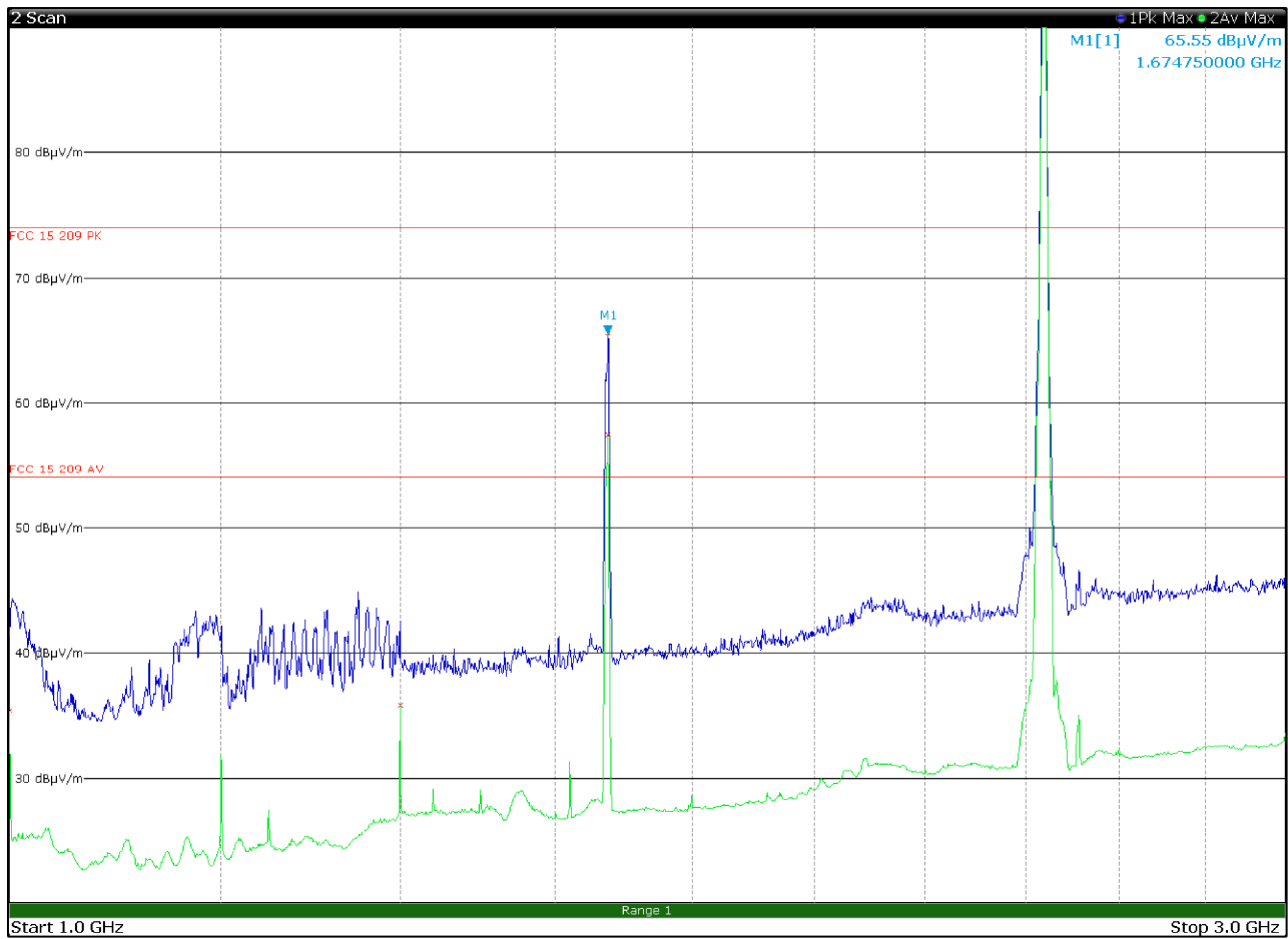
Figure 8.1-24: Radiated spurious emissions with WCDMA at 832.6 MHz and WIFI at 2437 MHz – antenna in vertical polarization
