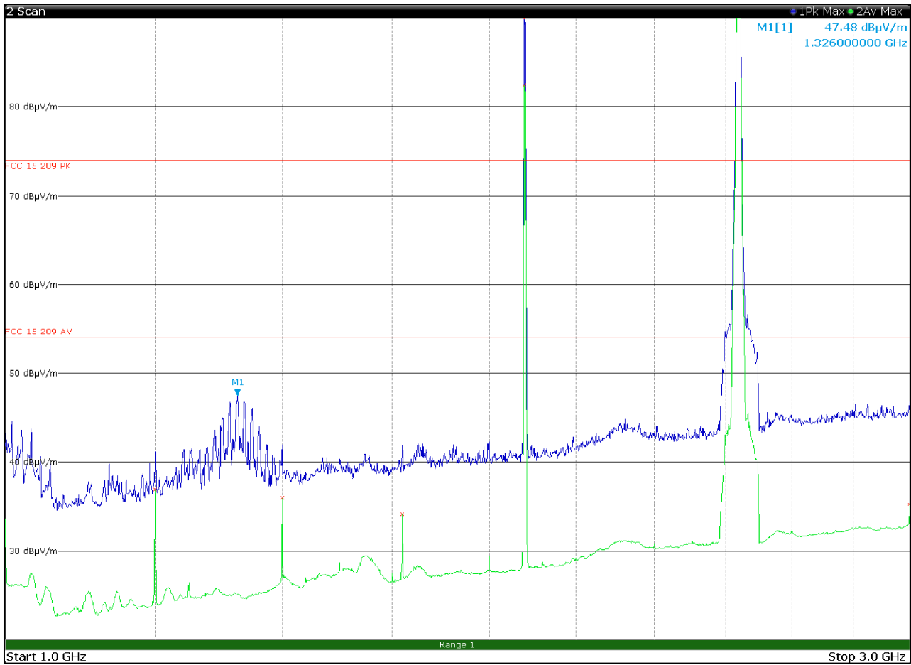
Figure 8.1-3: Radiated spurious emissions with WCDMA at 1880 MHz and WIFI at 2437 MHz – antenna in horizontal polarization
