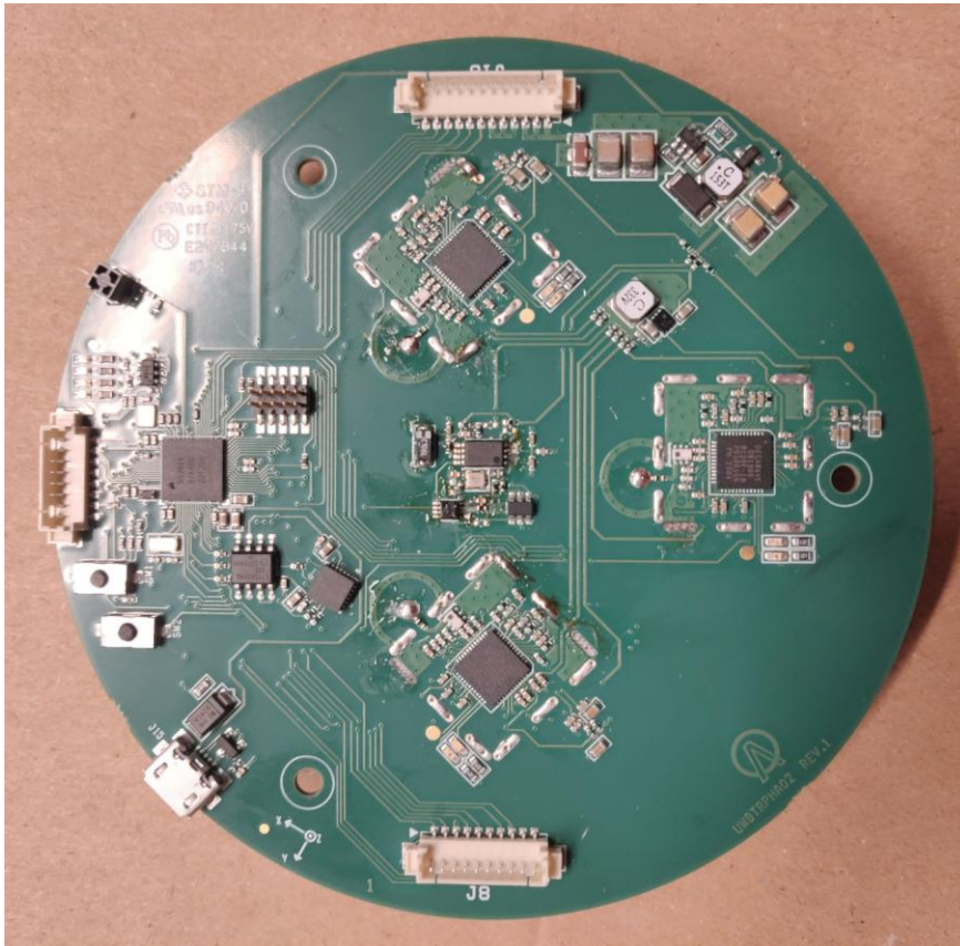
Figura 3. Bottom Side Module without transceivers Shield
