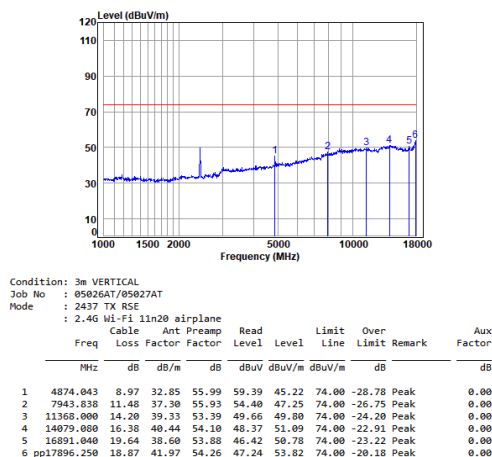
11n_20M_TX_CH_06_Vertical-Peak
