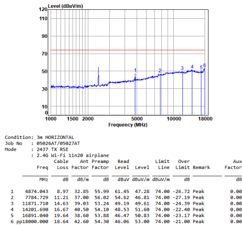
11n_20M_TX_CH_06_Horizontal-Peak
