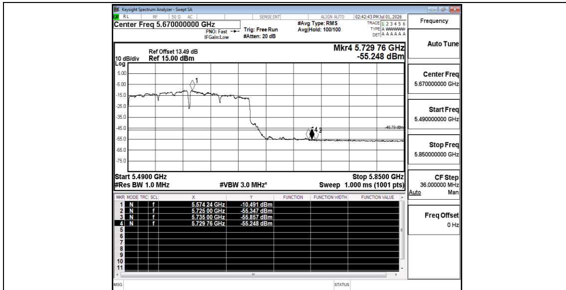
11AC160SISO_Ant1_High_5570_Peak
