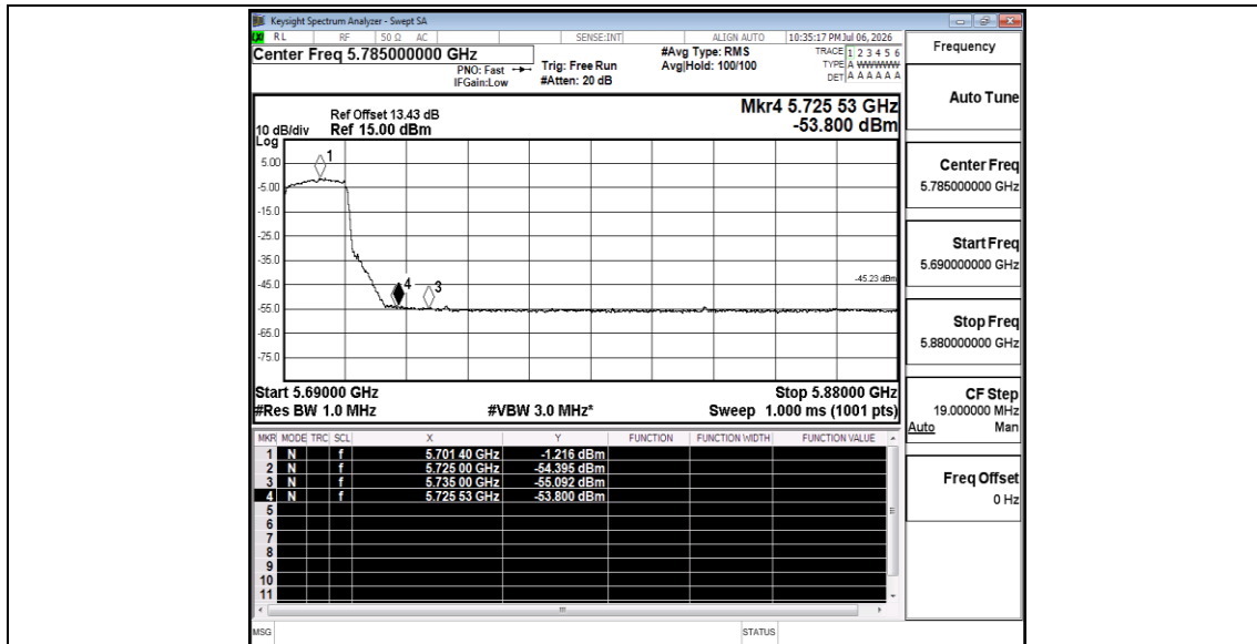
11AX20ISO_Ant3_High_5700_Peak
