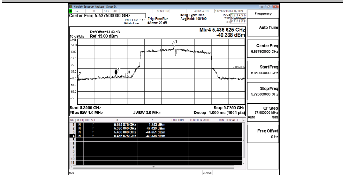
11AX160SISO_Ant3_High_5570_AV
