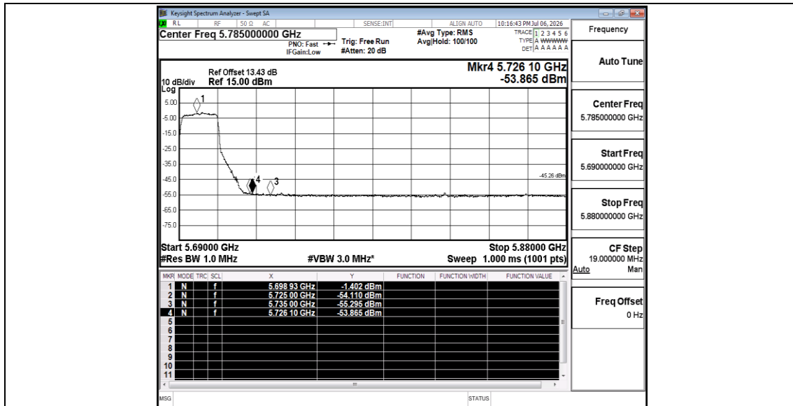
11AC20ISO_Ant3_High_5700_Peak
