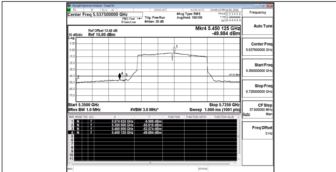
11AX160SISO_Ant3_Low_5570_Peak
