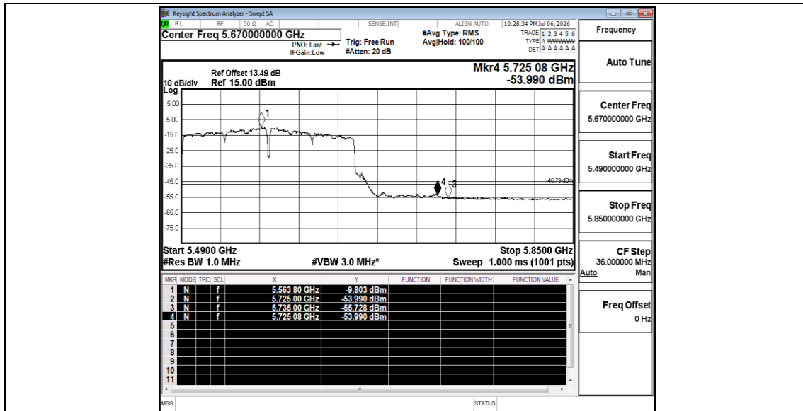
11AC160SISO_Ant3_High_5570_Peak
