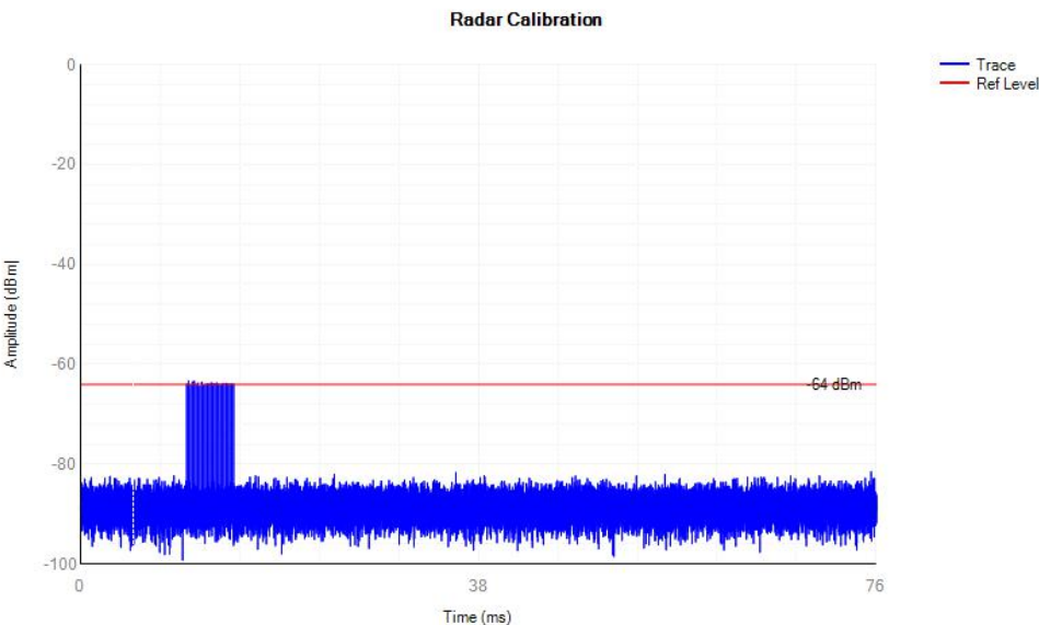
Radar Singal 2
