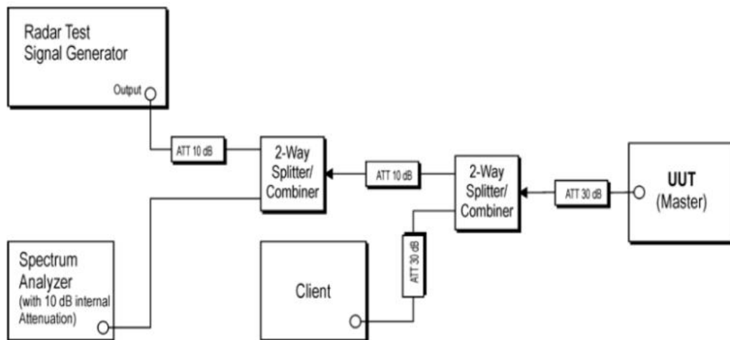
Figure 7-1. Test Setup
