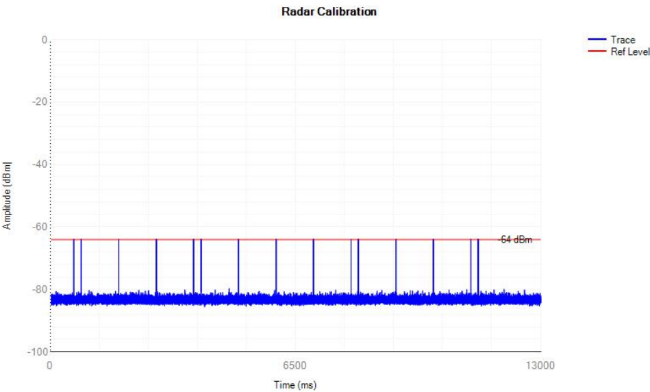
Radar Singal 5
