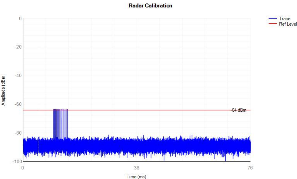
Radar Singal 4
