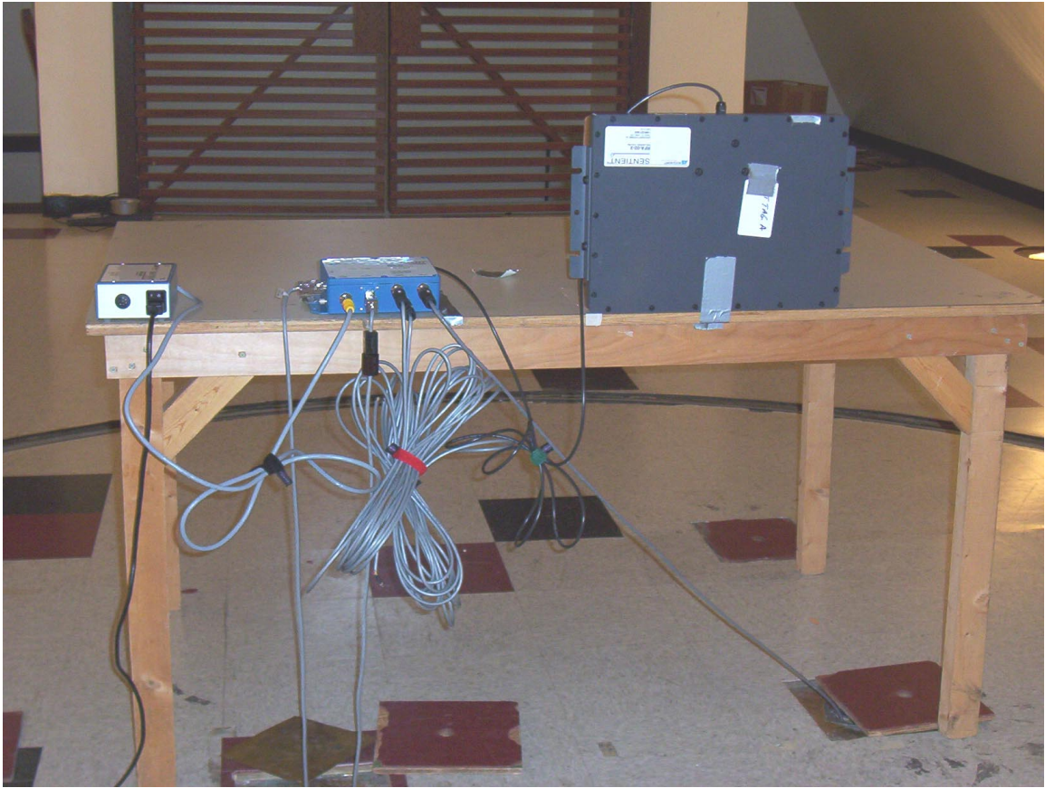
RFR-02/RFA-02-2 Radiated Emission Test Setup
