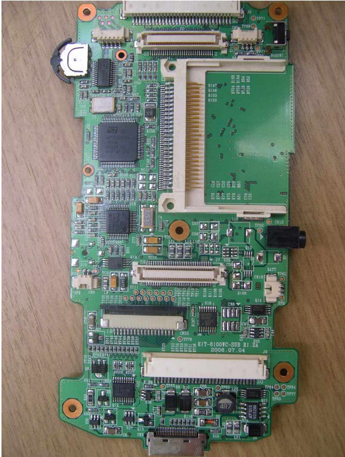
<Photograph 2: Internal Front View - Main>
