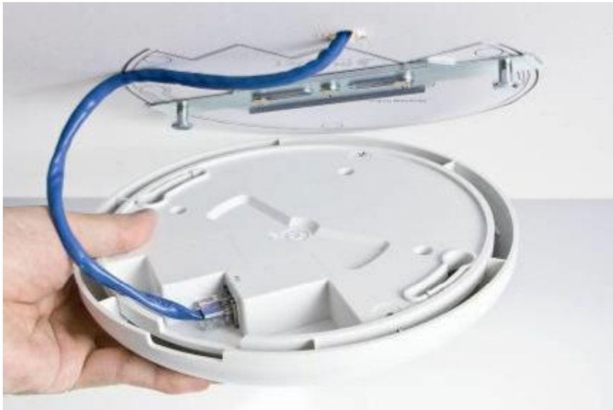
Figure 3-3 WDAP-C7200AC Installation Diagram 3
