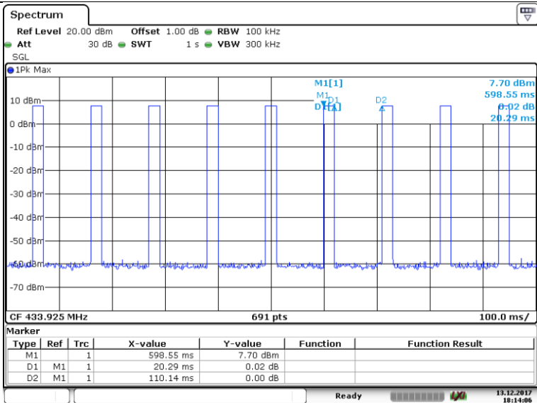
T_{on} + T_{off}
