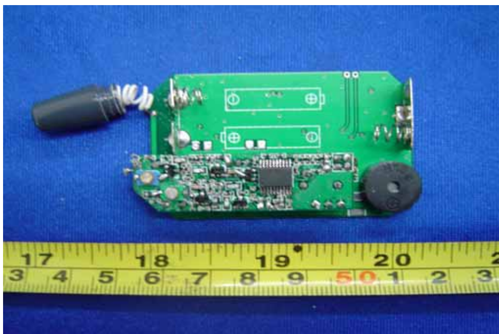
PCB-Solder View
