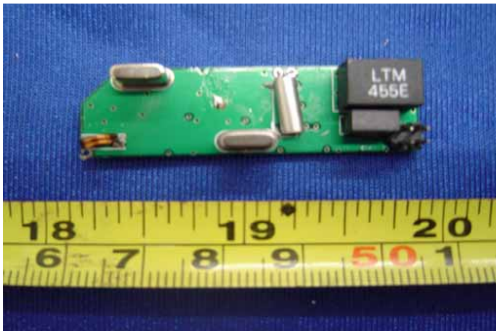
PCB2-Back View
