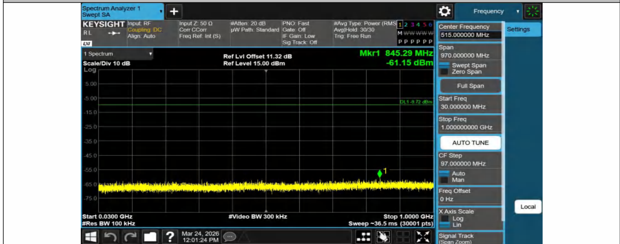
11B-Ant1-2462-30~1000-PASS
