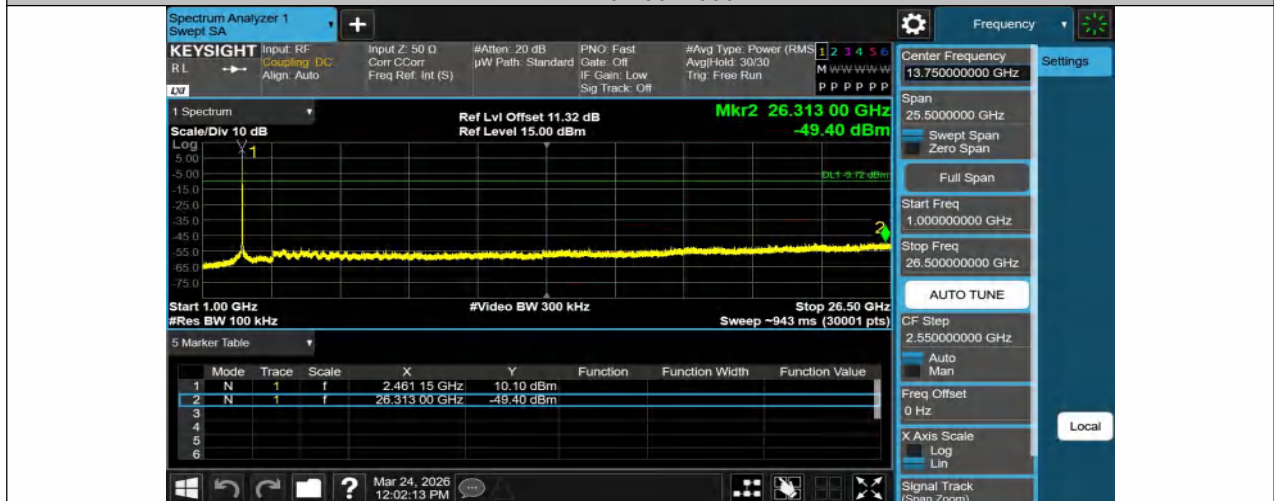
11B-Ant1-2462-1000~26500-PASS
