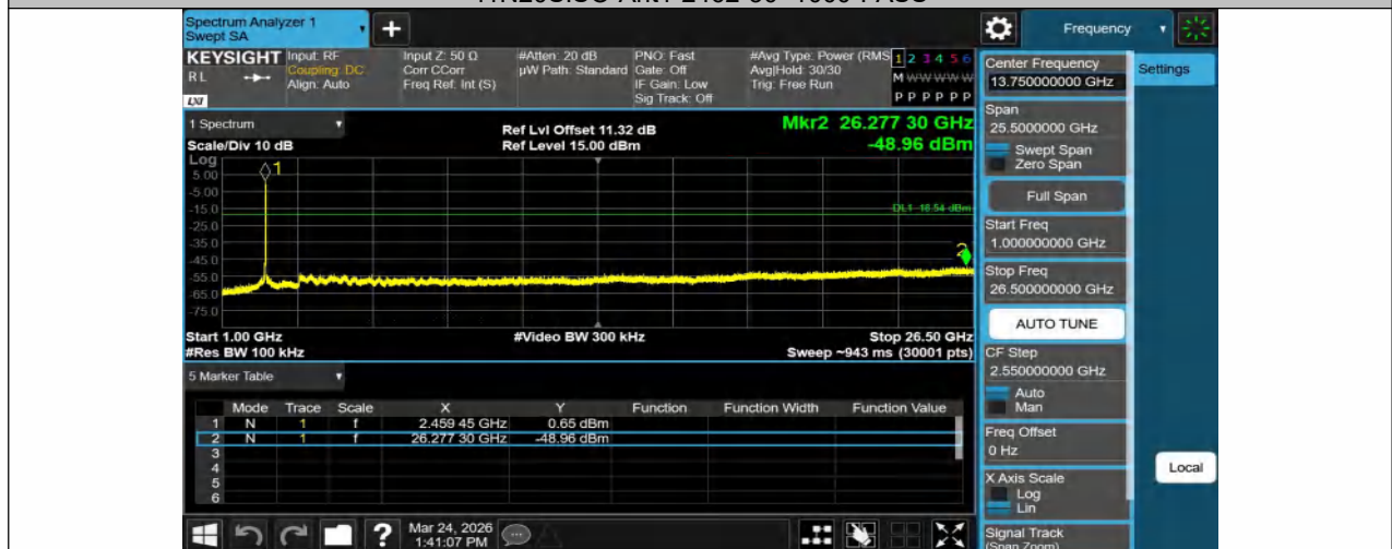
11N20SISO-Ant1-2462-1000~26500-PASS
