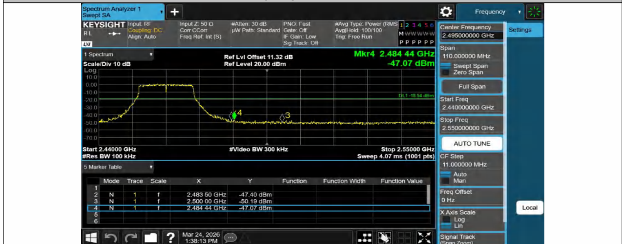
11N20SISO-Ant1-2462-PASS
