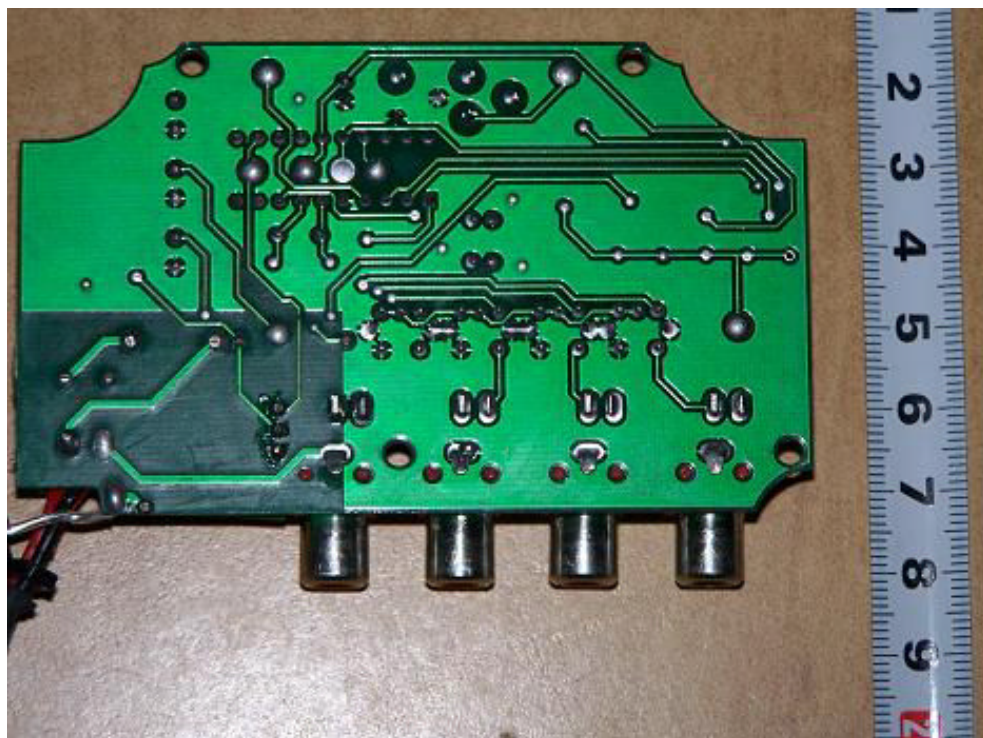
Solder View
