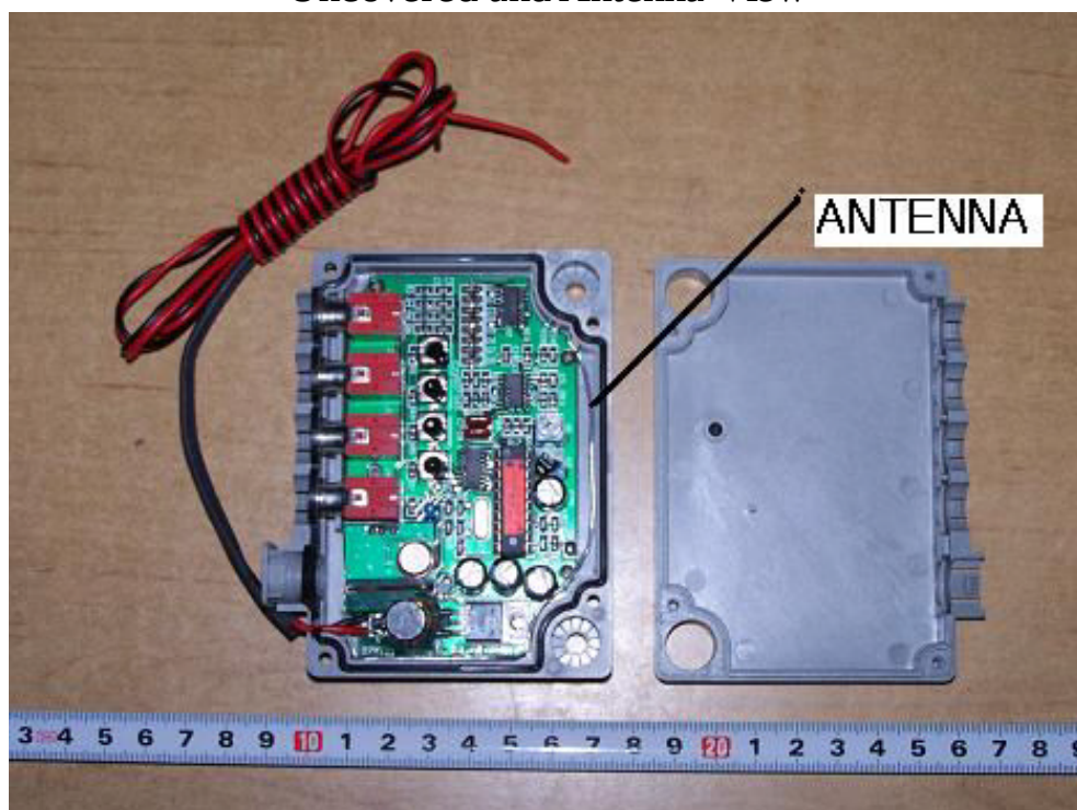
Uncovered and Antenna View
