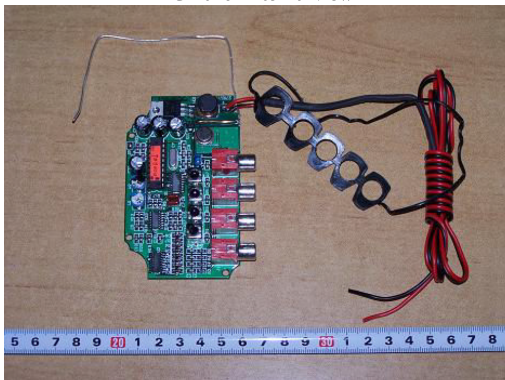
PCB and Antenna View
