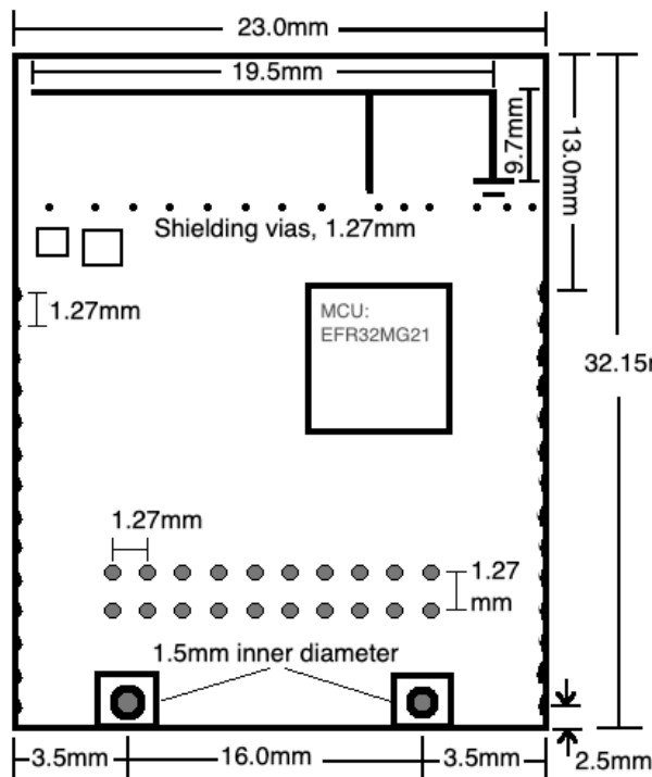
Figure 4: Board Dimensions
