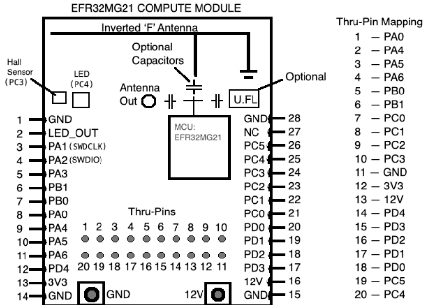
Figure 3: Module connections
