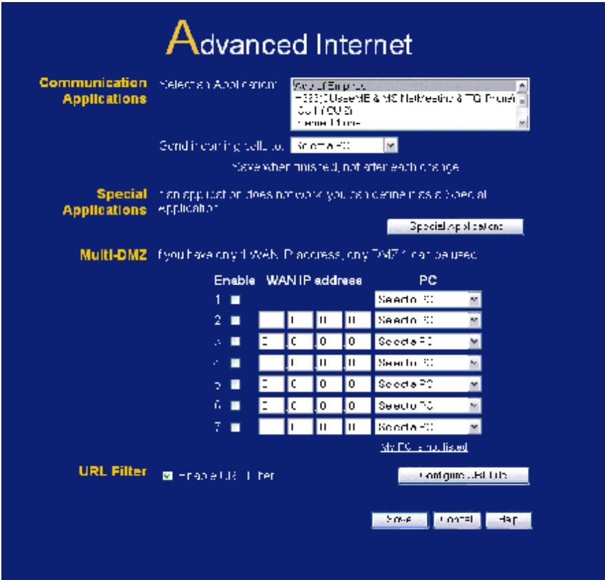
Figure 32: Internet Screen
