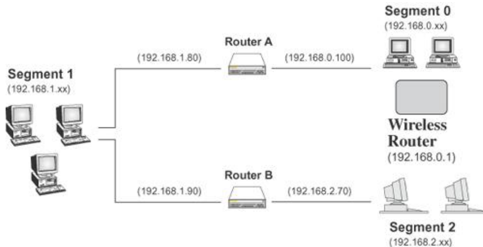
Figure 48: Routing Example
