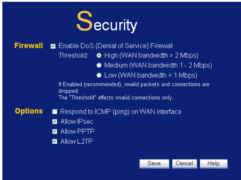
Figure 49: Security Screen
