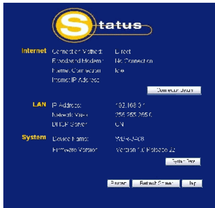
Figure 20: Status Screen
