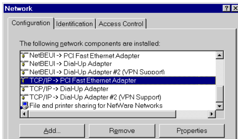
Figure 12: Network Configuration
