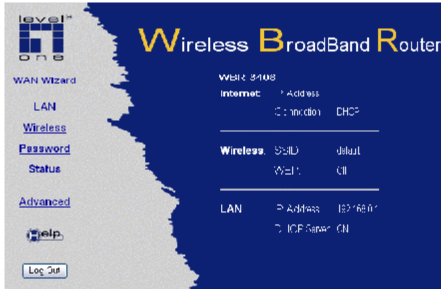
Figure 5: Home Screen
