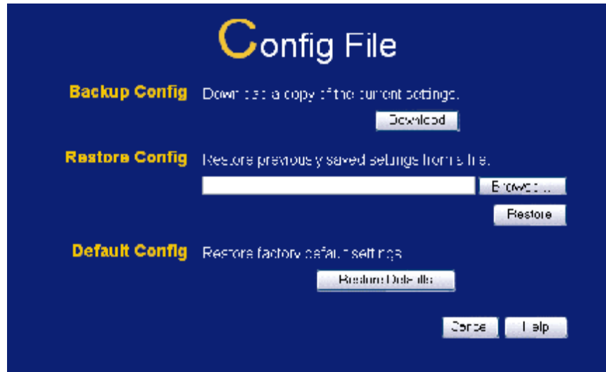
Figure 38: Config Screen
