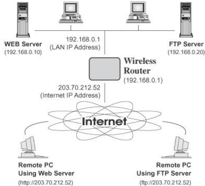
Figure 35: Virtual Servers
