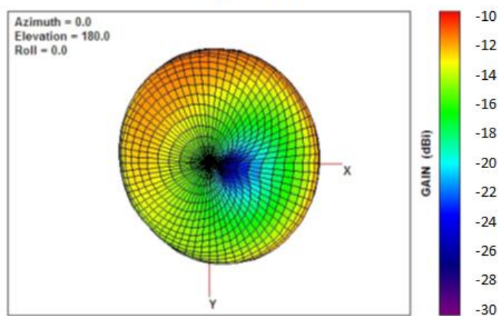
Total, Bottom View
